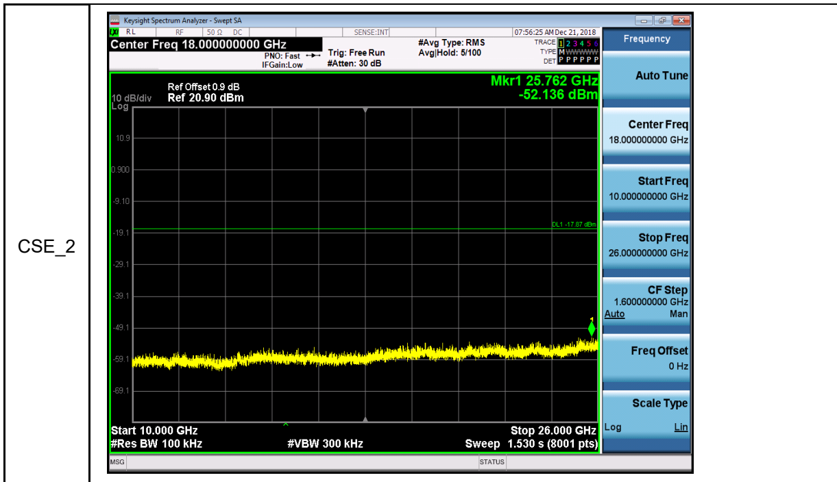
RF Conducted Spurious Emissions_3DH5_2402
