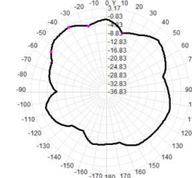
Total(H-XY), Max= -1.30dBi, CirD=13.97
