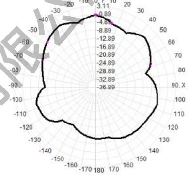
Total(H-XY), Max= -1.36dBi, CirD=14.05
