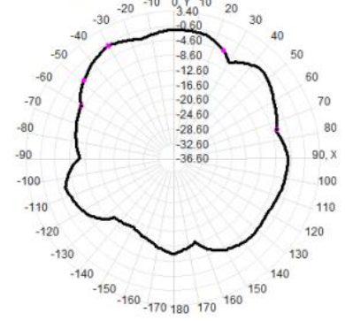
Total(H-XY), Max= -1.34dBi, CirD=13.90
