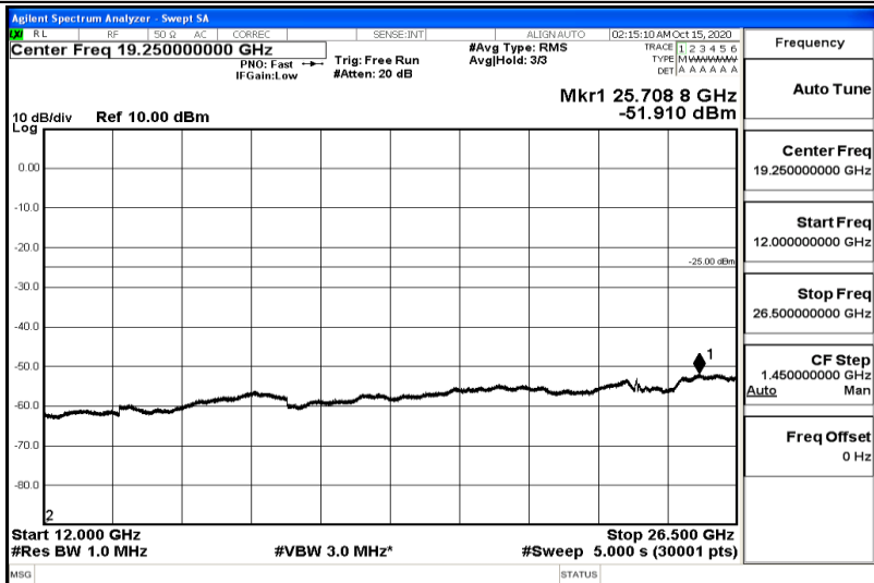
Band41-20MHz-16QAM-41490-1RB#0-Range6:12000~26500MHz
