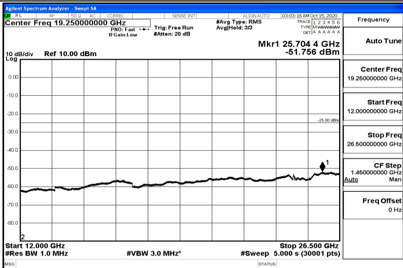
Band41-10MHz-QPSK-40620-1RB#0-Range1:0.009~0.15MHz
