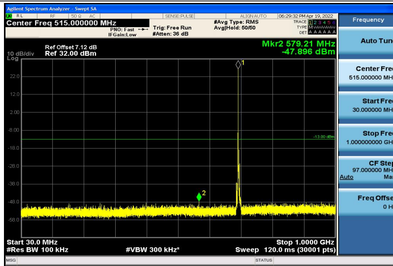
Band12-3MHz-16QAM-23025-1RB#0-30~1000MHz
