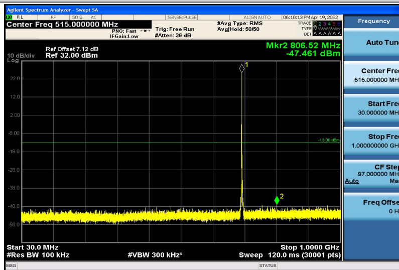
Band12-1.4MHz-16QAM-23017-1RB#0-30~1000MHz
