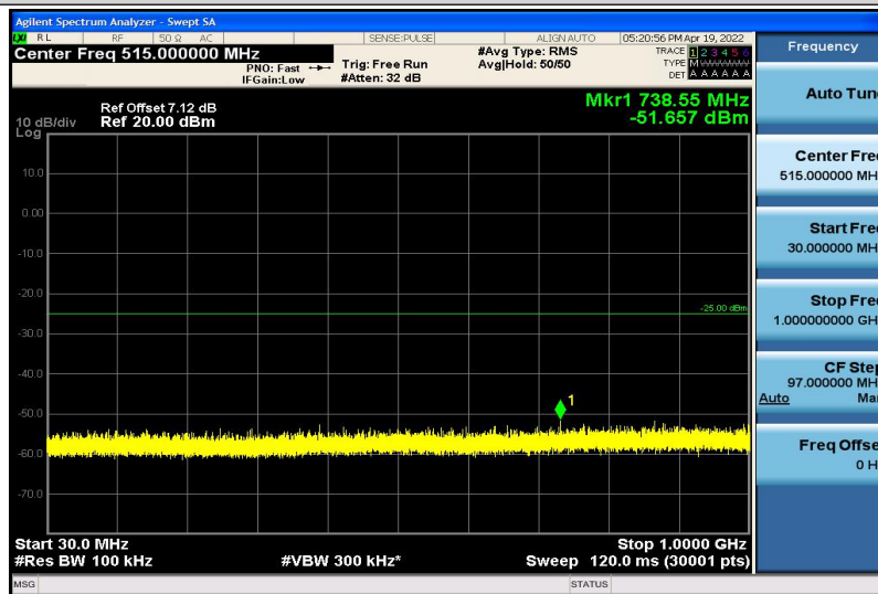
Band7-15MHz-16QAM-20825-1RB#0-30~1000MHz
