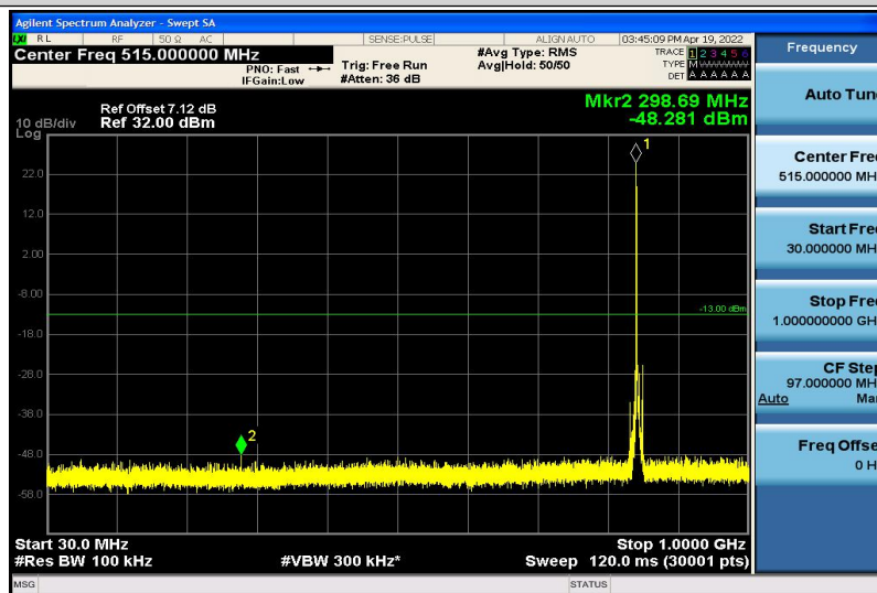
Band5-5MHz-16QAM-20625-1RB#0-30~1000MHz
