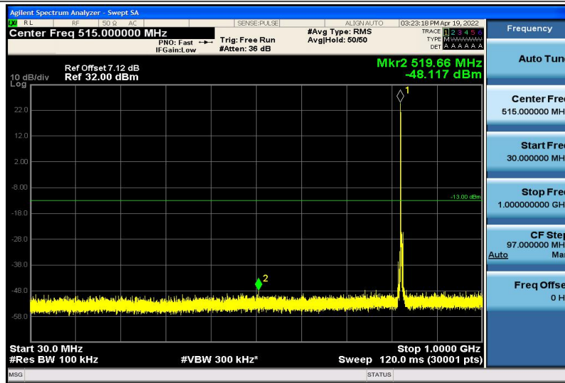
Band5-3MHz-16QAM-20415-1RB#0-30~1000MHz
