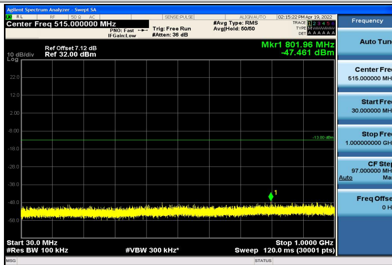
Band4-15MHz-QPSK-20025-1RB#0-30~1000MHz
