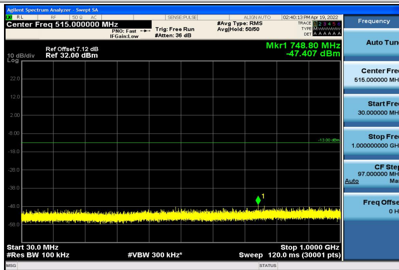
Band4-20MHz-16QAM-20050-1RB#0-30~1000MHz
