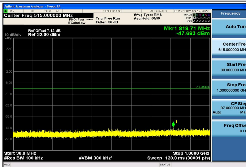
Band4-3MHz-16QAM-20385-1RB#0-30~1000MHz
