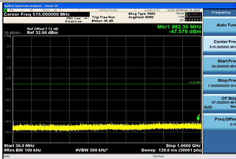
Band4-1.4MHz-16QAM-19957-1RB#0-30~1000MHz
