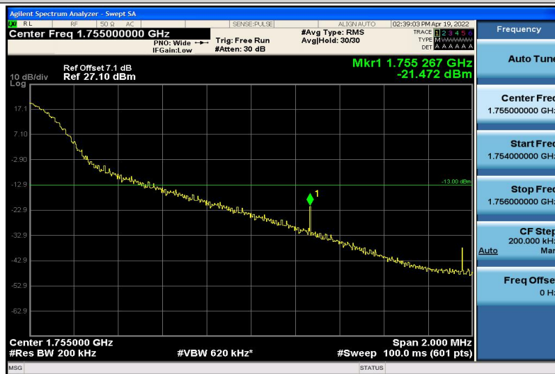
Band4-20MHz-16QAM-20300-1RB#99
