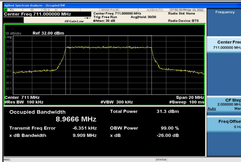
Band17-10MHz-16QAM-23800-50RB#0-8.9666
