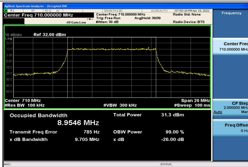
Band17-10MHz-16QAM-23790-50RB#0-8.9546
