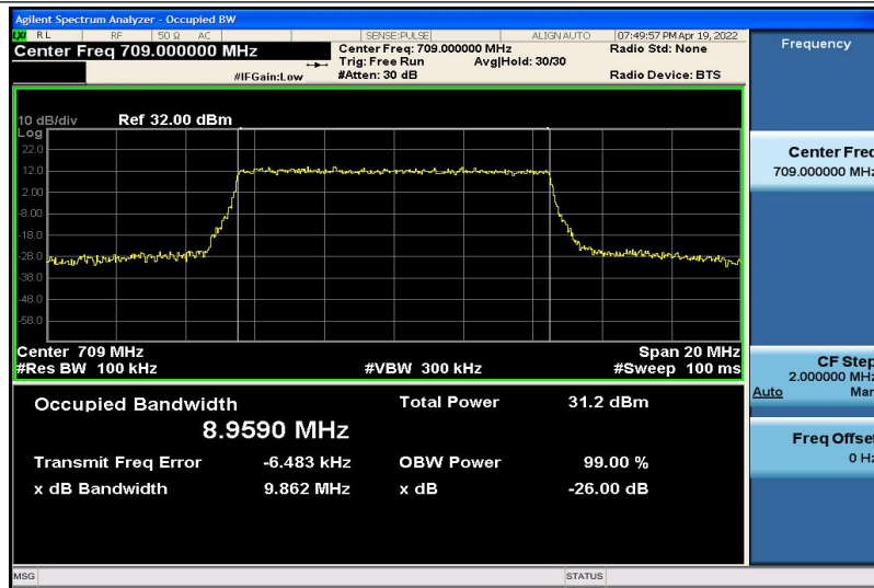
Band17-10MHz-16QAM-23780-50RB#0-8.9590
