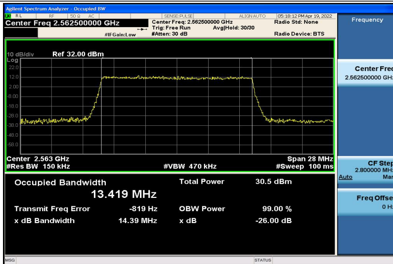
Band7-15MHz-QPSK-21375-75RB#0-13.419
