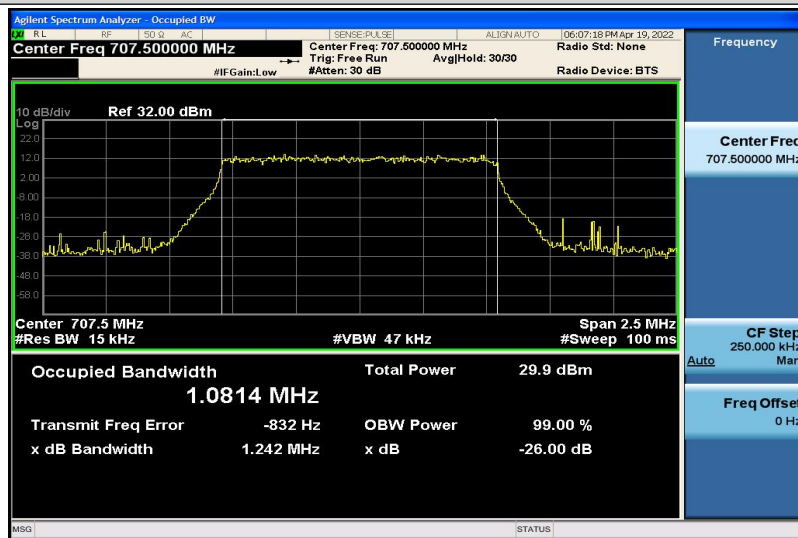
Band12-1.4MHz-QPSK-23095-6RB#0-1.0814
