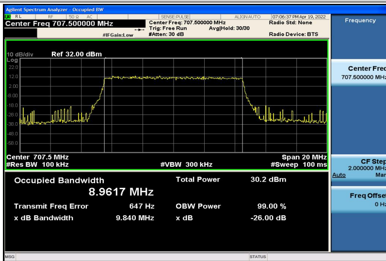
Band12-10MHz-16QAM-23095-50RB#0-8.9617
