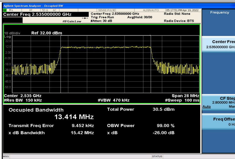
Band7-15MHz-QPSK-21100-75RB#0-13.414
