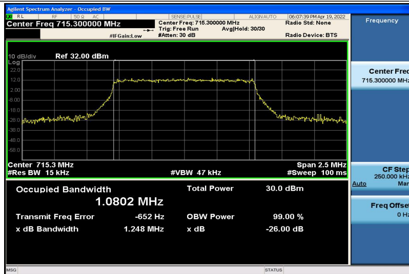
Band12-1.4MHz-QPSK-23173-6RB#0-1.0802
