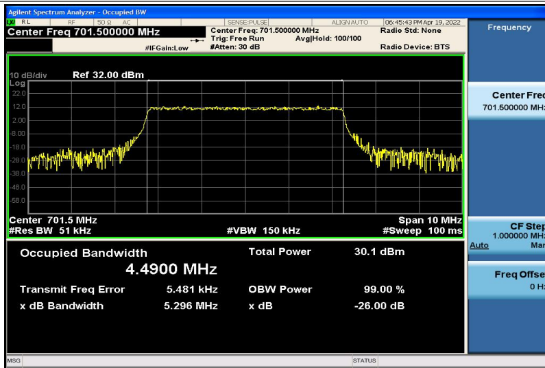
Band12-5MHz-16QAM-23035-25RB#0-4.4900
