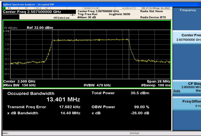
Band7-15MHz-QPSK-20825-75RB#0-13.401
