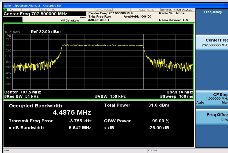
Band12-5MHz-QPSK-23095-25RB#0-4.4875
