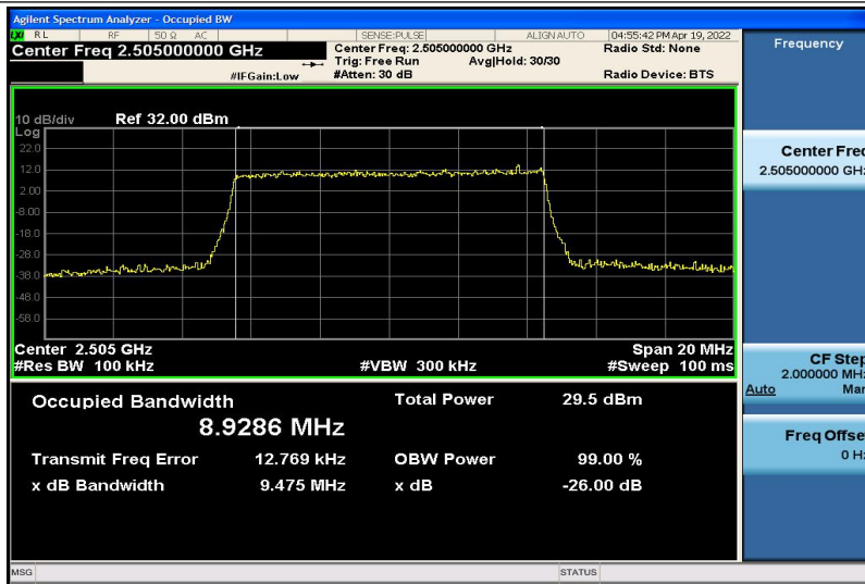
Band7-10MHz-16QAM-20800-50RB#0-8.9286
