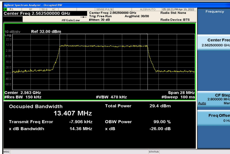
Band7-15MHz-16QAM-21375-75RB#0-13.407
