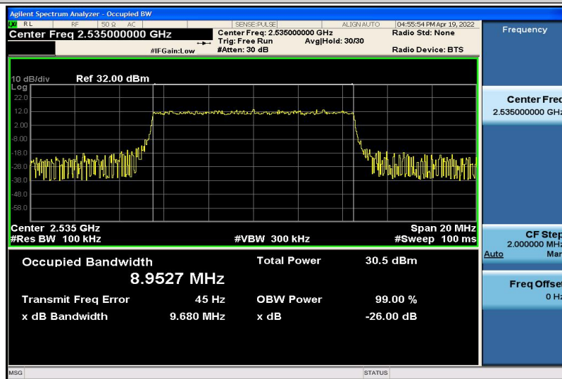
Band7-10MHz-QPSK-21100-50RB#0-8.9527
