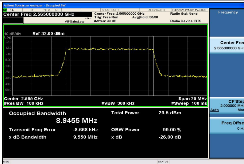
Band7-10MHz-16QAM-21400-50RB#0-8.9455
