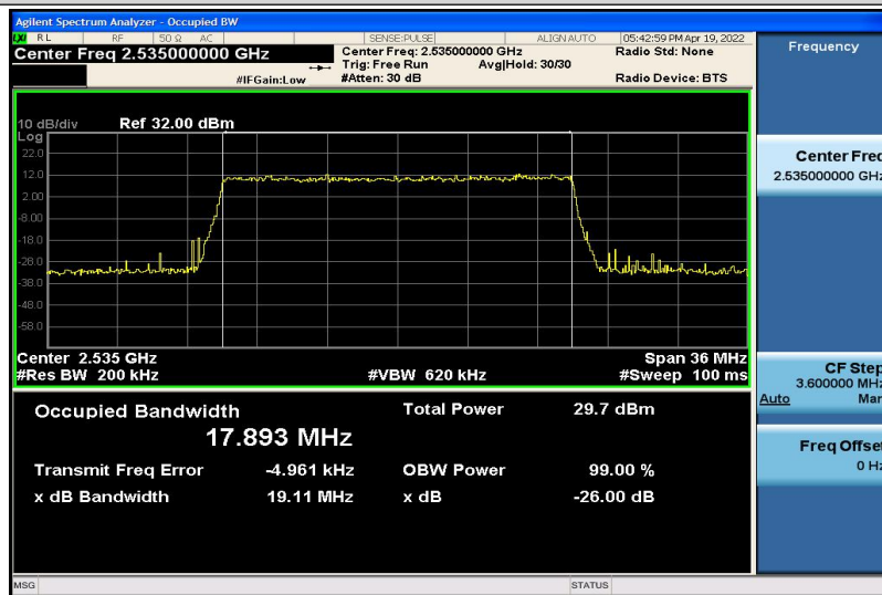
Band7-20MHz-QPSK-21100-100RB#0-17.893
