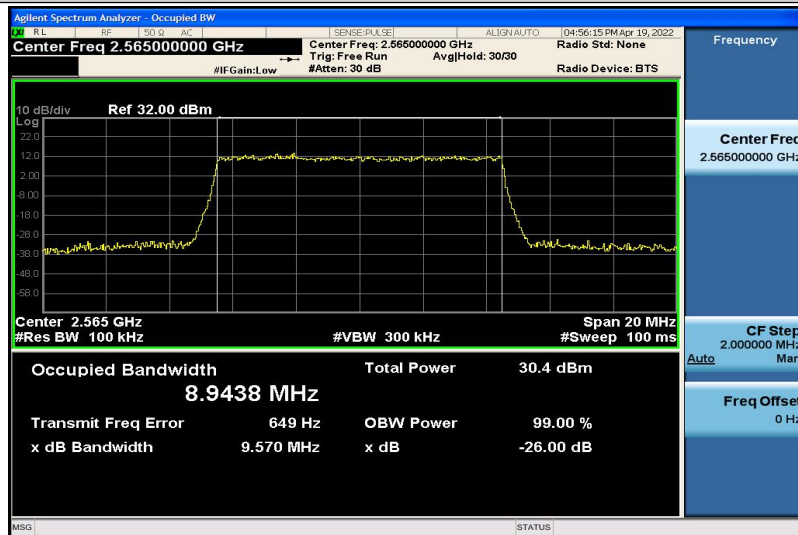
Band7-10MHz-QPSK-21400-50RB#0-8.9438
