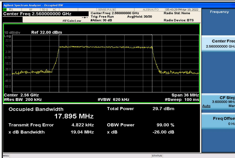
Band7-20MHz-16QAM-21350-100RB#0-17.895
