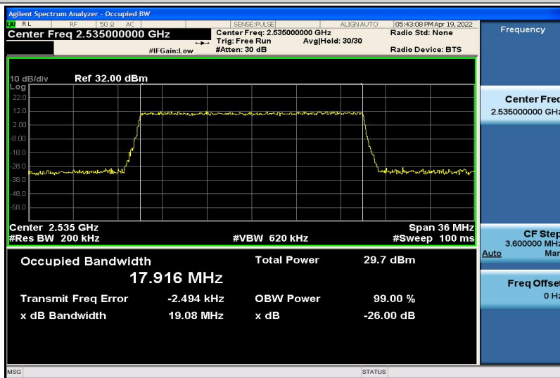
Band7-20MHz-16QAM-21100-100RB#0-17.916
