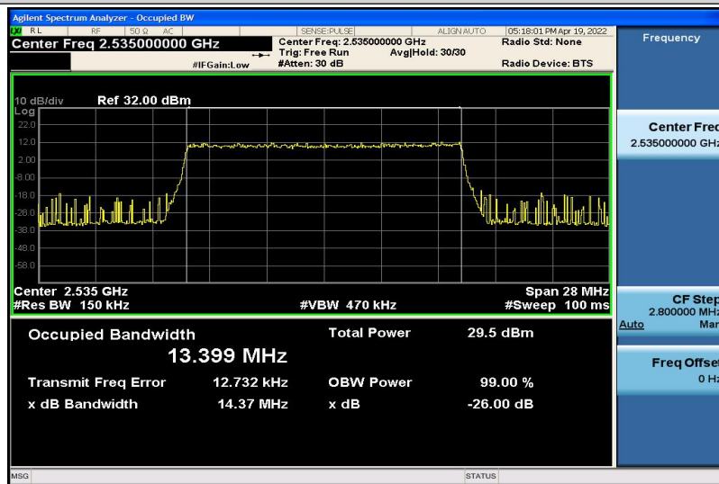
Band7-15MHz-16QAM-21100-75RB#0-13.399
