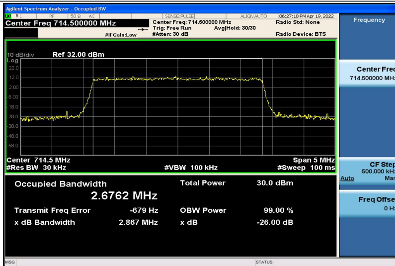
Band12-3MHz-16QAM-23165-15RB#0-2.6762
