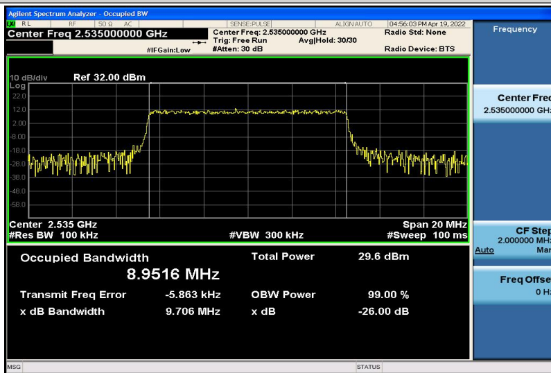
Band7-10MHz-16QAM-21100-50RB#0-8.9516
