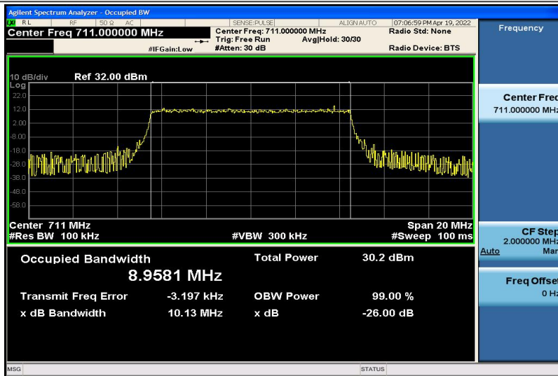
Band12-10MHz-16QAM-23130-50RB#0-8.9581
