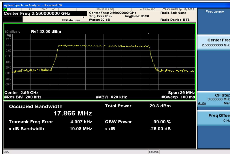
Band7-20MHz-QPSK-21350-100RB#0-17.866
