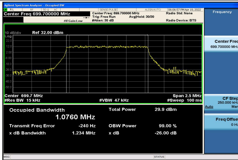
Band12-1.4MHz-QPSK-23017-6RB#0-1.0760
