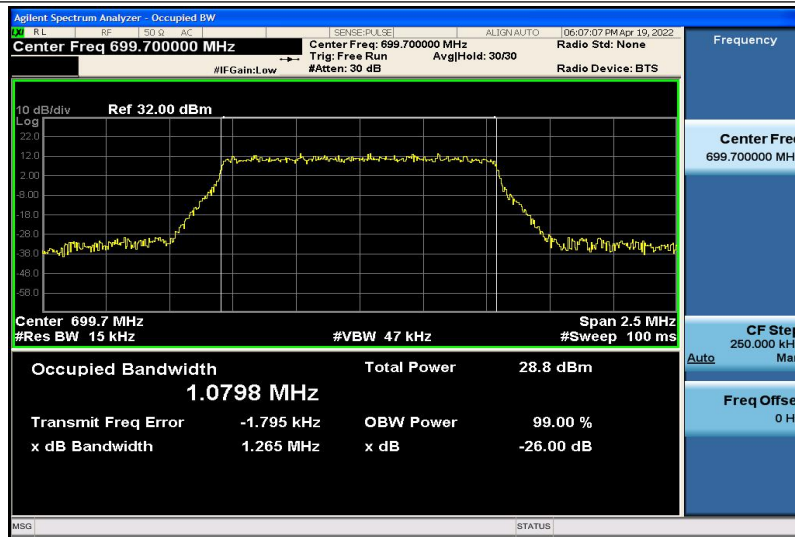
Band12-1.4MHz-16QAM-23017-6RB#0-1.0798
