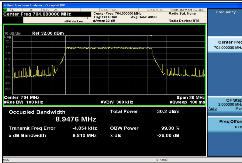
Band12-10MHz-16QAM-23060-50RB#0-8.9476
