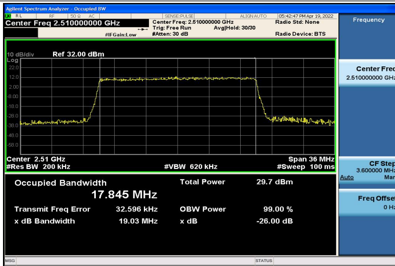
Band7-20MHz-16QAM-20850-100RB#0-17.845
