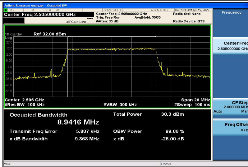
Band7-10MHz-QPSK-20800-50RB#0-8.9416
