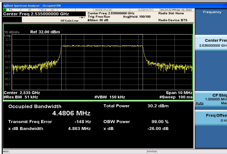
Band7-5MHz-QPSK-21100-25RB#0-4.4806
