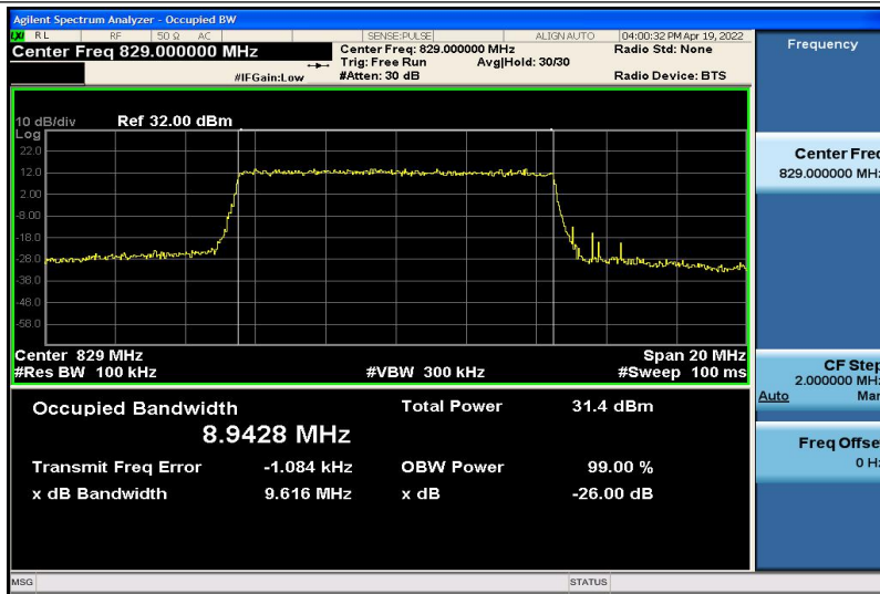
Band5-10MHz-QPSK-20450-50RB#0-8.9428
