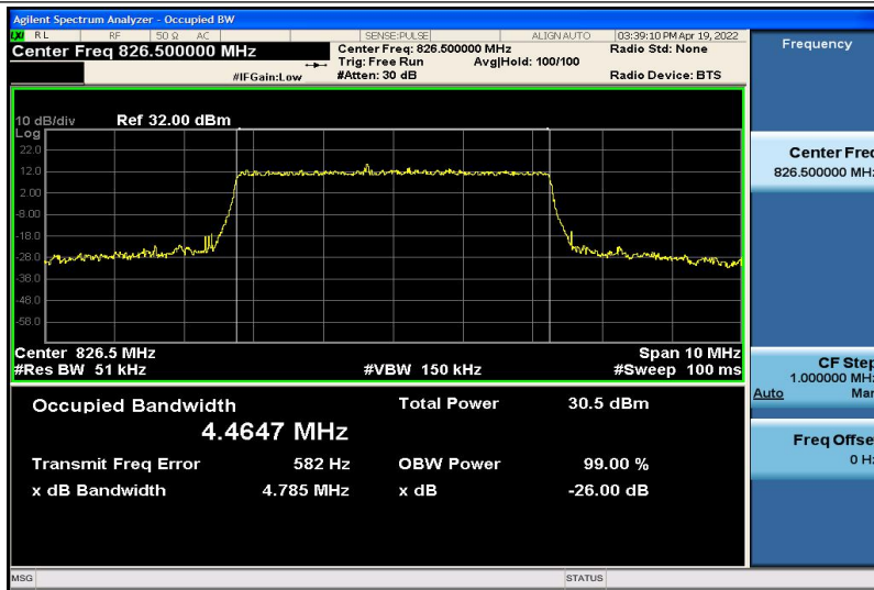
Band5-5MHz-16QAM-20425-25RB#0-4.4647
