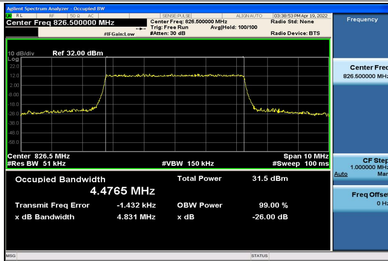
Band5-5MHz-QPSK-20425-25RB#0-4.4765
