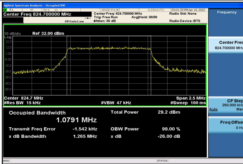
Band5-1.4MHz-16QAM-20407-6RB#0-1.0791
