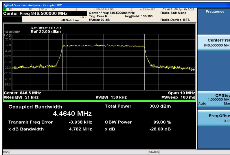
Band5-5MHz-16QAM-20625-25RB#0-4.4640
