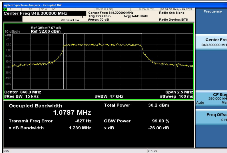
Band5-1.4MHz-QPSK-20643-6RB#0-1.0787
