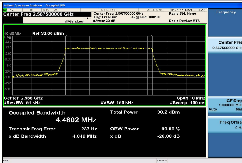
Band7-5MHz-QPSK-21425-25RB#0-4.4802
