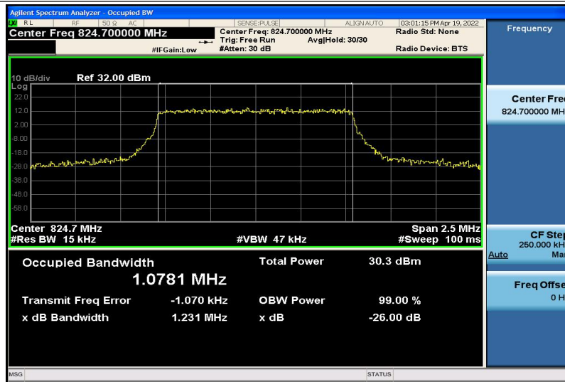
Band5-1.4MHz-QPSK-20407-6RB#0-1.0781
