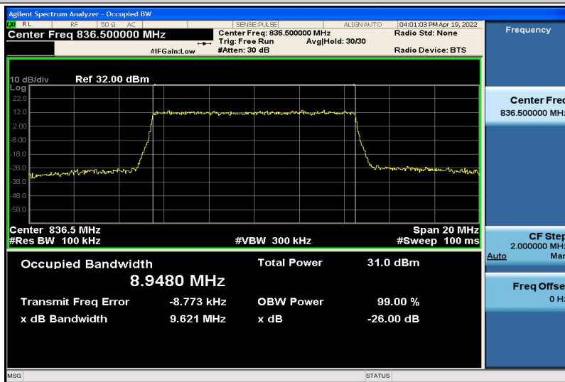
Band5-10MHz-16QAM-20525-50RB#0-8.9480
