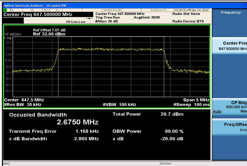
Band5-3MHz-16QAM-20635-15RB#0-2.6750
