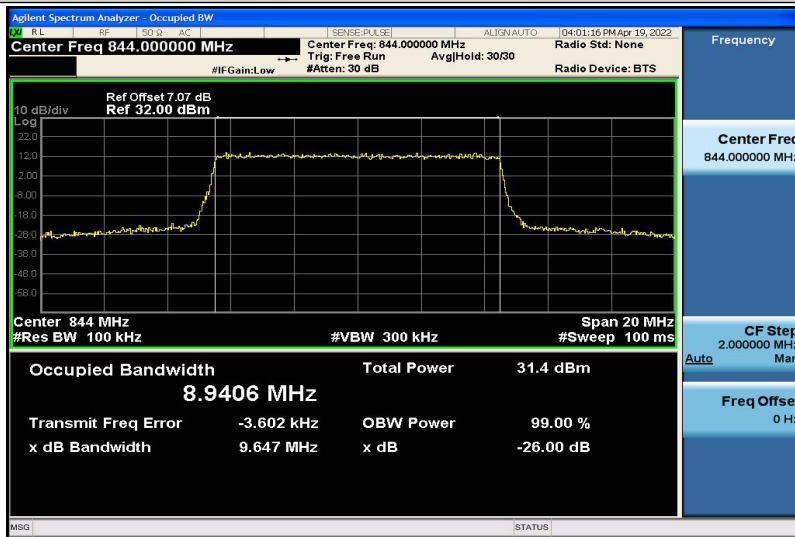
Band5-10MHz-QPSK-20600-50RB#0-8.9406
