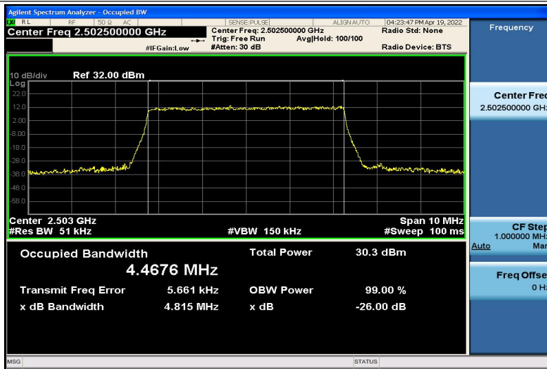
Band7-5MHz-QPSK-20775-25RB#0-4.4676
