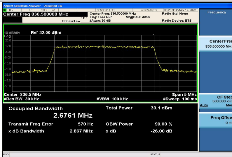
Band5-3MHz-16QAM-20525-15RB#0-2.6761
