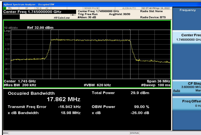
Band4-20MHz-16QAM-20300-100RB#0-17.862
