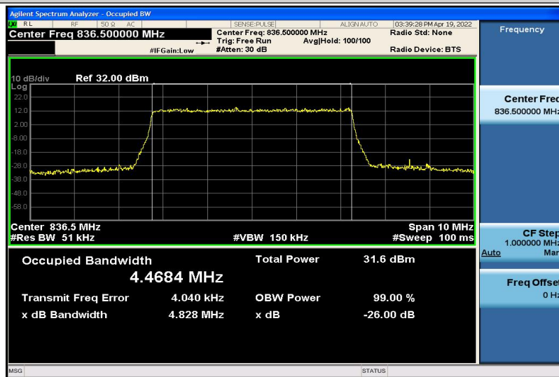
Band5-5MHz-QPSK-20525-25RB#0-4.4684
