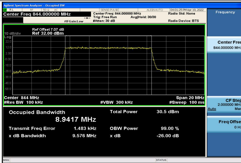
Band5-10MHz-16QAM-20600-50RB#0-8.9417
