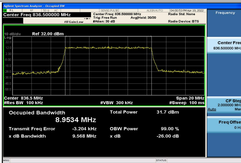
Band5-10MHz-QPSK-20525-50RB#0-8.9534
