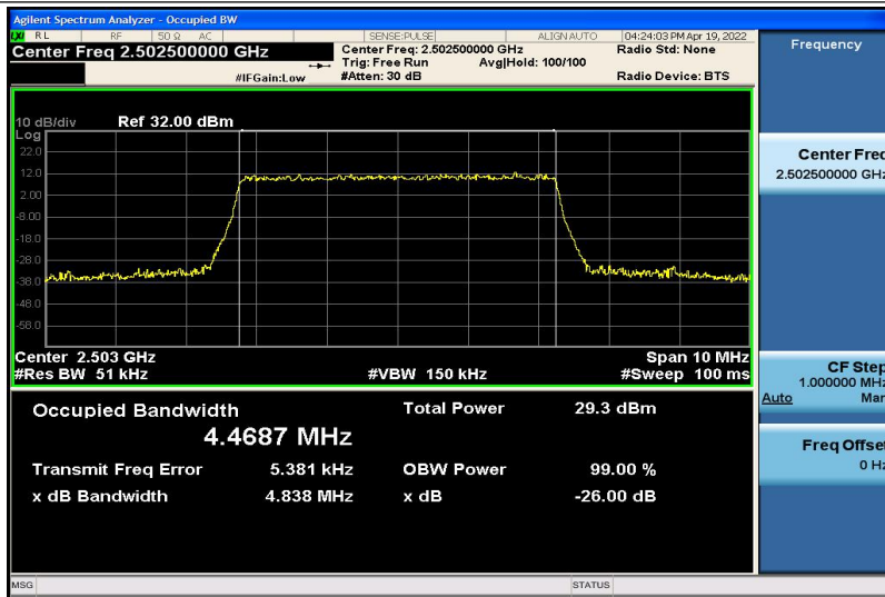
Band7-5MHz-16QAM-20775-25RB#0-4.4687
