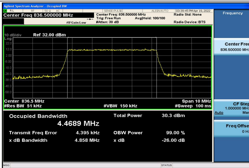
Band5-5MHz-16QAM-20525-25RB#0-4.4689
