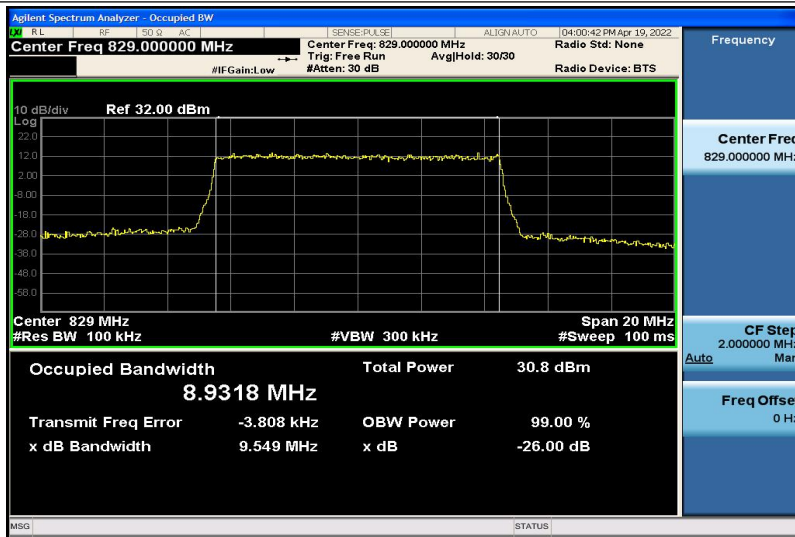
Band5-10MHz-16QAM-20450-50RB#0-8.9318
