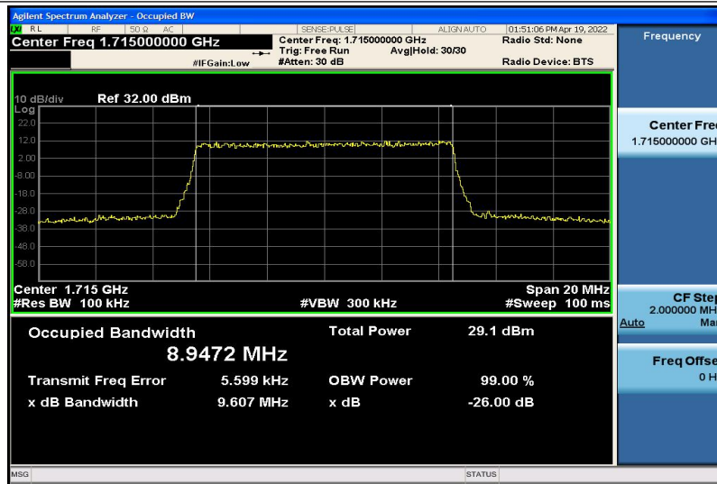
Band4-10MHz-16QAM-20000-50RB#0-8.9472
