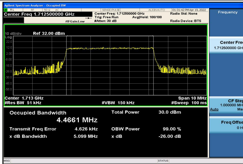
Band4-5MHz-QPSK-19975-25RB#0-4.4661
