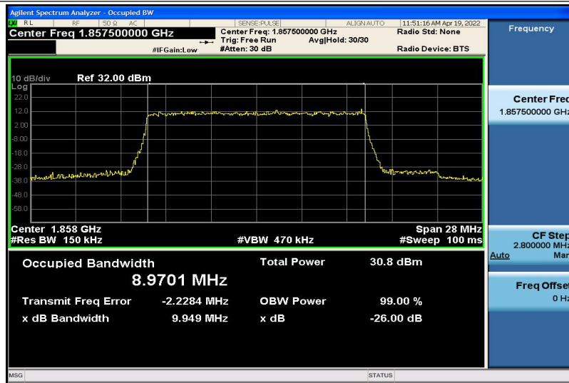
Band2-15MHz-QPSK-18675-75RB#0-8.9701
