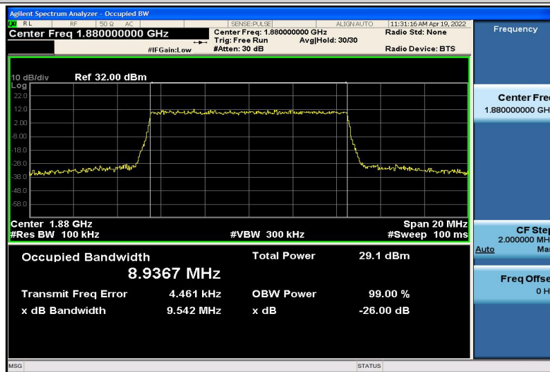
Band2-10MHz-16QAM-18900-50RB#0-8.9367
