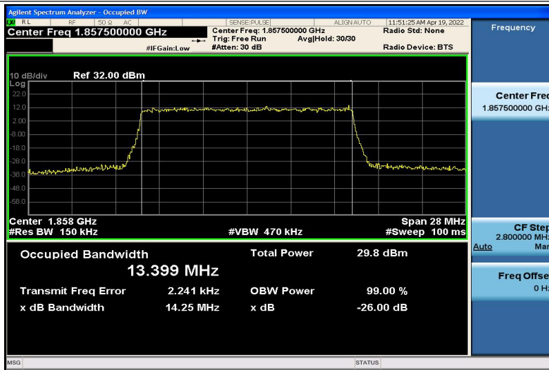
Band2-15MHz-16QAM-18675-75RB#0-13.399
