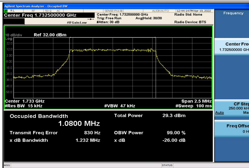
Band4-1.4MHz-QPSK-20175-6RB#0-1.0800
