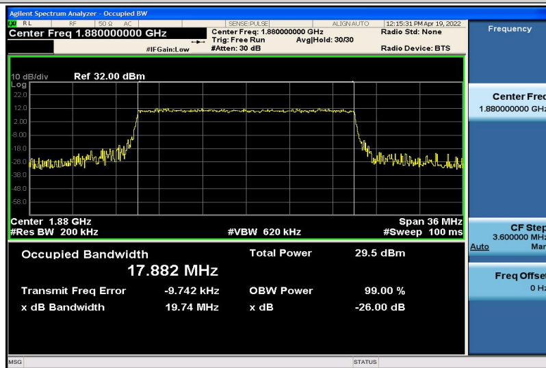
Band2-20MHz-16QAM-18900-100RB#0-17.882
