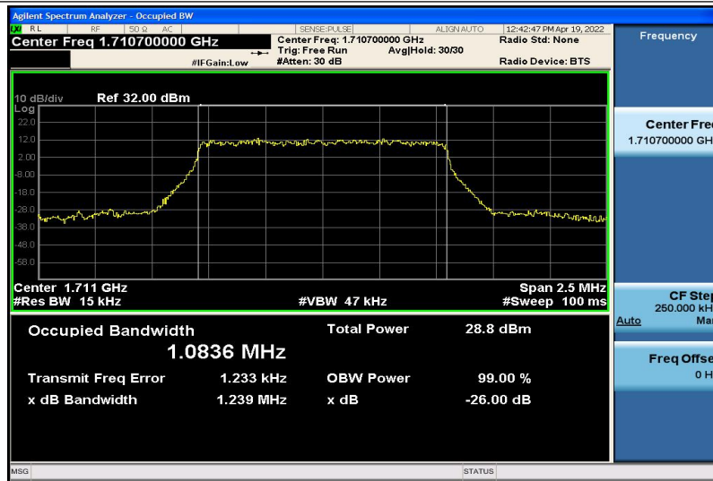
Band4-1.4MHz-QPSK-19957-6RB#0-1.0836
