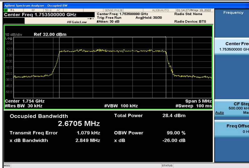
Band4-3MHz-16QAM-20385-15RB#0-2.6705
