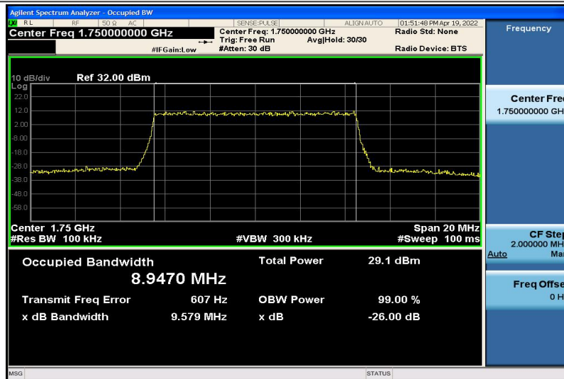
Band4-10MHz-16QAM-20350-50RB#0-8.9470
