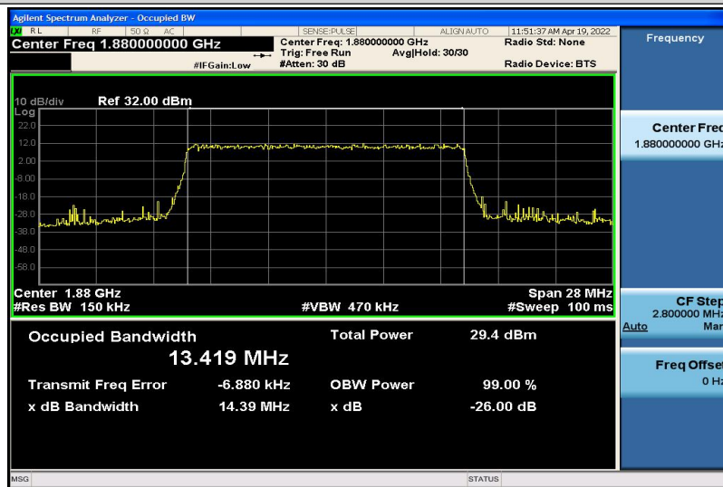
Band2-15MHz-QPSK-18900-75RB#0-13.419
