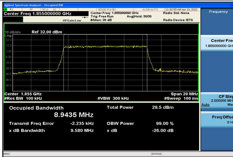
Band2-10MHz-16QAM-18650-50RB#0-8.9435
