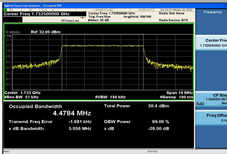
Band4-5MHz-QPSK-17325-25RB#0-4.4784
