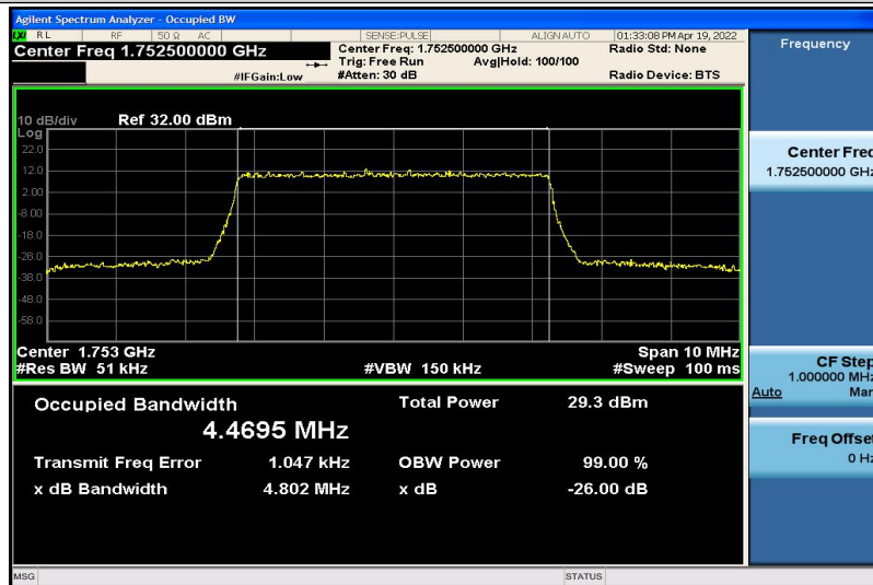
Band4-5MHz-16QAM-20375-25RB#0-4.4695
