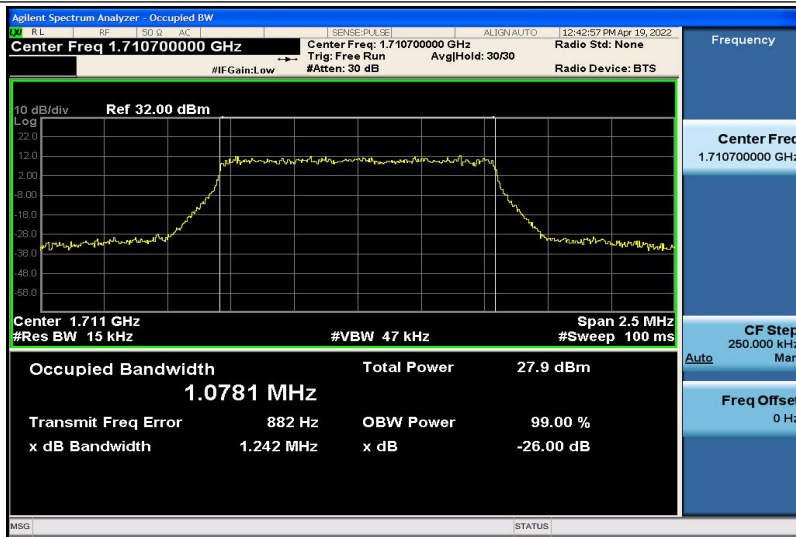
Band4-1.4MHz-16QAM-19957-6RB#0-1.0781
