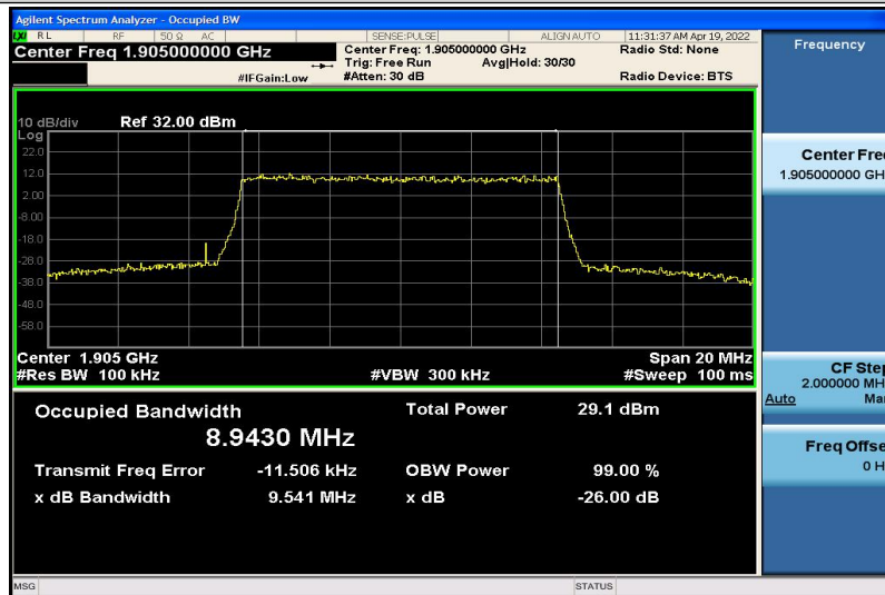
Band2-10MHz-16QAM-19150-50RB#0-8.9430
