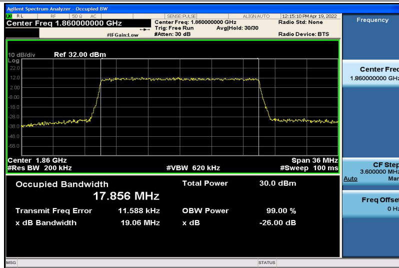
Band2-20MHz-16QAM-18700-100RB#0-17.856
