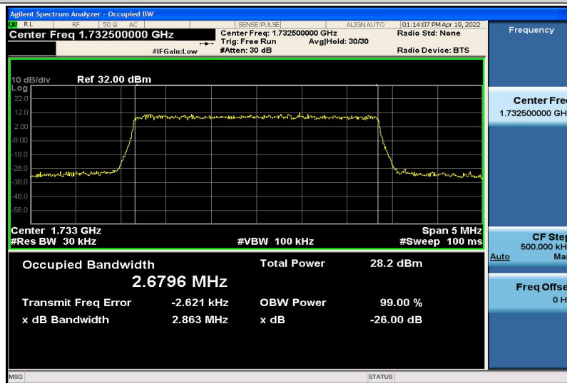
Band4-3MHz-16QAM-20175-15RB#0-2.6796
