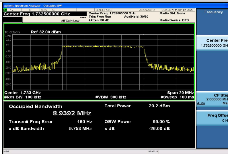
Band4-10MHz-16QAM-20175-50RB#0-8.9392
