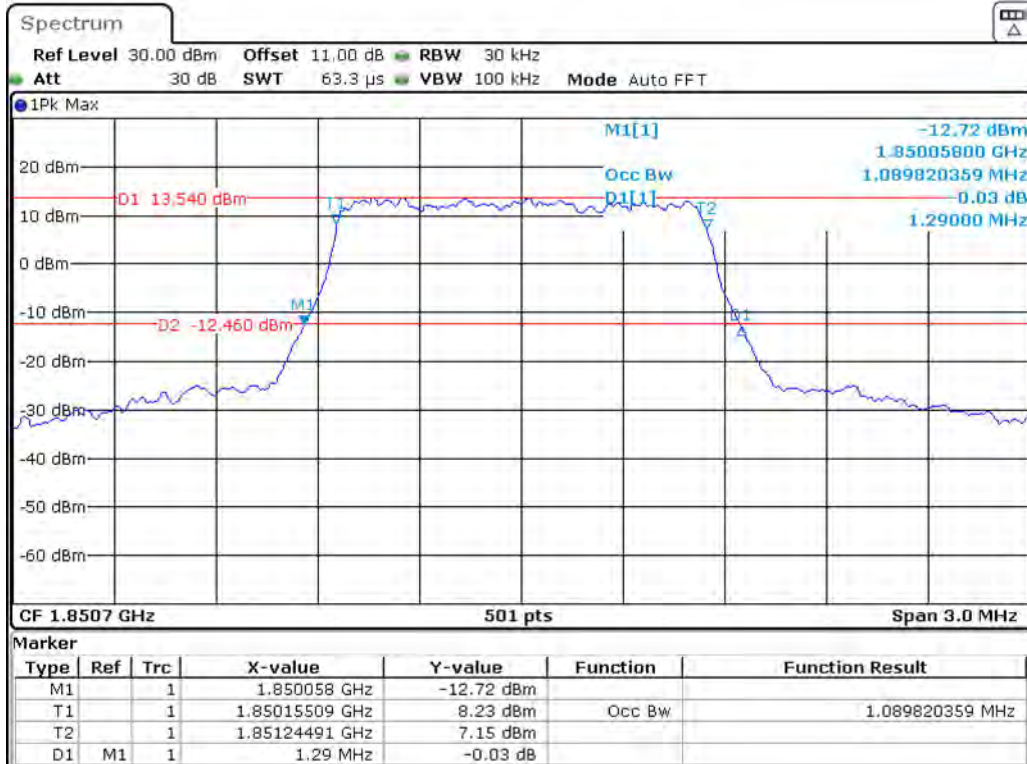
Band 2_1.4 MHz_Low_16QAM_RB6#0
