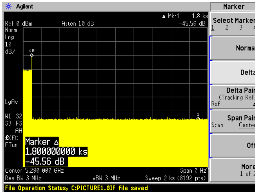
5290 MHz
