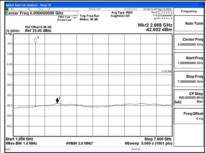
1 GHz – 7 GHz
