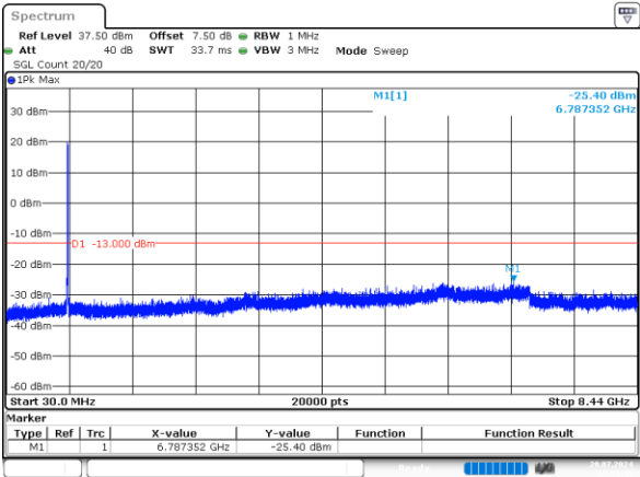
10MHz_High_QPSK_50@0 -25.40dBm
