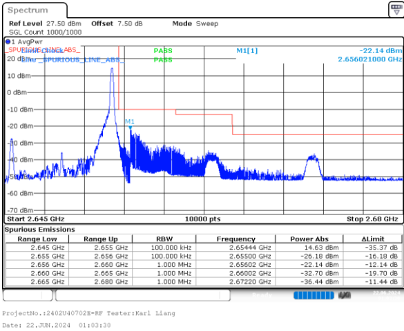
3_15MHz_Low_QPSK_1@0
