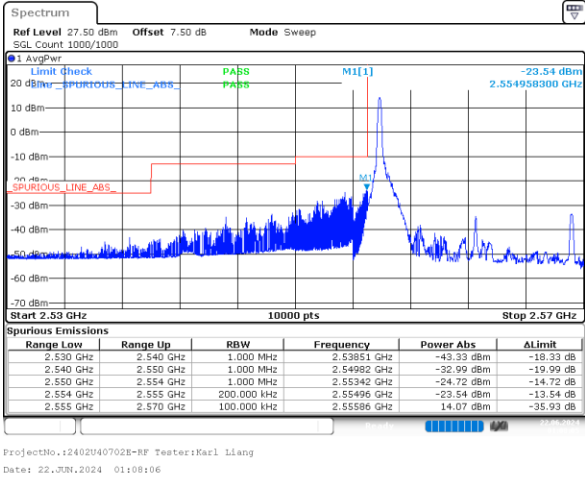
3_15MHz_Low_16QAM_1@0
