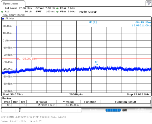
5MHz_Low_QPSK_25@0 -34.45dBm
