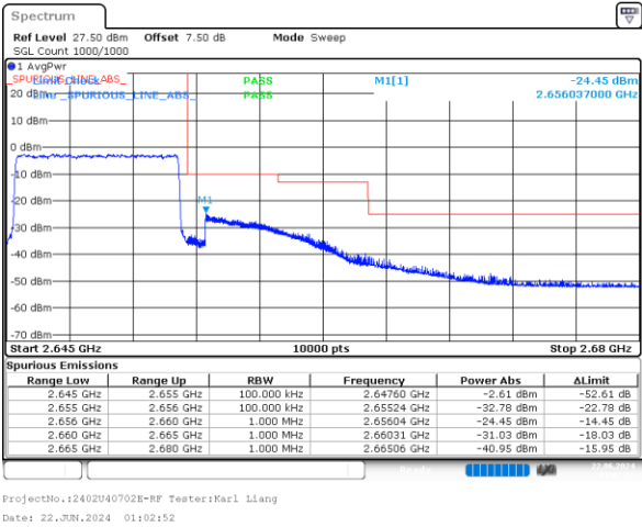
3_15MHz_Low_QPSK_75@0
