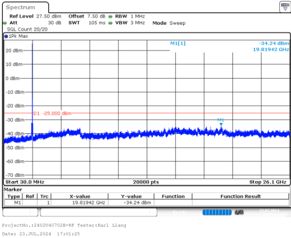
20MHz_High_QPSK_1@0 -34.24dBm
