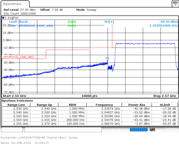
3_15MHz_Low_16QAM_75@0
