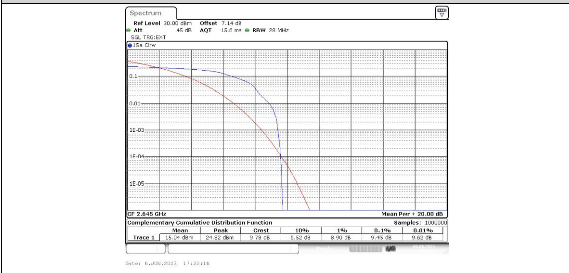
Band41-20MHz-16QAM-41140-100RB#0
