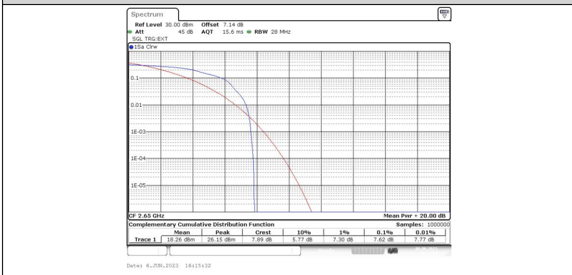
Band41-10MHz-16QAM-41190-50RB#0
