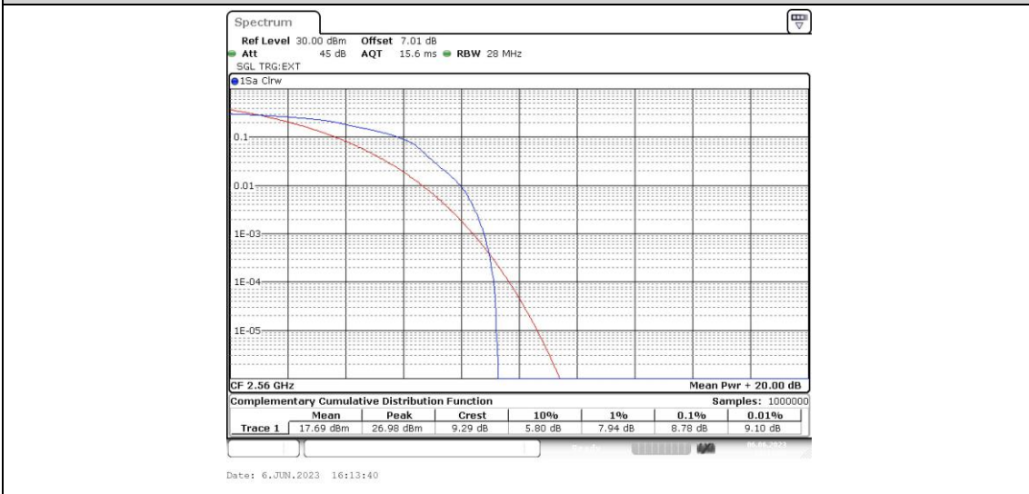
Band41-10MHz-16QAM-40290-50RB#0
