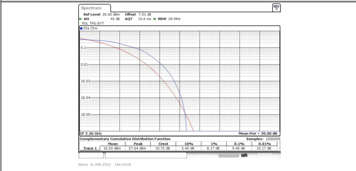
Band41-10MHz-16QAM-40740-1RB#0
