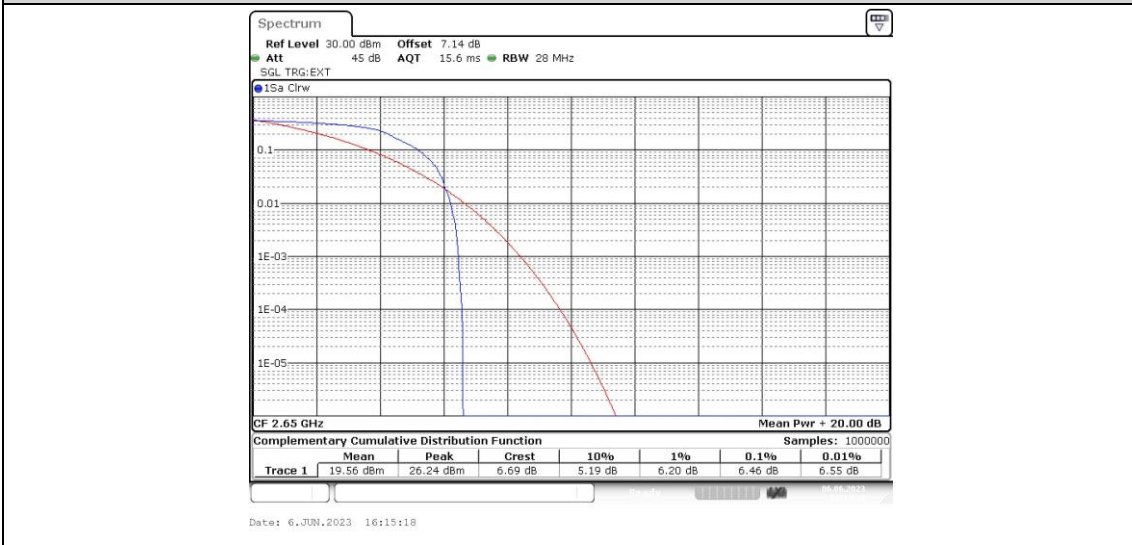
Band41-10MHz-QPSK-41190-50RB#0
