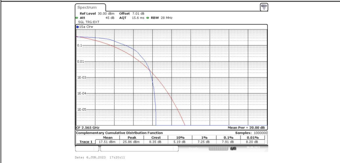
Band41-20MHz-QPSK-40340-100RB#0
