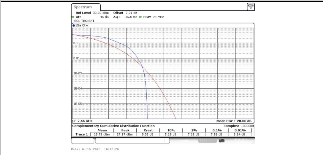
Band41-10MHz-QPSK-40290-50RB#0
