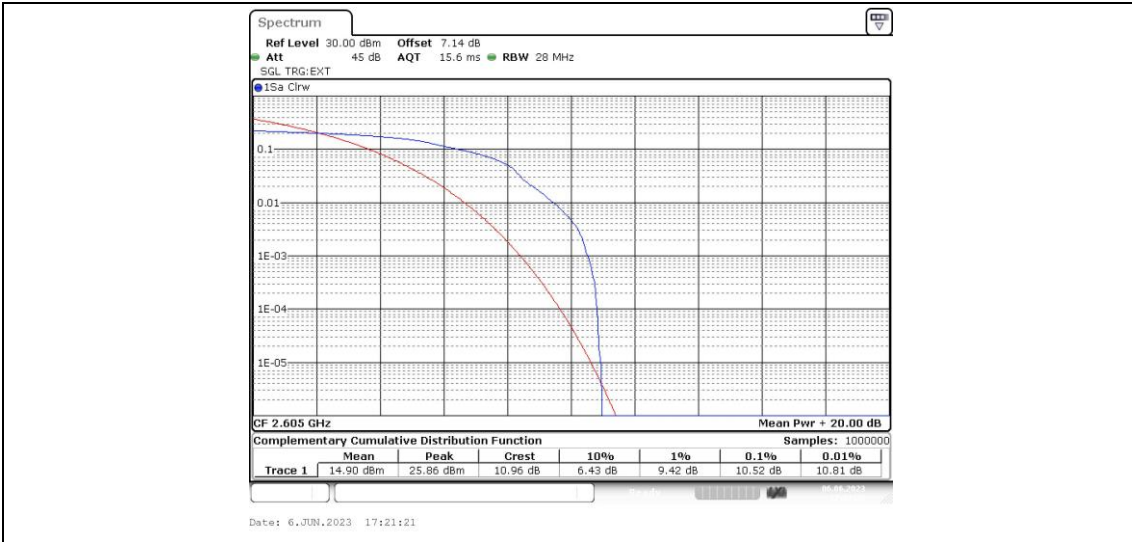
Band41-20MHz-16QAM-40740-100RB#0
