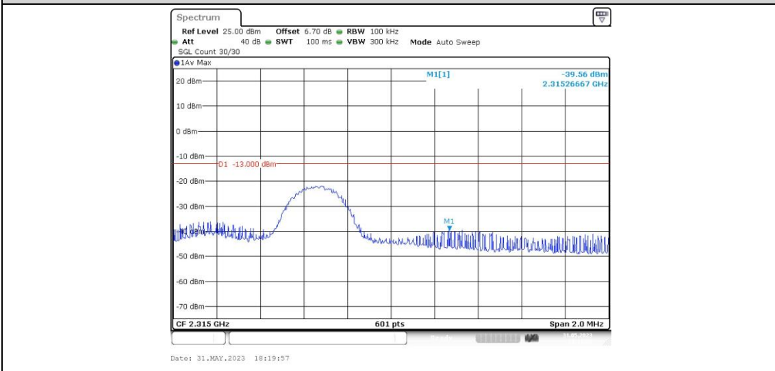
Band40-5MHz-16QAM-38775-1RB#24
