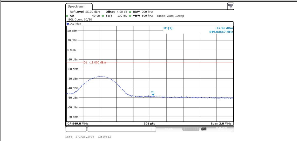
Band5-10MHz-QPSK-20600-1RB#49
