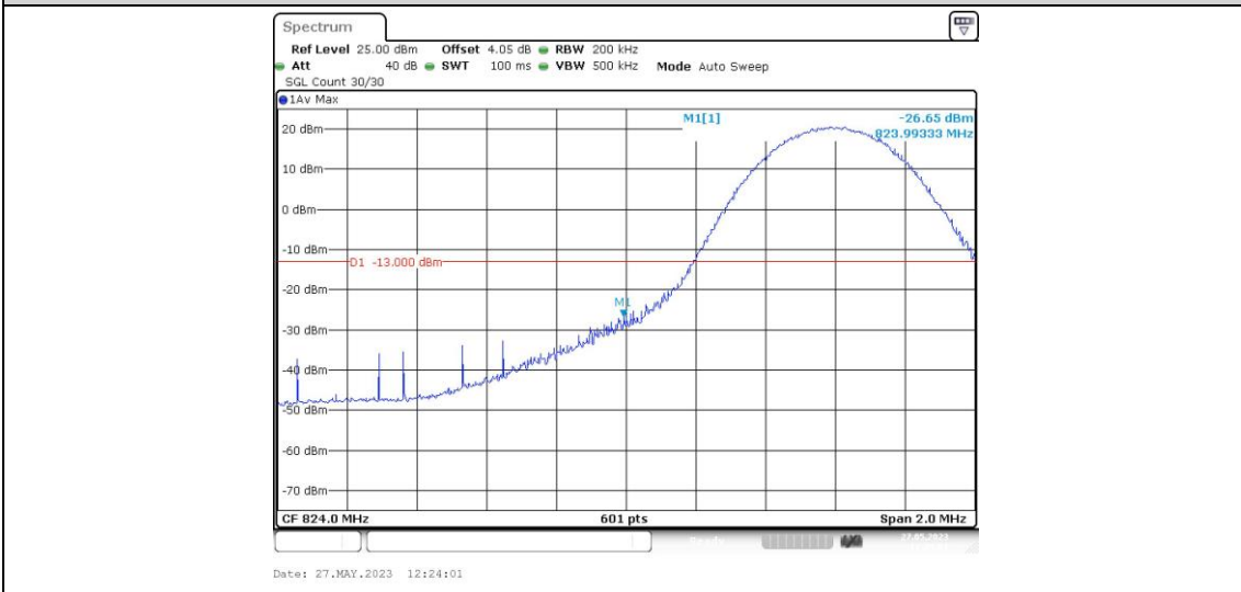
Band5-10MHz-16QAM-20450-1RB#49
