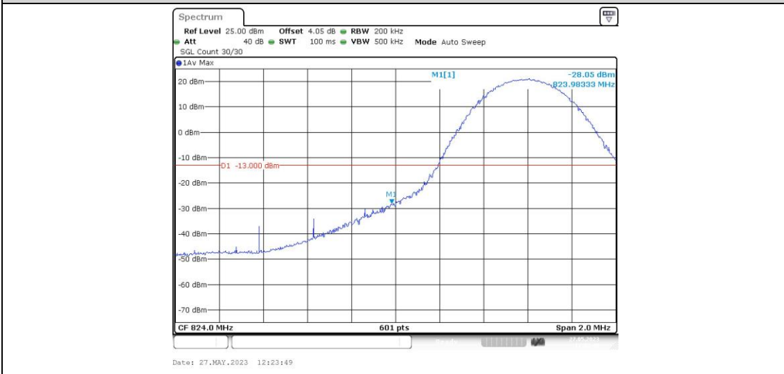
Band5-10MHz-QPSK-20450-1RB#49
