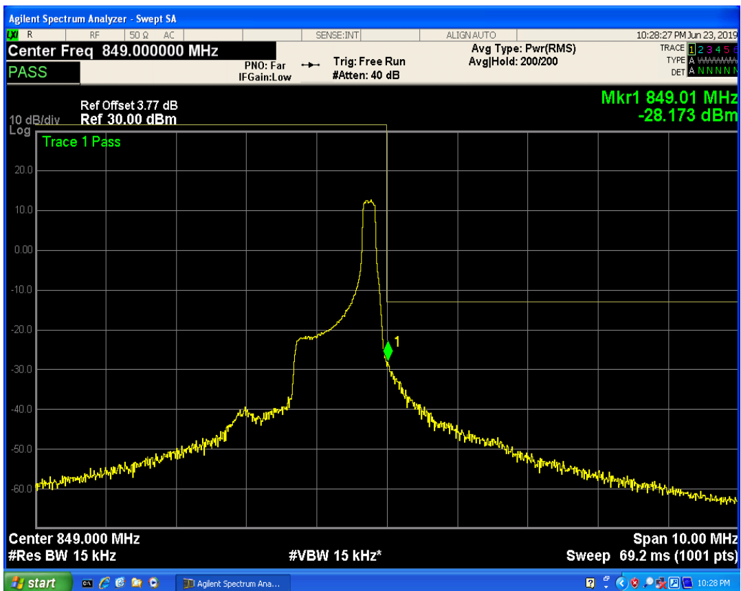
LTE Band5 QAM16 BW=1.4MHz Channel=20643 RB Size=3 Position=#0
