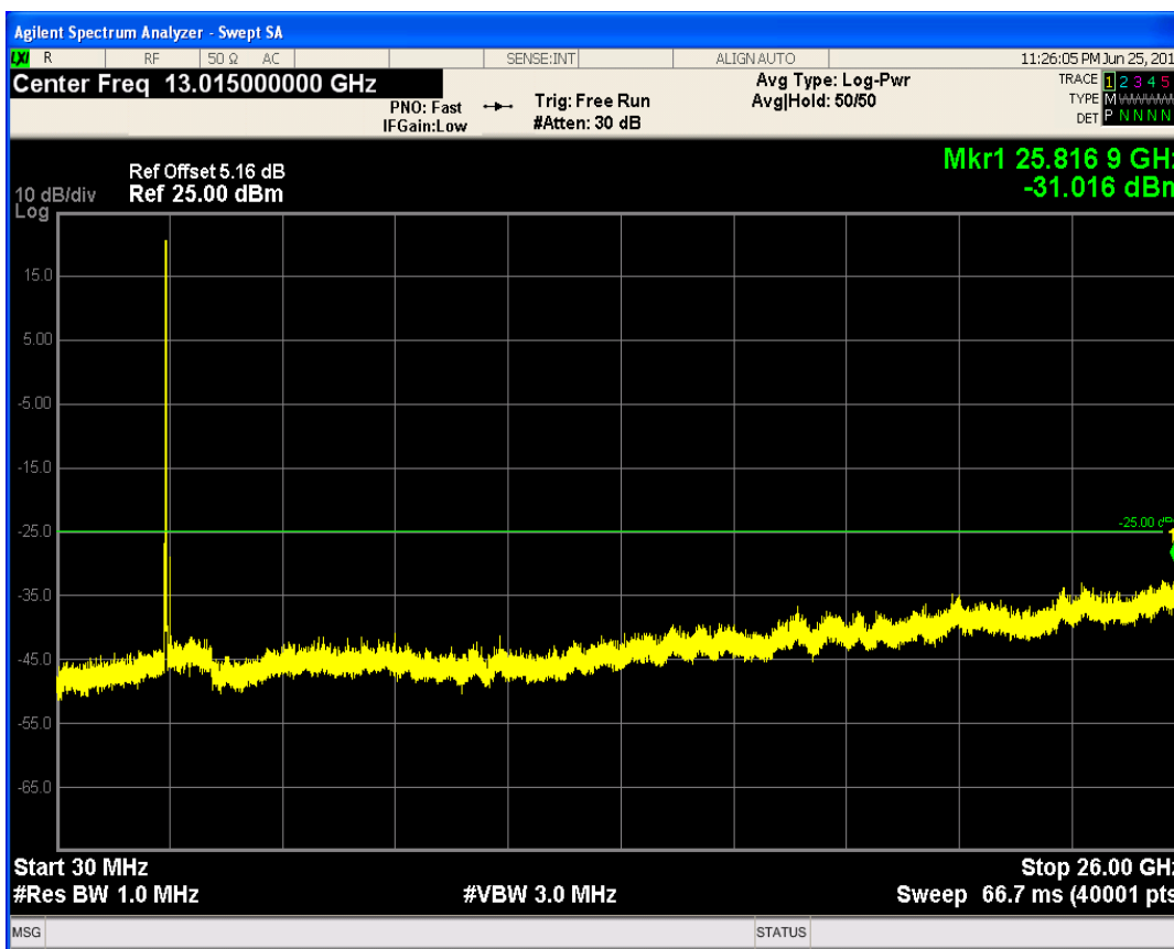
LTE Band41 QPSK BW=15MHz Channel=40115 RB Size=36 Position=#Max
