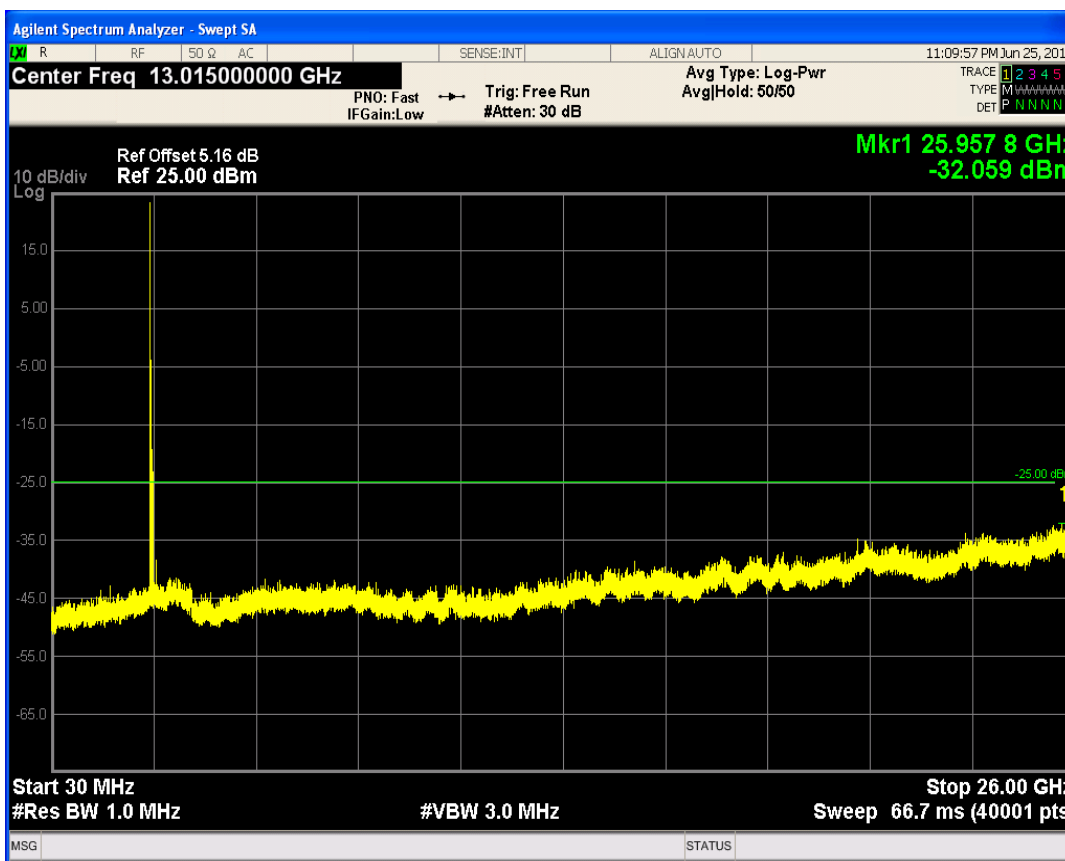
LTE Band41 QPSK BW=5MHz Channel=41215 RB Size=1 Position=#0
