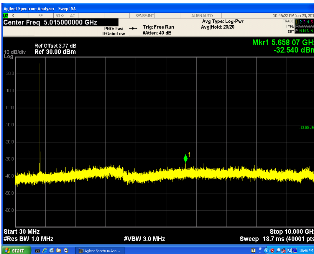
LTE Band5 QAM16 BW=1.4MHz Channel=20643 RB Size=1 Position=#Mid
