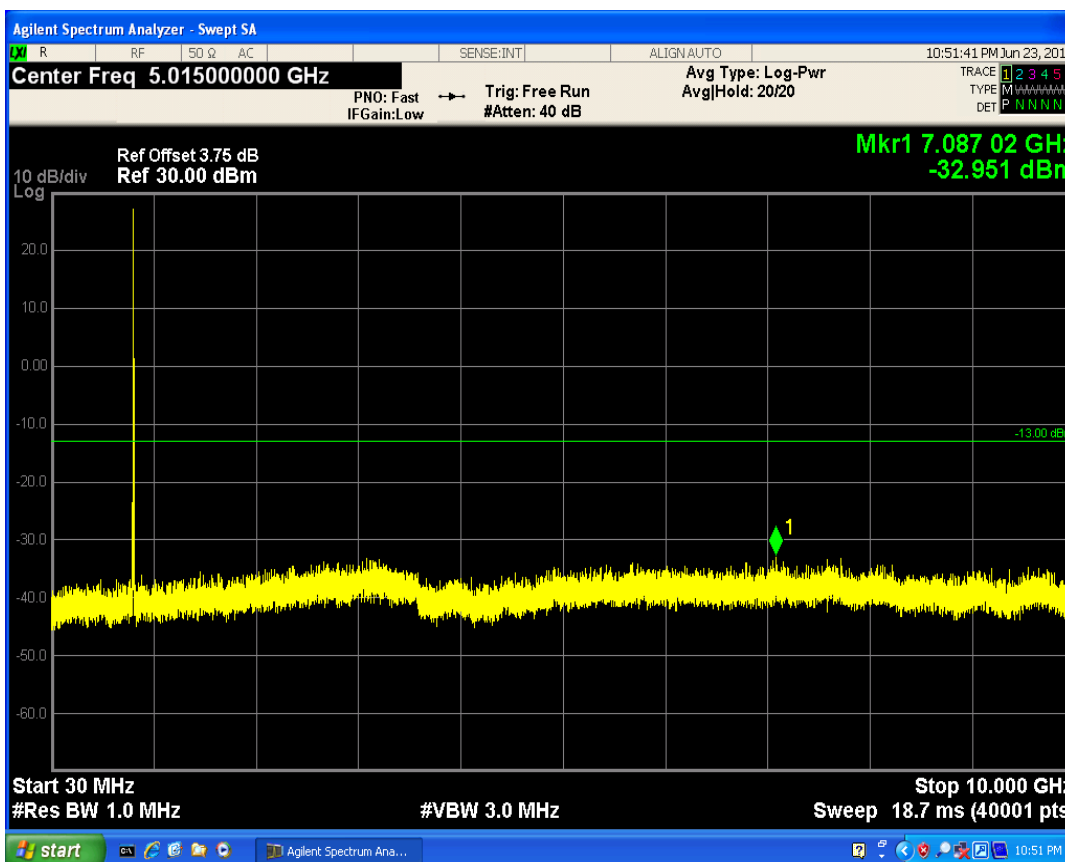
LTE Band5 QAM16 BW=5MHz Channel=20425 RB Size=12 Position=#0
