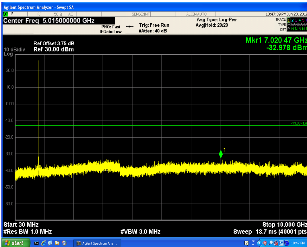
LTE Band5 QPSK BW=3MHz Channel=20415 RB Size=1 Position=#Mid
