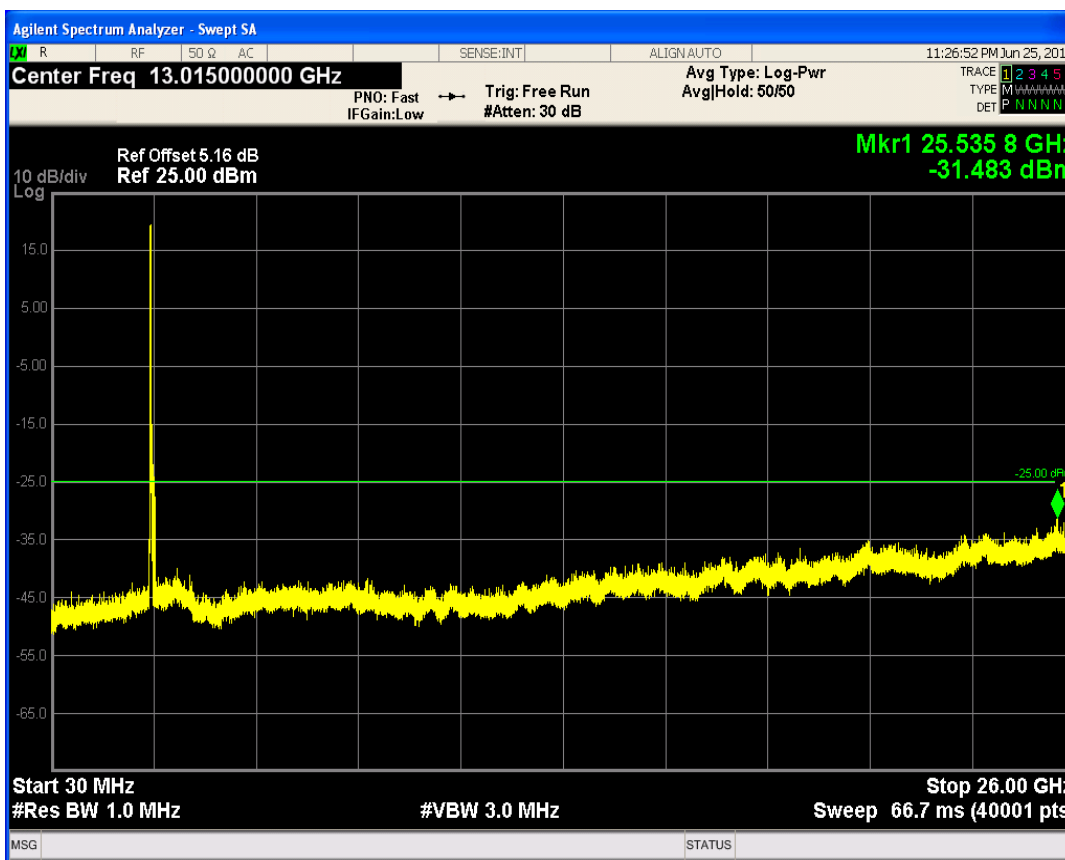
LTE Band41 QPSK BW=15MHz Channel=40115 RB Size=36 Position=#0
