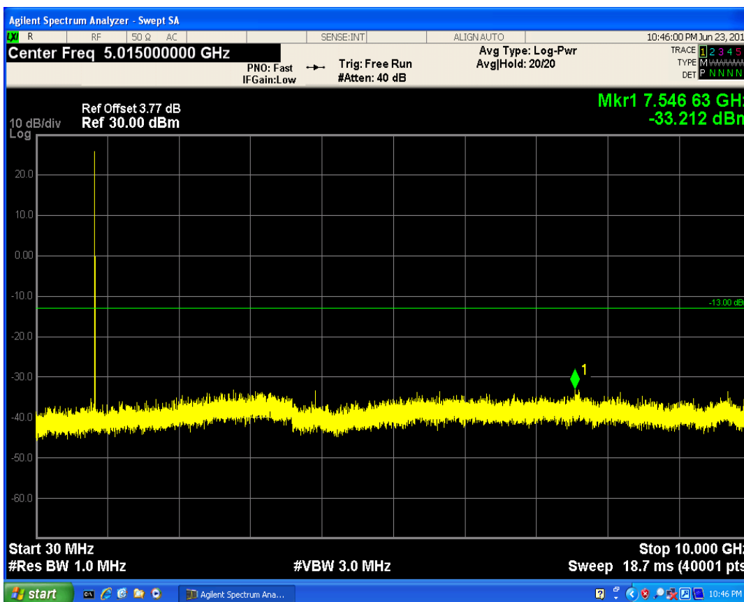
LTE Band5 QPSK BW=1.4MHz Channel=20643 RB Size=3 Position=#0
