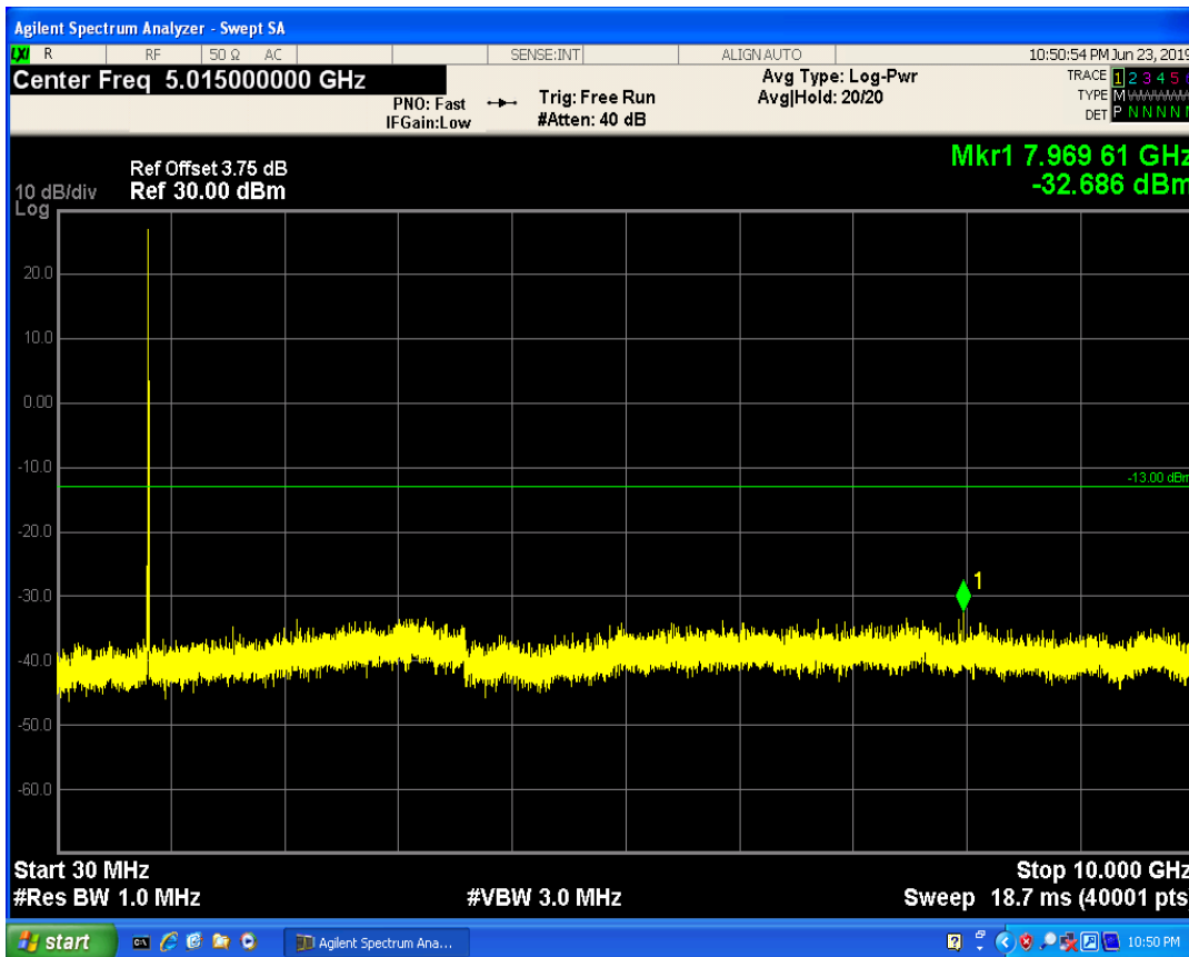
LTE Band5 QPSK BW=5MHz Channel=20425 RB Size=12 Position=#Max
