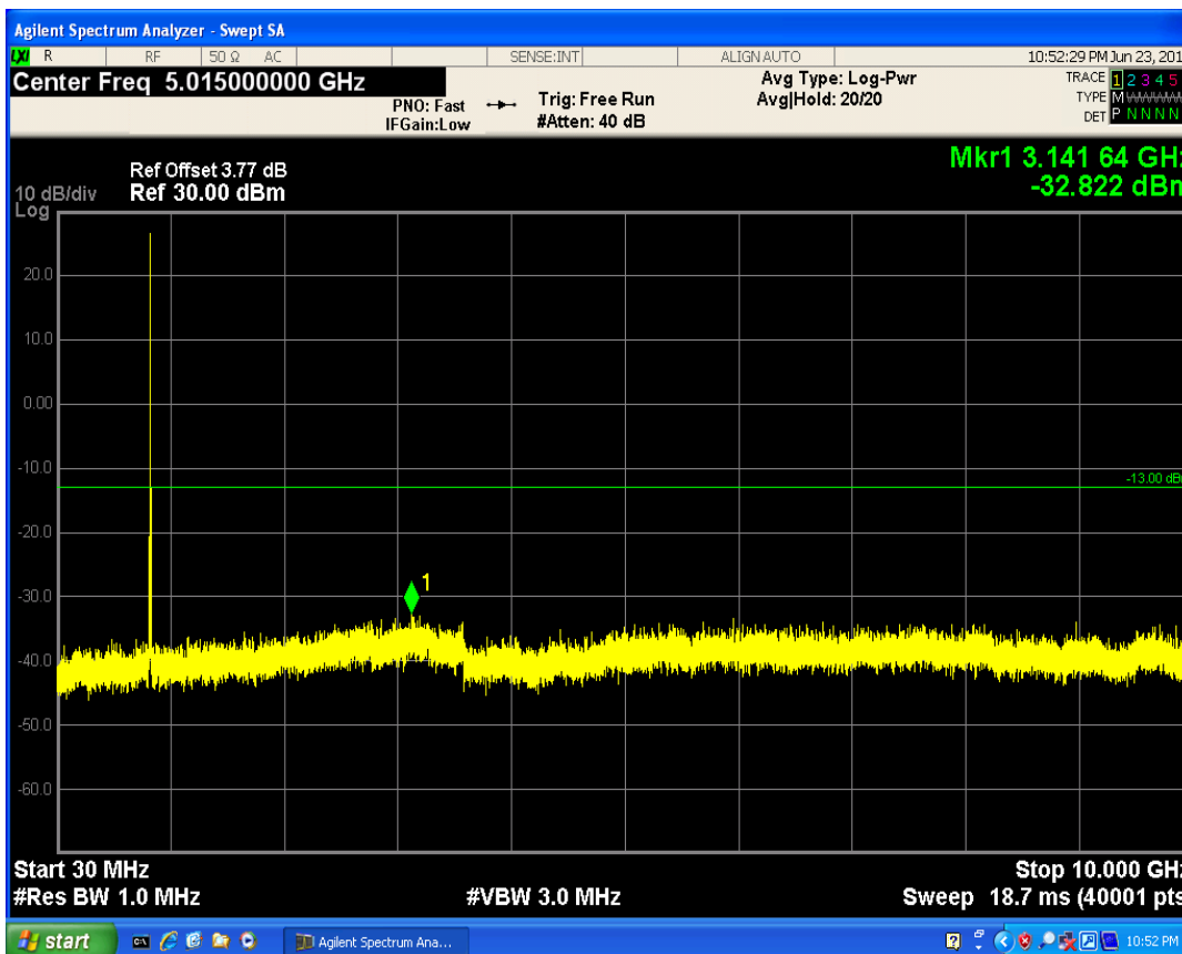
LTE Band5 QPSK BW=5MHz Channel=20625 RB Size=12 Position=#0
