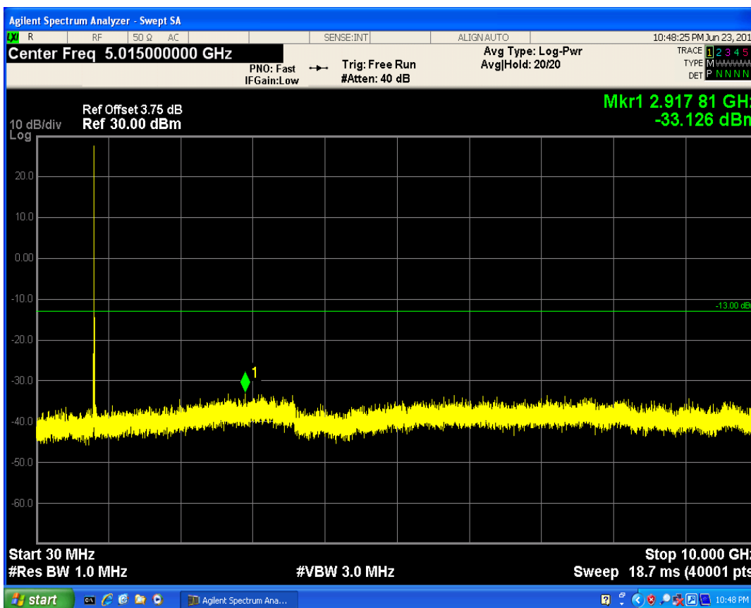
LTE Band5 QAM16 BW=3MHz Channel=20415 RB Size=8 Position=#0
