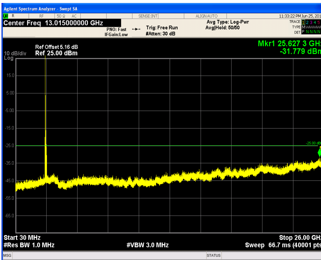
LTE Band41 QPSK BW=20MHz Channel=40140 RB Size=1 Position=#Max
