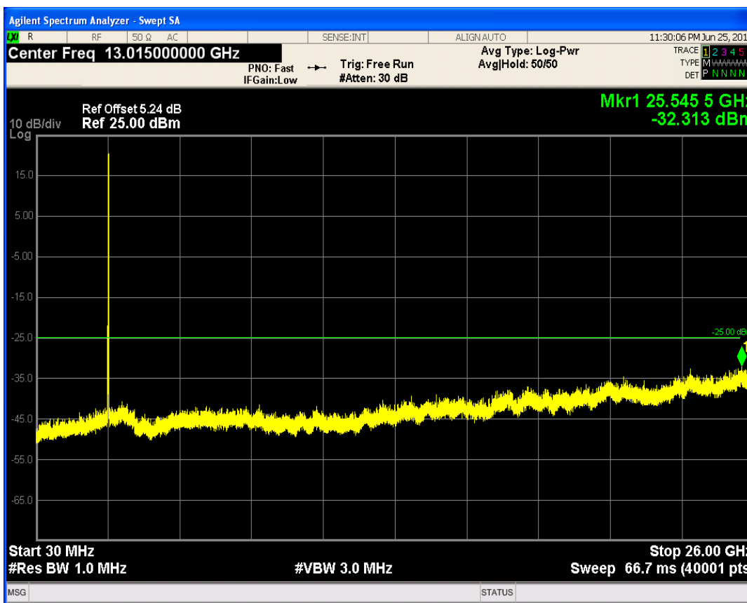
LTE Band41 QPSK BW=15MHz Channel=41165 RB Size=36 Position=#Max
