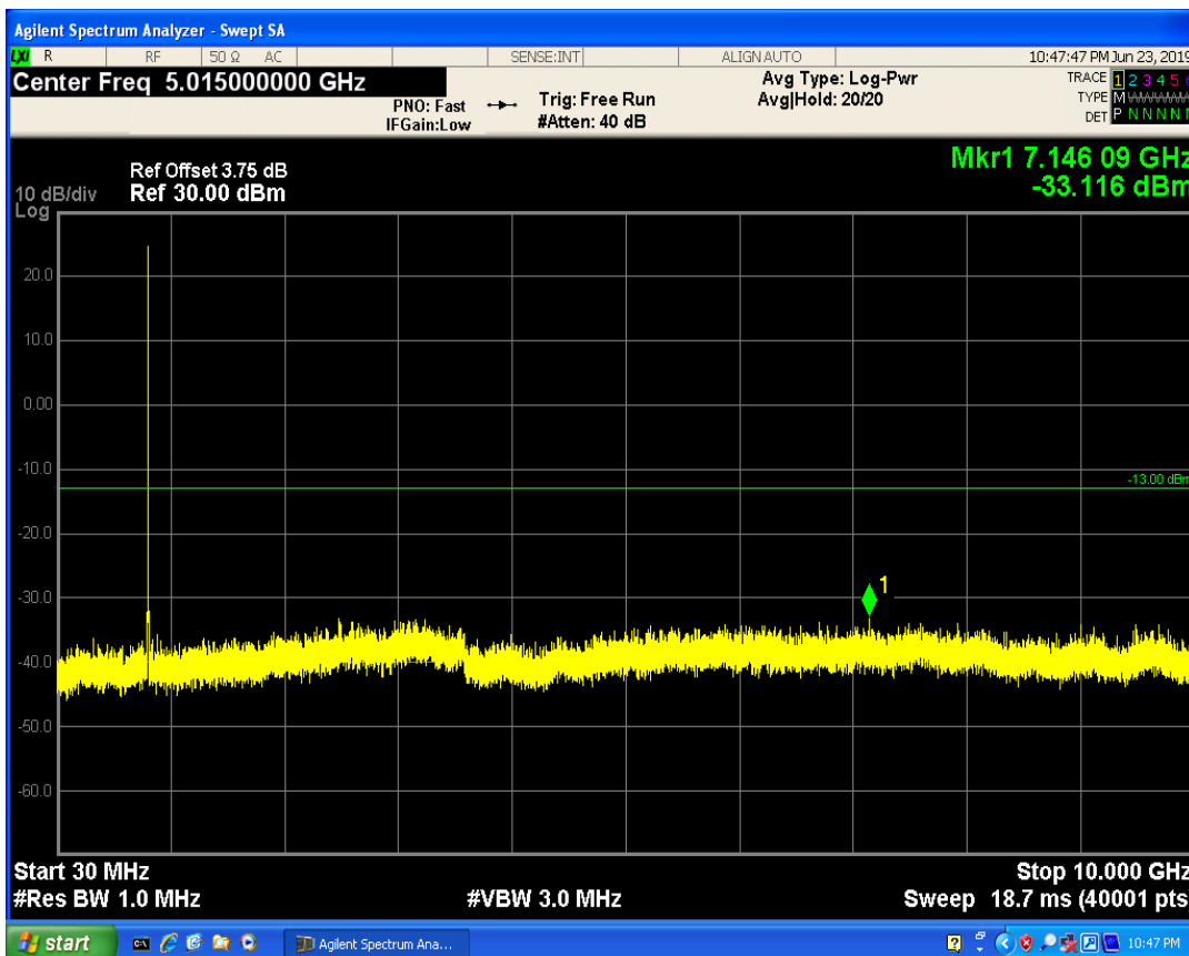
LTE Band5 QPSK BW=3MHz Channel=20415 RB Size=8 Position=#Max
