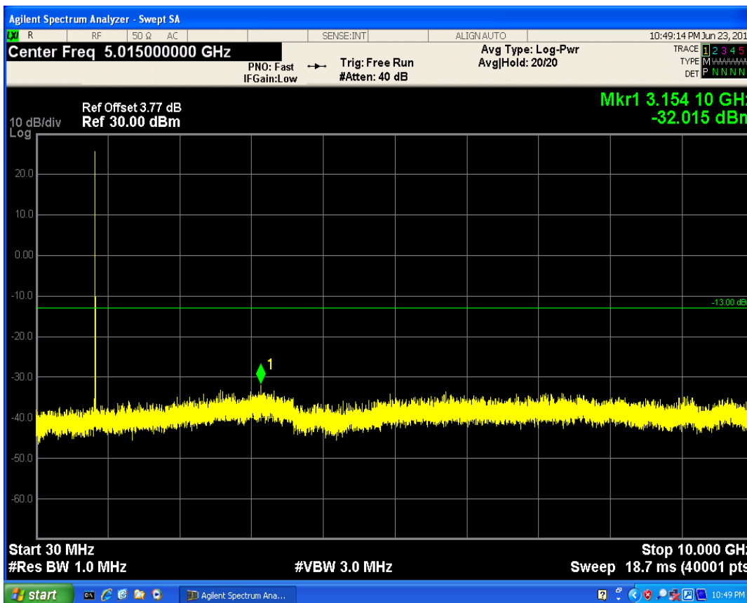
LTE Band5 QPSK BW=3MHz Channel=20635 RB Size=8 Position=#0
