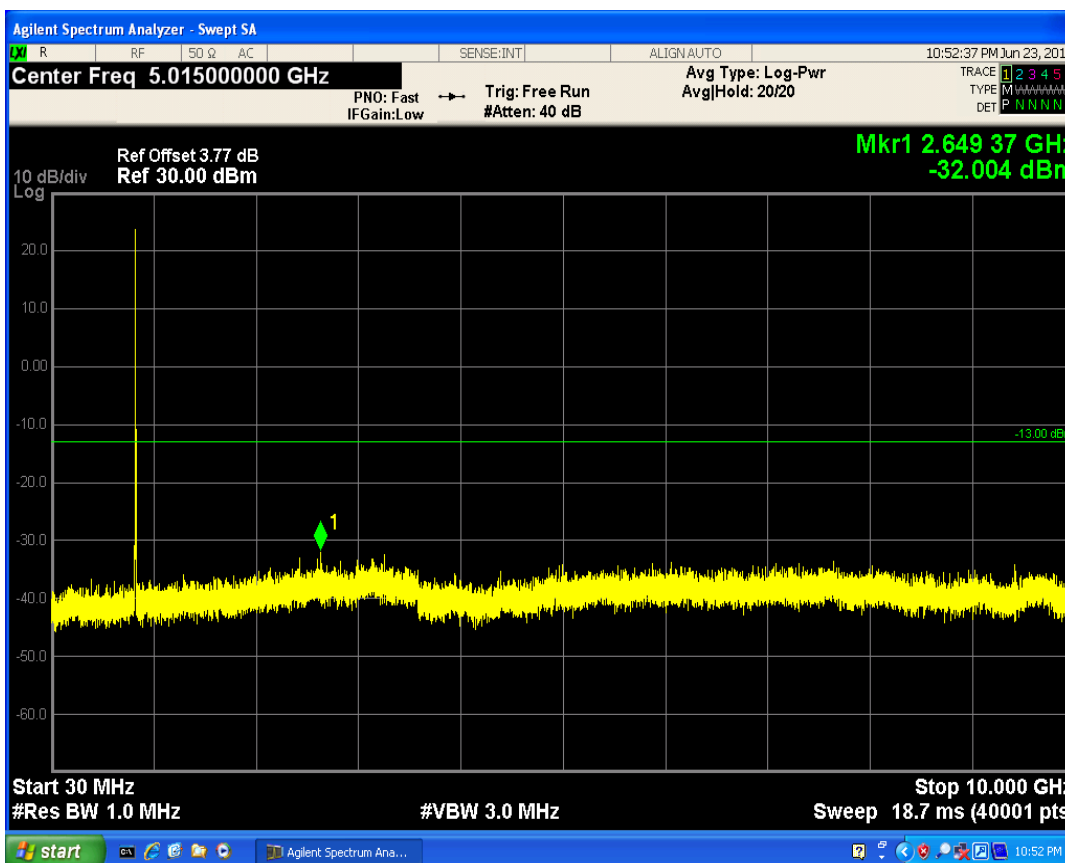
LTE Band5 QPSK BW=5MHz Channel=20625 RB Size=12 Position=#Max
