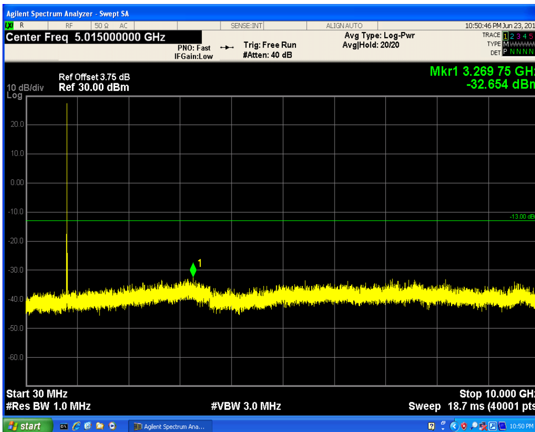
LTE Band5 QPSK BW=5MHz Channel=20425 RB Size=12 Position=#0
