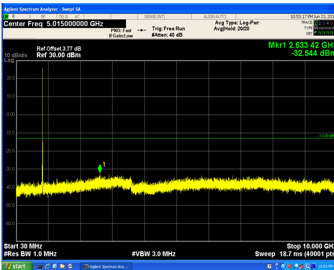
LTE Band5 QAM16 BW=5MHz Channel=20625 RB Size=12 Position=#Max
