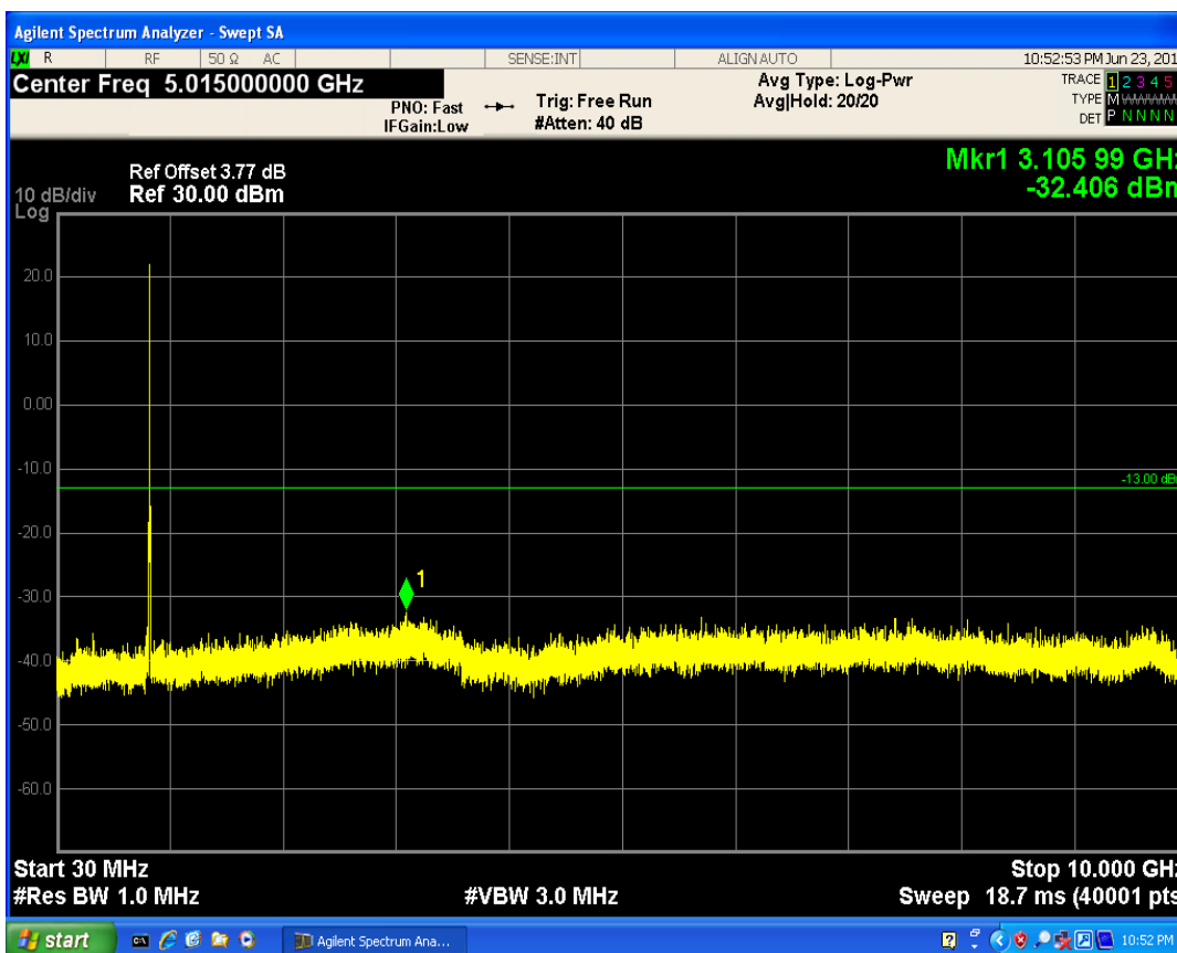
LTE Band5 QAM16 BW=5MHz Channel=20625 RB Size=1 Position=#Mid
