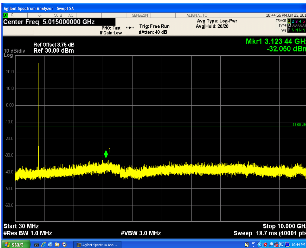
LTE Band5 QAM16 BW=1.4MHz Channel=20407 RB Size=1 Position=#Mid
