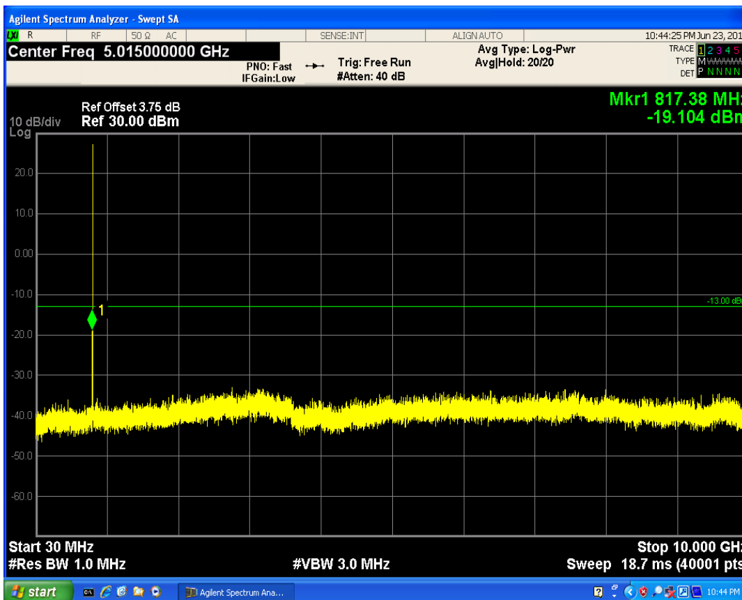
LTE Band5 QPSK BW=1.4MHz Channel=20407 RB Size=1 Position=#Mid
