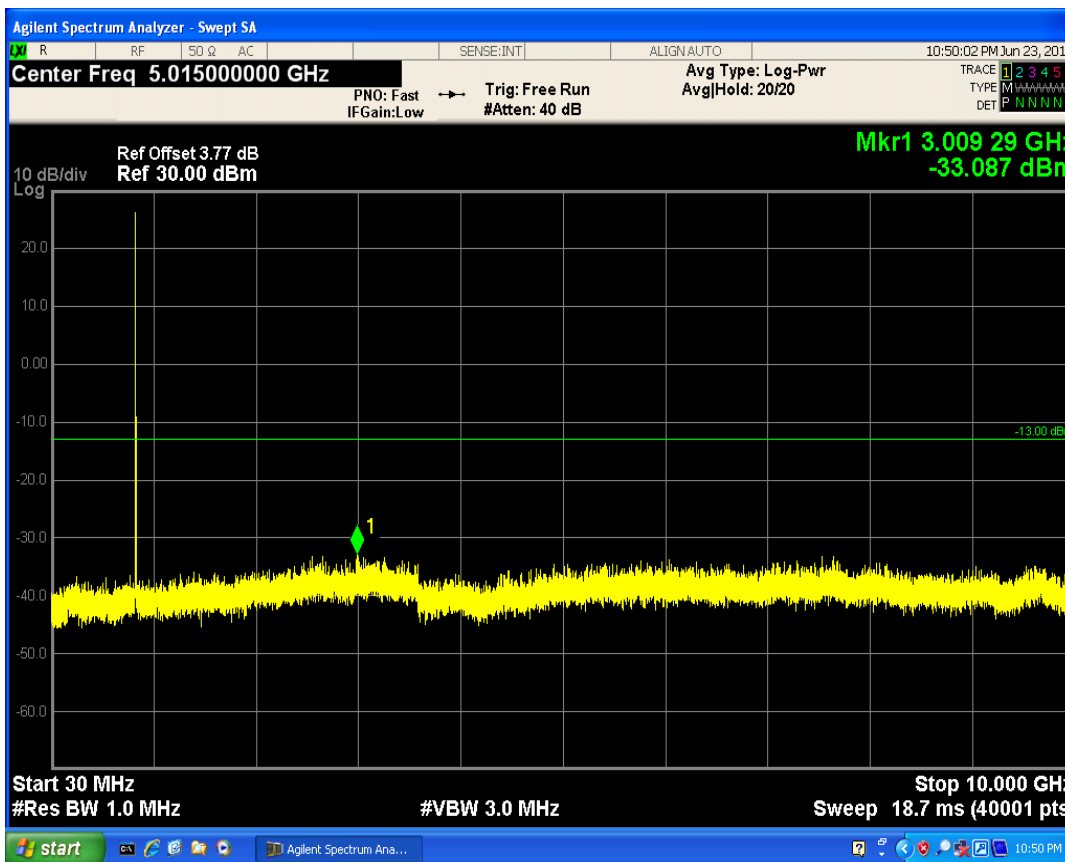
LTE Band5 QAM16 BW=3MHz Channel=20635 RB Size=8 Position=#0
