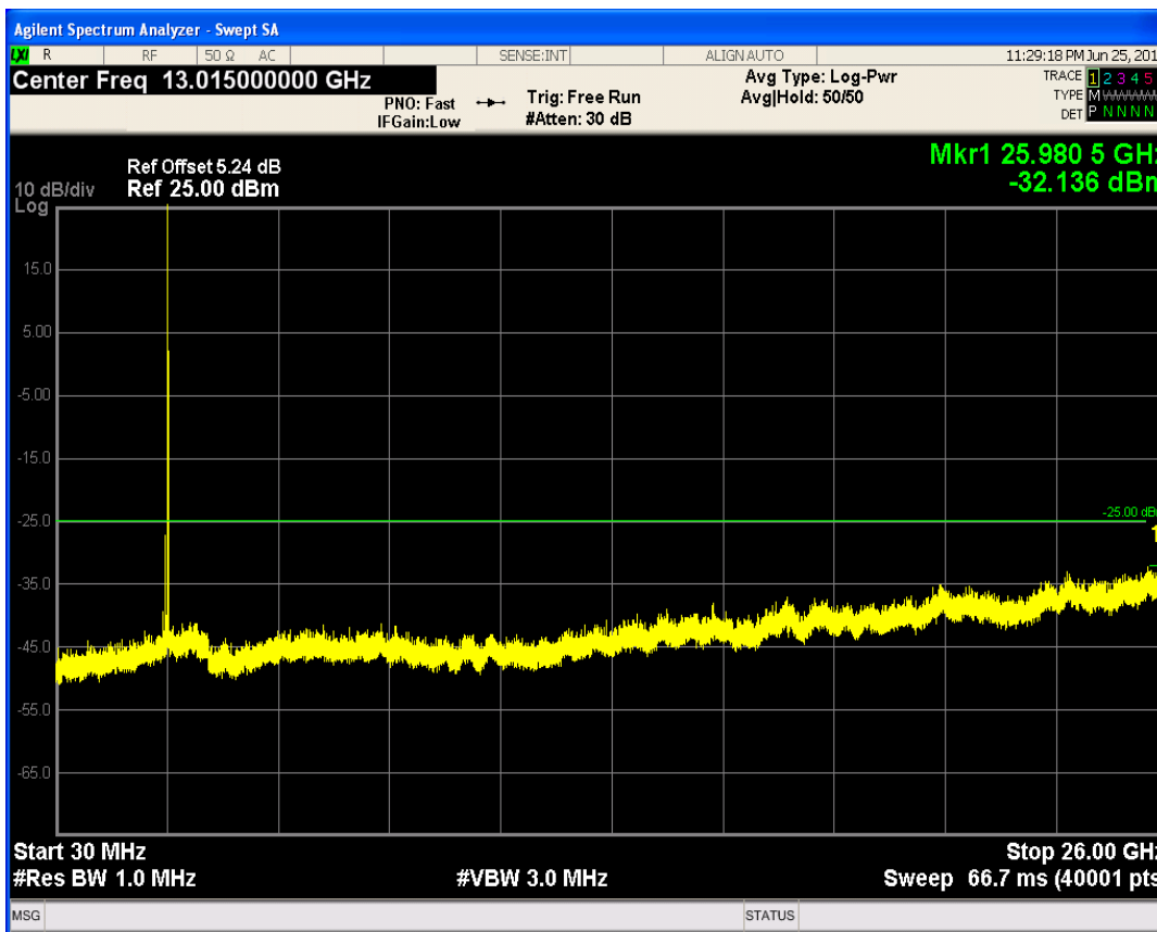
LTE Band41 QPSK BW=5MHz Channel=41215 RB Size=1 Position=#Max
