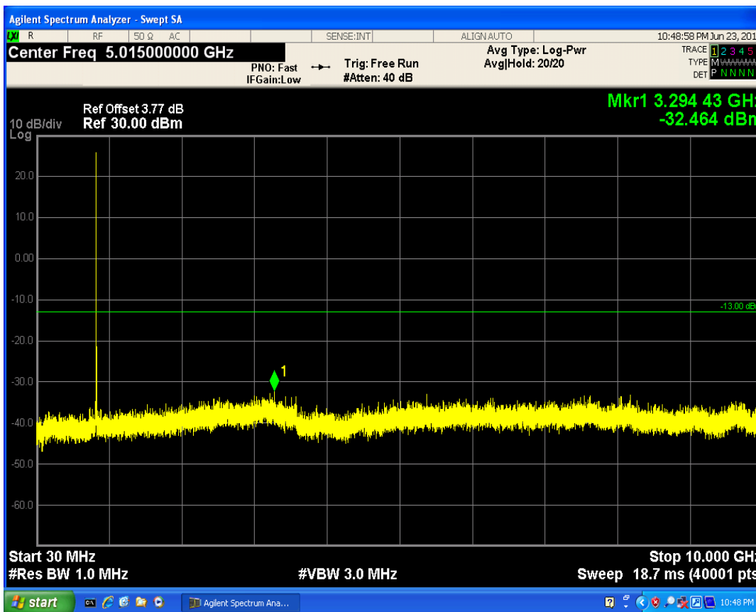
LTE Band5 QPSK BW=3MHz Channel=20635 RB Size=1 Position=#Mid
