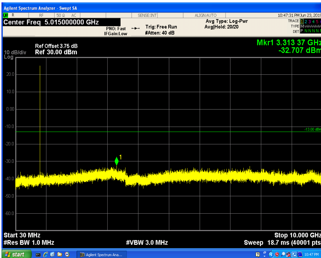
LTE Band5 QPSK BW=3MHz Channel=20415 RB Size=8 Position=#0
