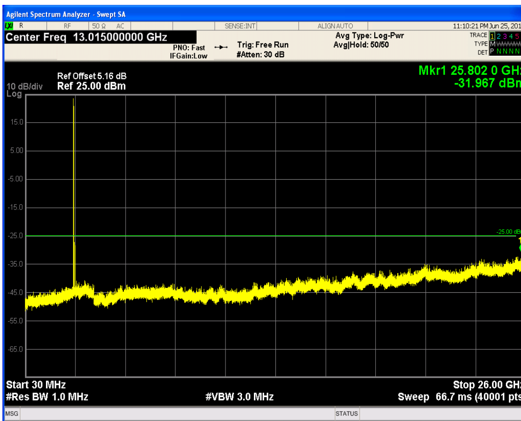
LTE Band41 QPSK BW=5MHz Channel=40065 RB Size=12 Position=#0
