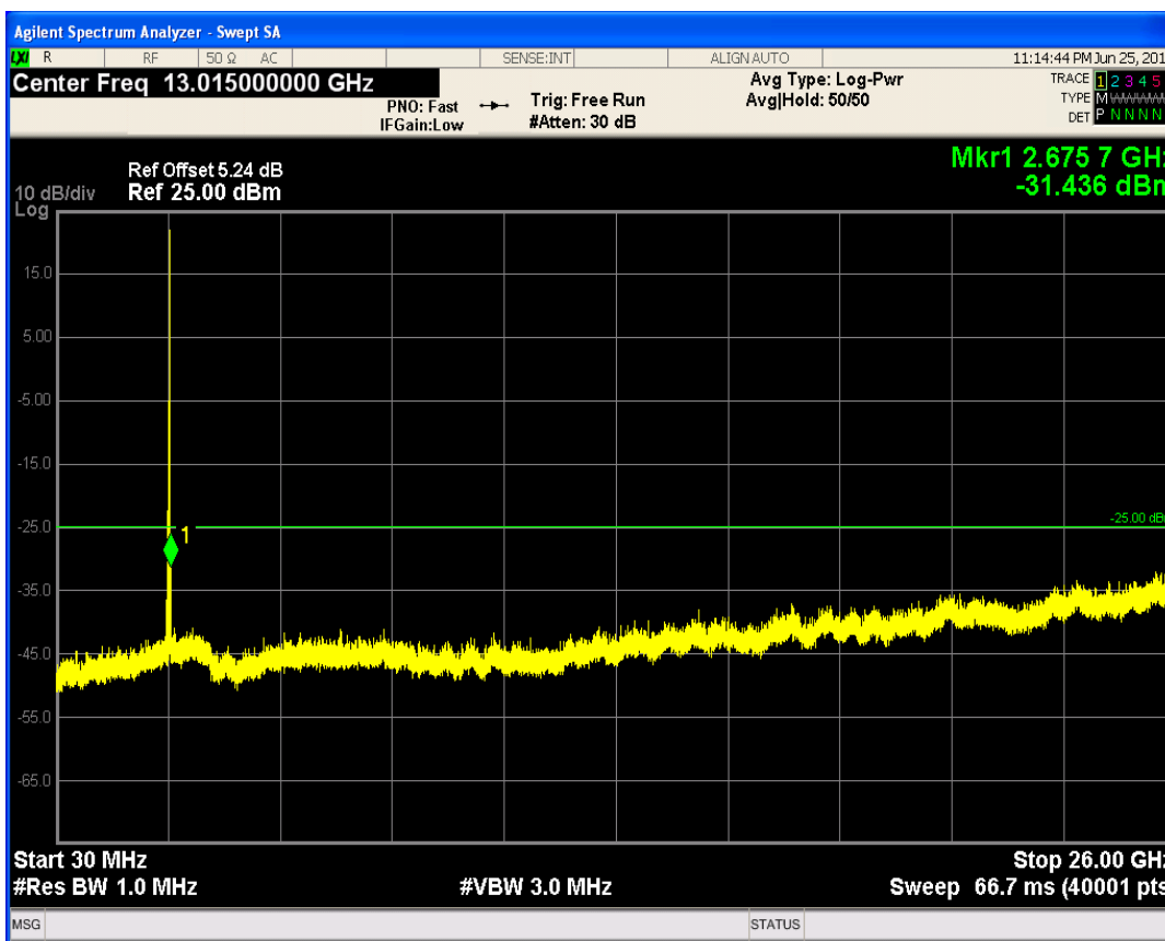
LTE Band41 QPSK BW=5MHz Channel=41215 RB Size=12 Position=#Max
