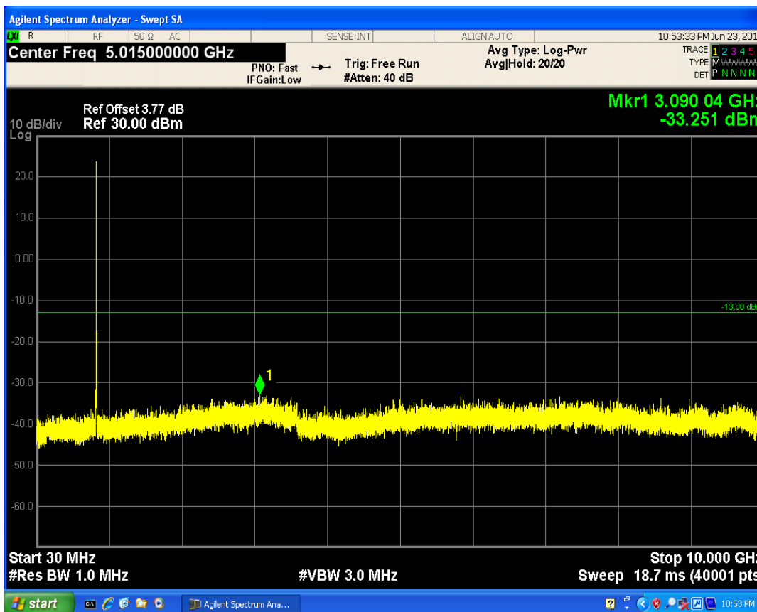
LTE Band5 QAM16 BW=5MHz Channel=20625 RB Size=12 Position=#0
