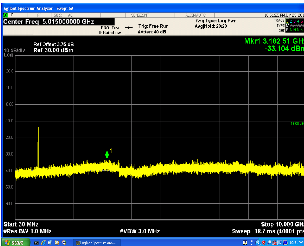
LTE Band5 QAM16 BW=5MHz Channel=20425 RB Size=1 Position=#Mid
