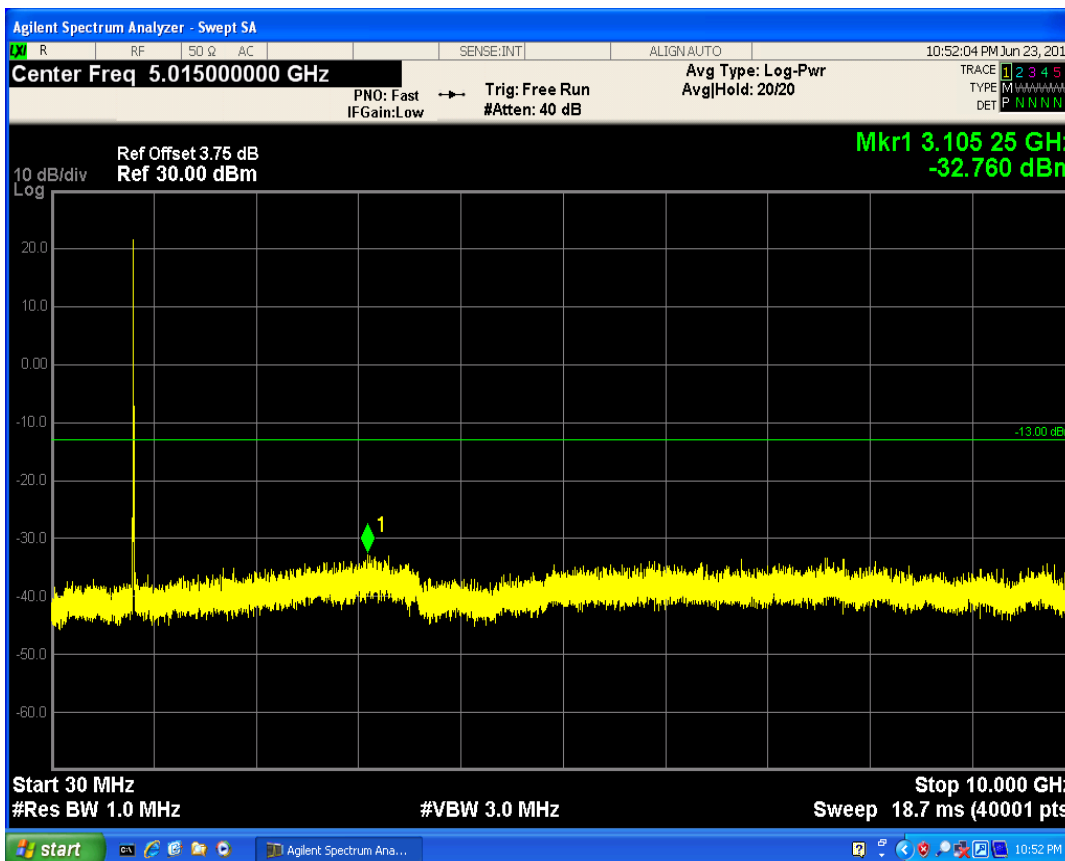
LTE Band5 QPSK BW=5MHz Channel=20625 RB Size=1 Position=#Mid
