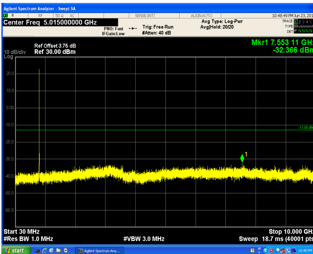
LTE Band5 QAM16 BW=3MHz Channel=20415 RB Size=8 Position=#Max
