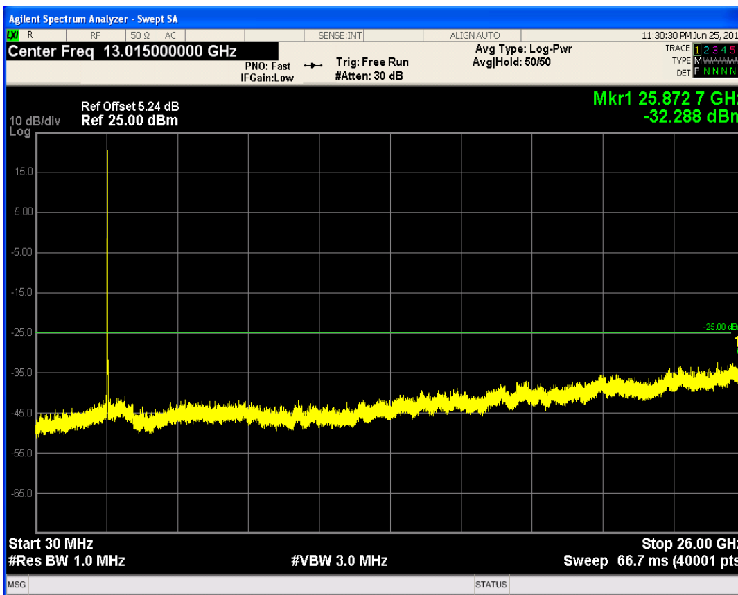
LTE Band41 QPSK BW=5MHz Channel=41215 RB Size=12 Position=#0
