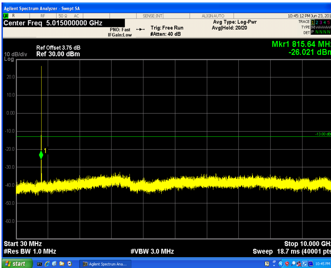
LTE Band5 QAM16 BW=1.4MHz Channel=20407 RB Size=3 Position=#0
