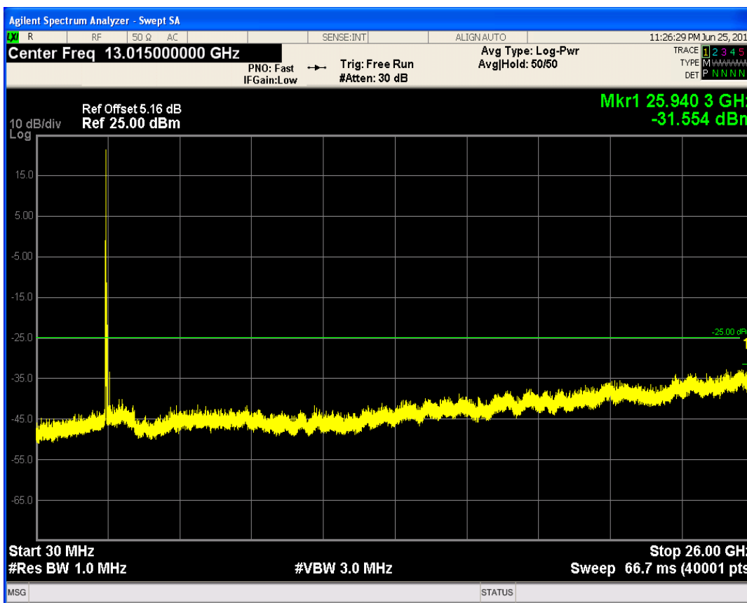
LTE Band41 QPSK BW=20MHz Channel=40140 RB Size=1 Position=#0
