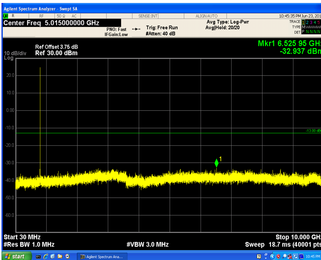
LTE Band5 QPSK BW=1.4MHz Channel=20643 RB Size=1 Position=#Mid
