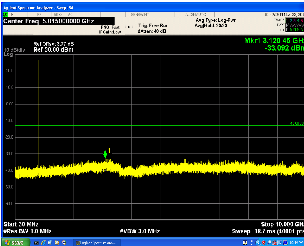
LTE Band5 QPSK BW=3MHz Channel=20635 RB Size=1 Position=#Max
