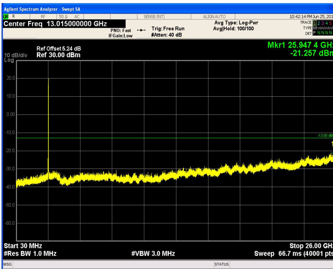
LTE Band41 QAM16 BW=10MHz Channel=40090 RB Size=50 Position=#0
