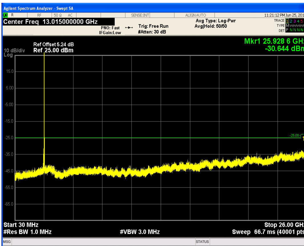
LTE Band41 QPSK BW=10MHz Channel=41190 RB Size=1 Position=#Max
