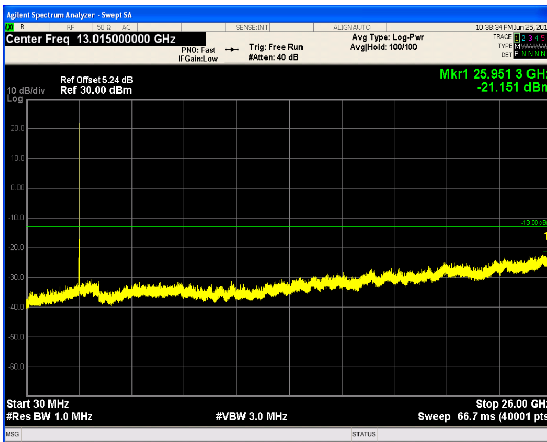
LTE Band41 QPSK BW=5MHz Channel=40065 RB Size=25 Position=#0
