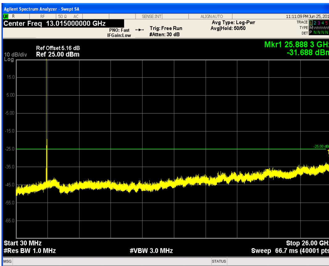
LTE Band41 QAM16 BW=20MHz Channel=41140 RB Size=50 Position=#0
