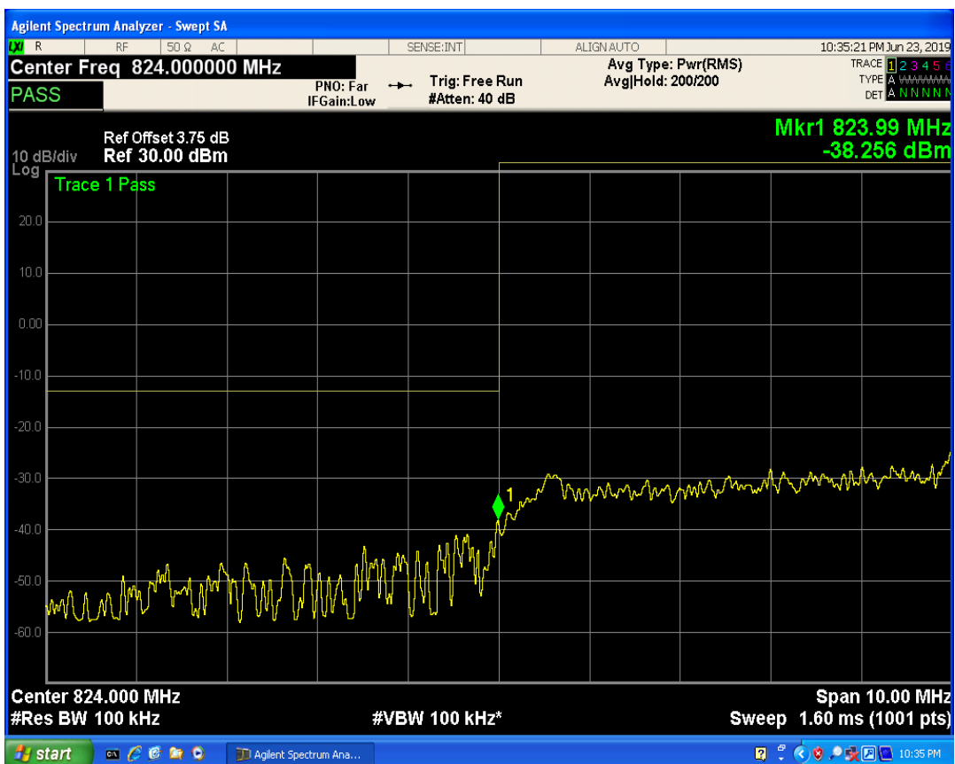
LTE Band5 QAM16 BW=10MHz Channel=20450 RB Size=25 Position=#0
