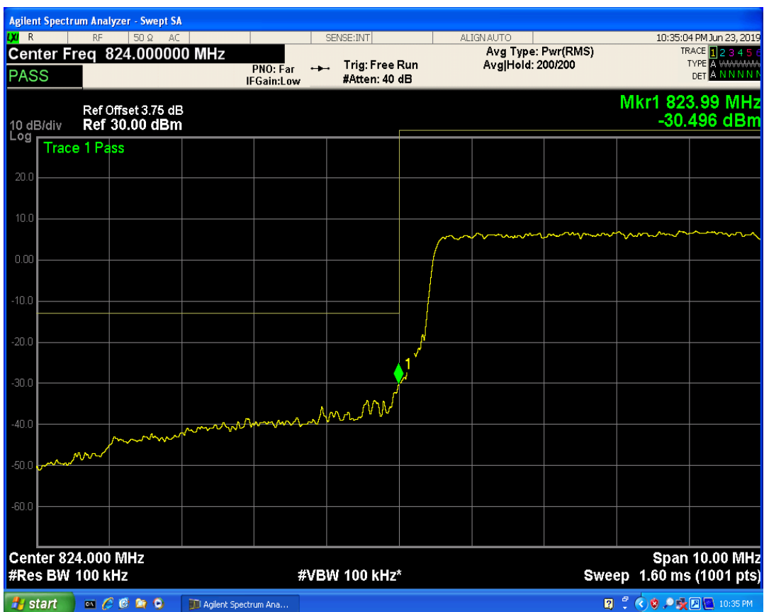
LTE Band5 QPSK BW=10MHz Channel=20450 RB Size=25 Position=#Max
