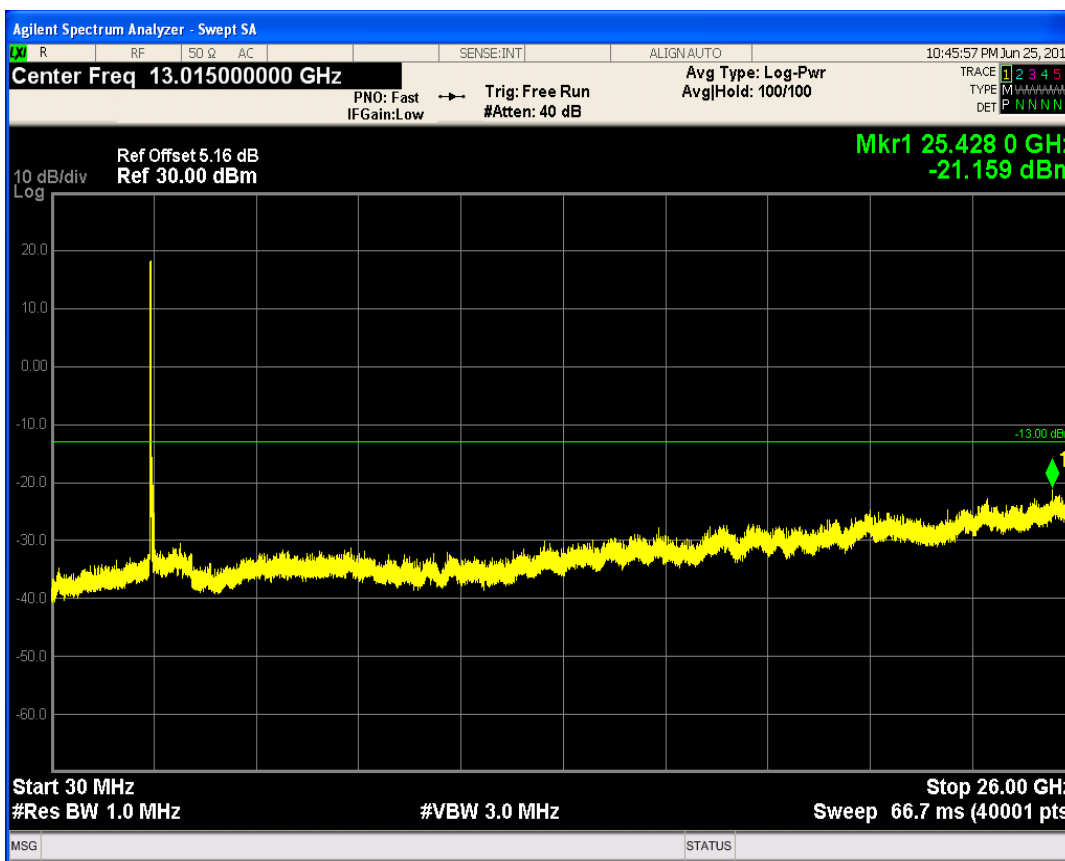
LTE Band41 QPSK BW=15MHz Channel=41165 RB Size=75 Position=#0
