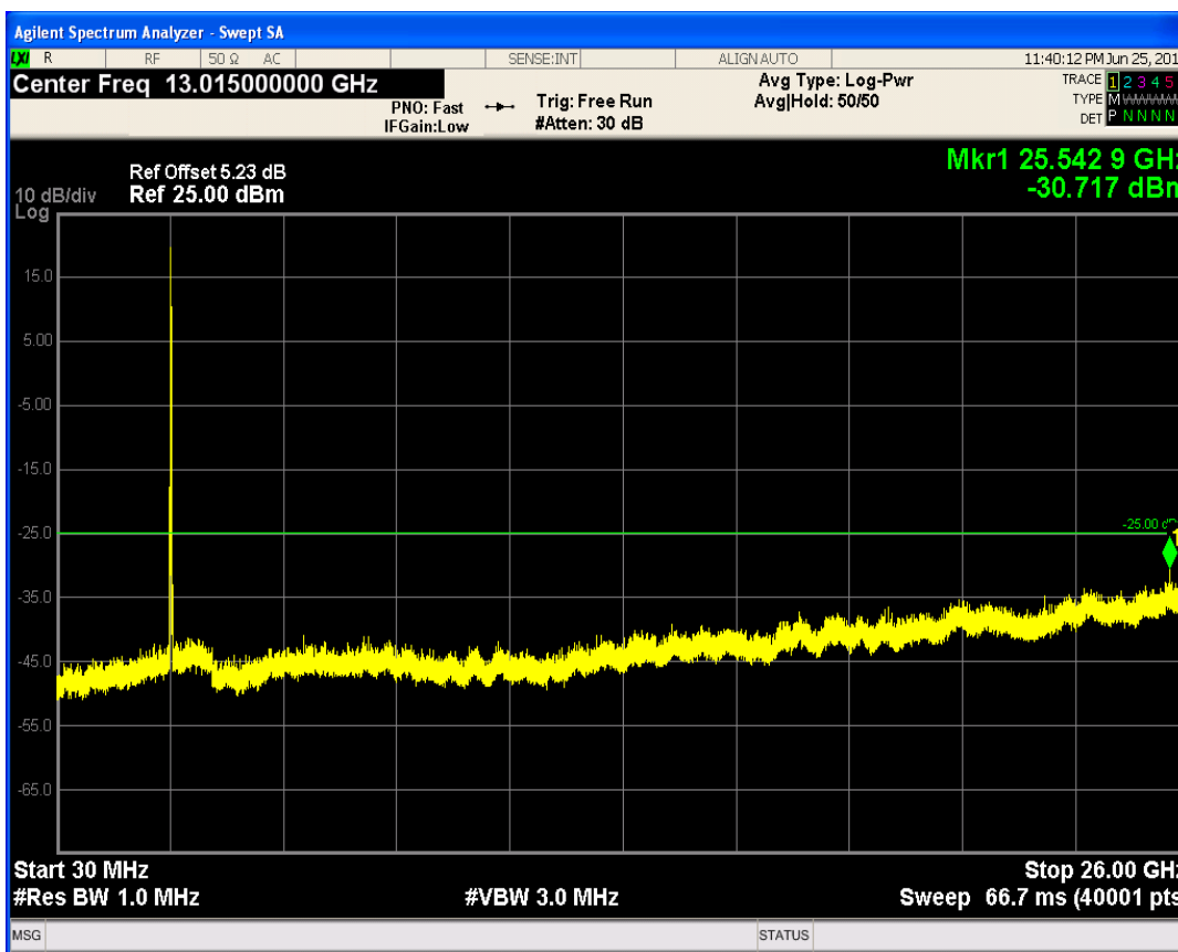
LTE Band41 QAM16 BW=20MHz Channel=41140 RB Size=50 Position=#Max
