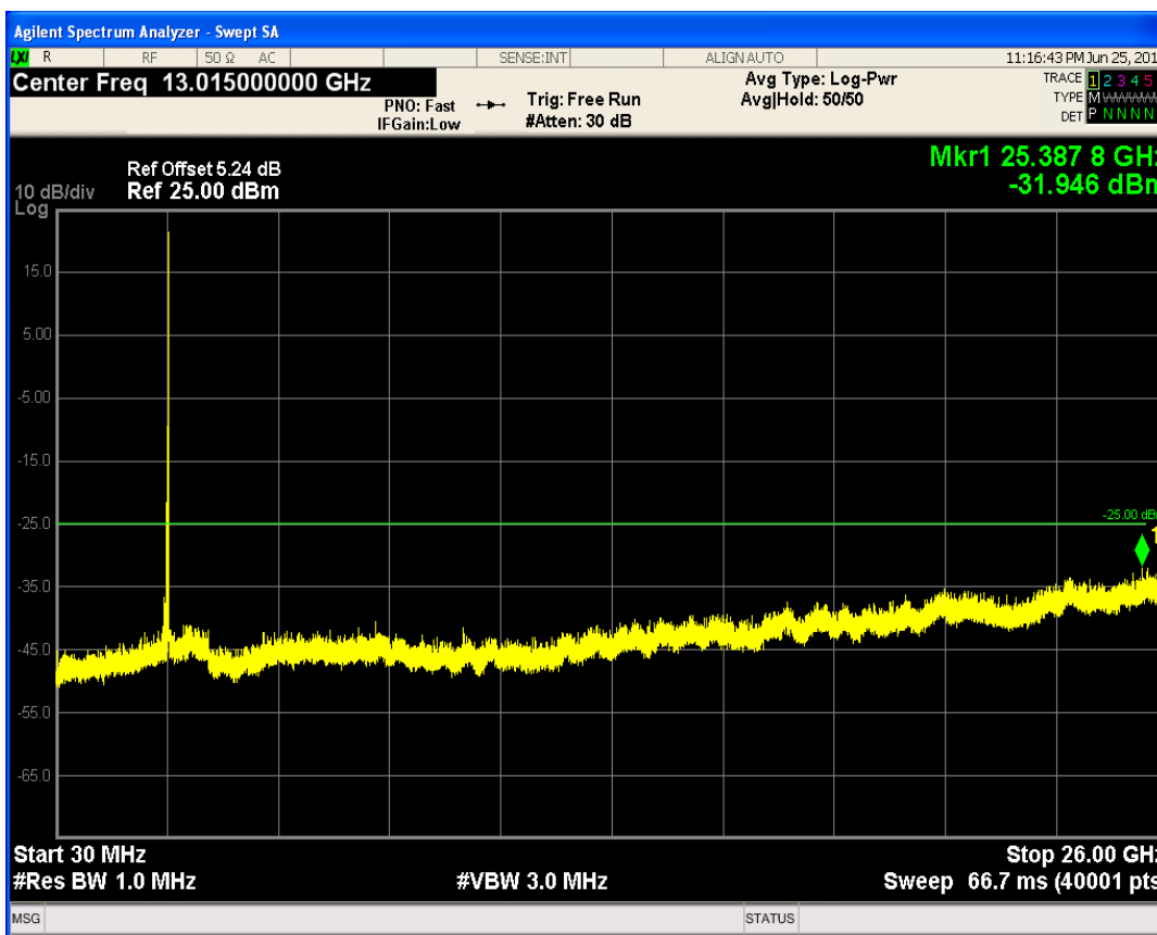
LTE Band41 QPSK BW=20MHz Channel=41140 RB Size=1 Position=#0
