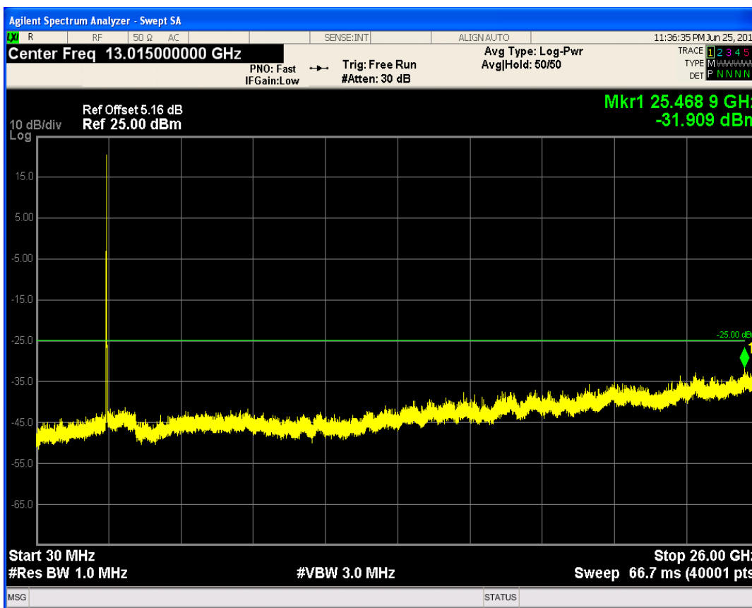
LTE Band41 QAM16 BW=5MHz Channel=40065 RB Size=1 Position=#Max
