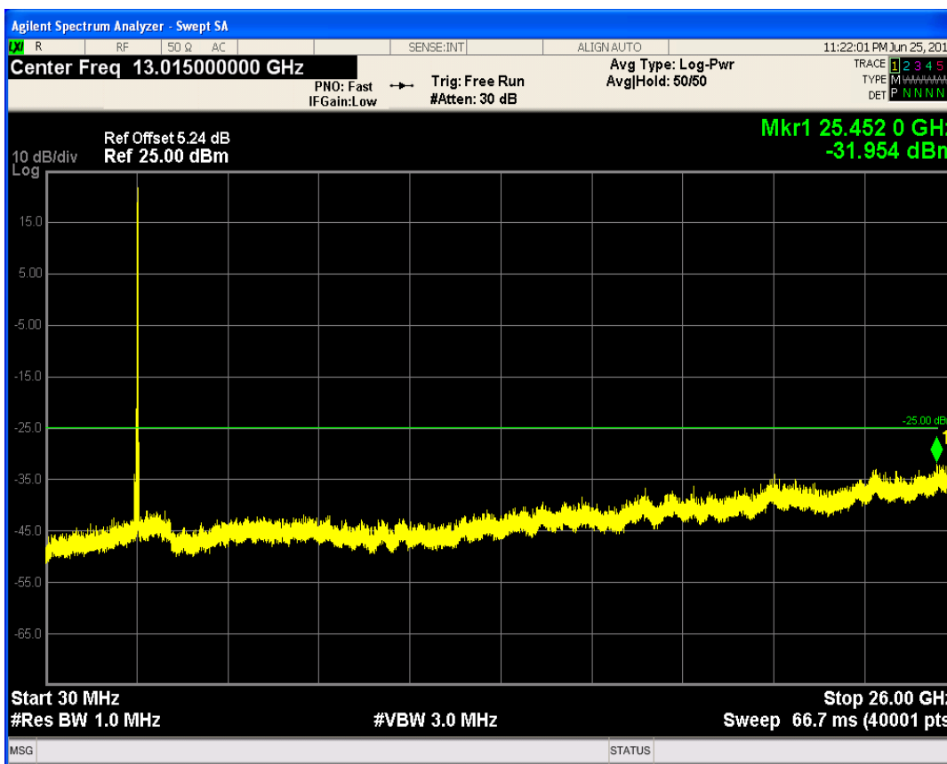
LTE Band41 QAM16 BW=5MHz Channel=40065 RB Size=12 Position=#Max
