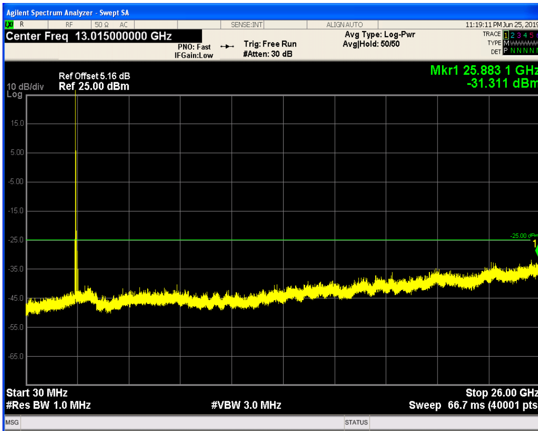
LTE Band41 QAM16 BW=10MHz Channel=41190 RB Size=1 Position=#0
