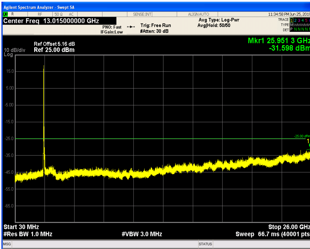
LTE Band41 QPSK BW=20MHz Channel=40140 RB Size=50 Position=#0
