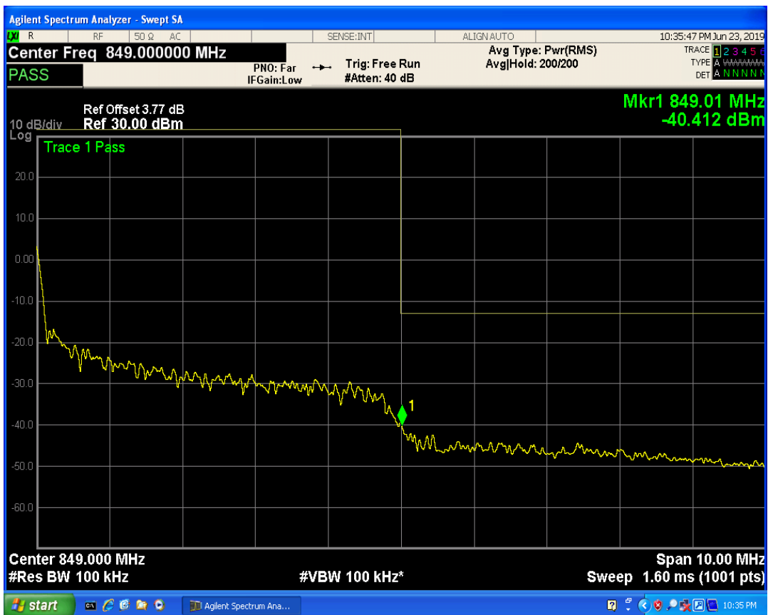
LTE Band5 QPSK BW=10MHz Channel=20600 RB Size=25 Position=#Max
