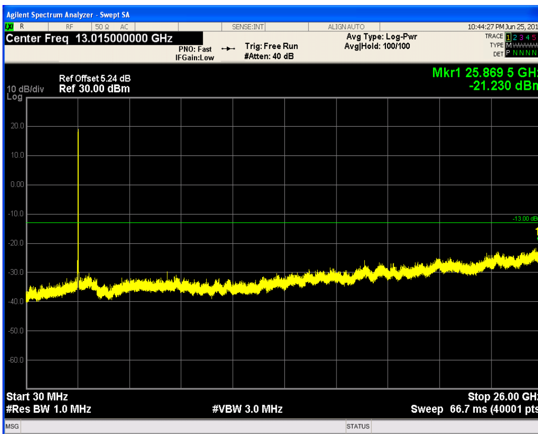
LTE Band41 QPSK BW=15MHz Channel=40115 RB Size=75 Position=#0
