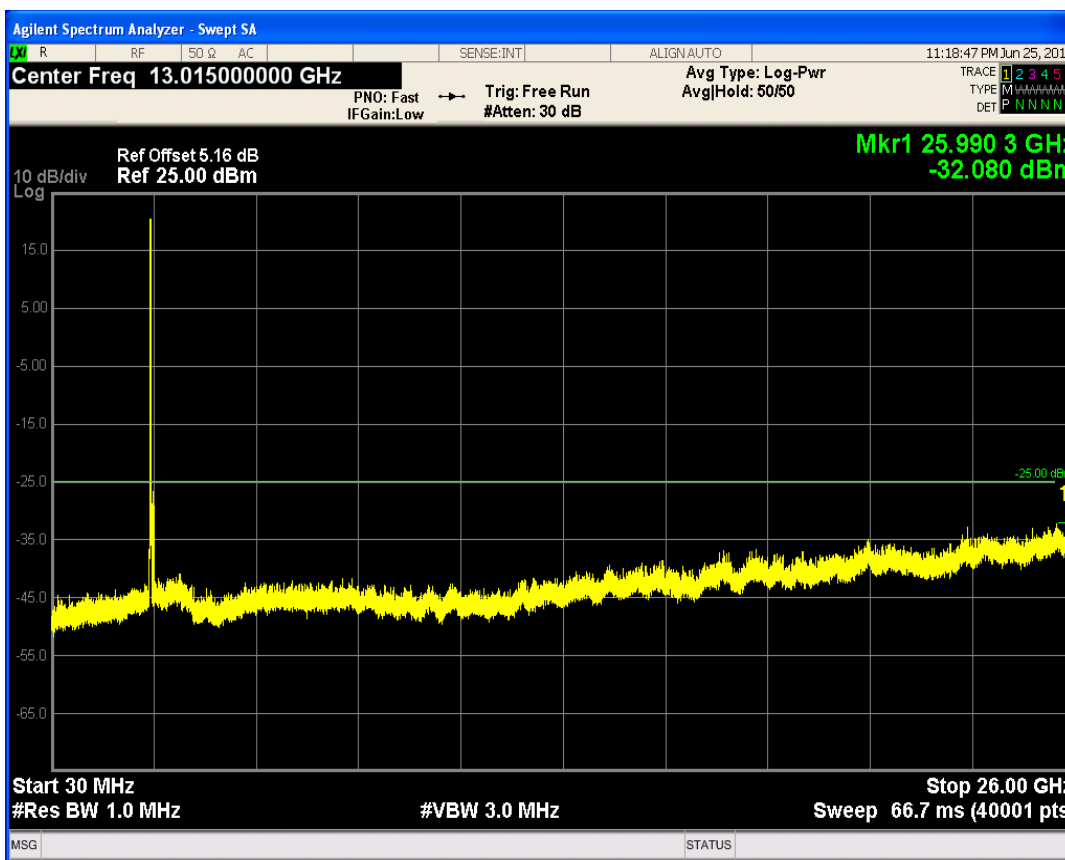
LTE Band41 QPSK BW=10MHz Channel=41190 RB Size=25 Position=#0
