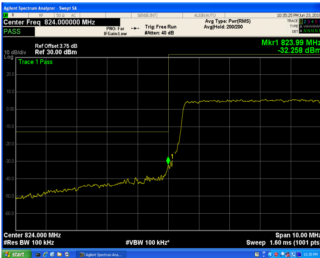
LTE Band5 QAM16 BW=10MHz Channel=20450 RB Size=25 Position=#Max
