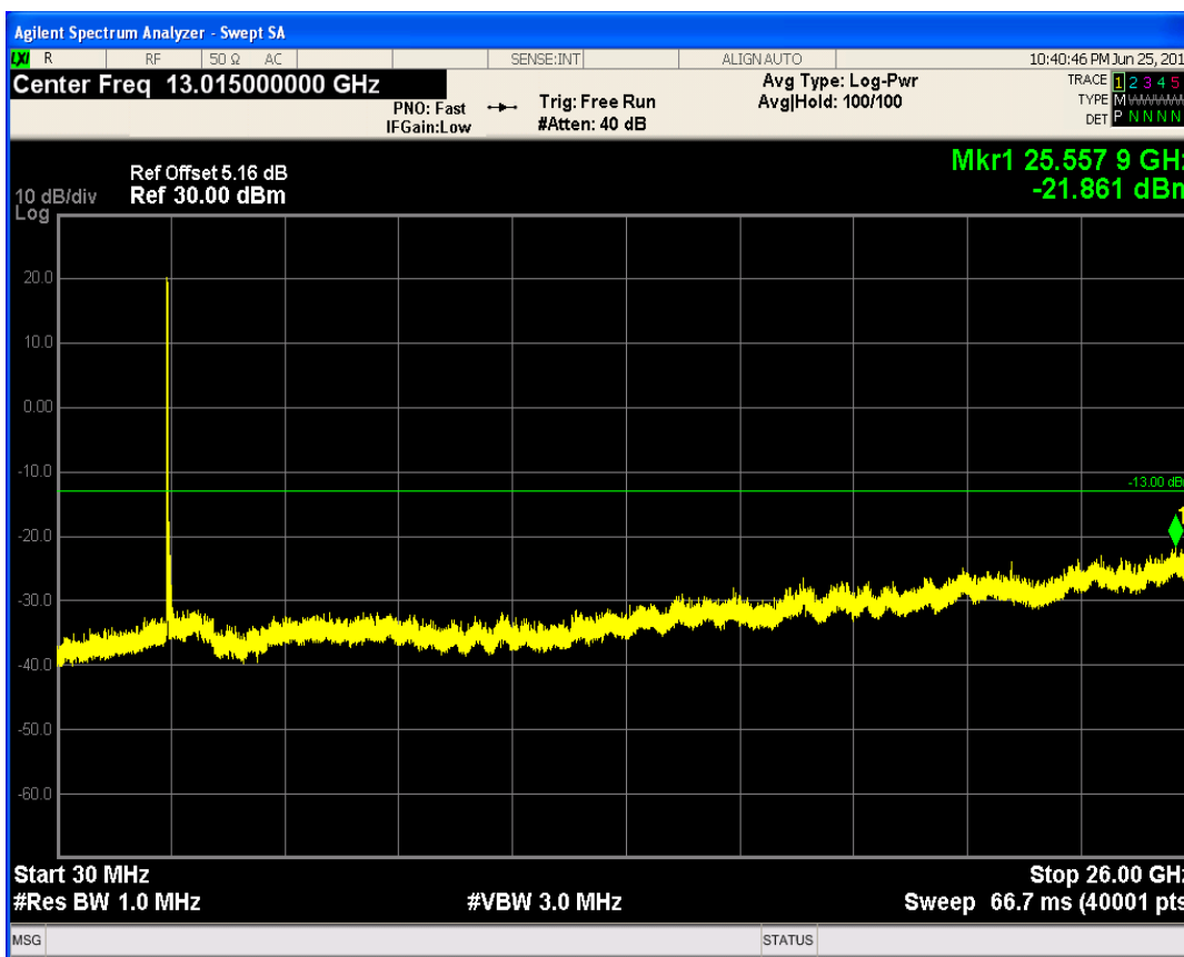
LTE Band41 QAM16 BW=20MHz Channel=41140 RB Size=100 Position=#0
