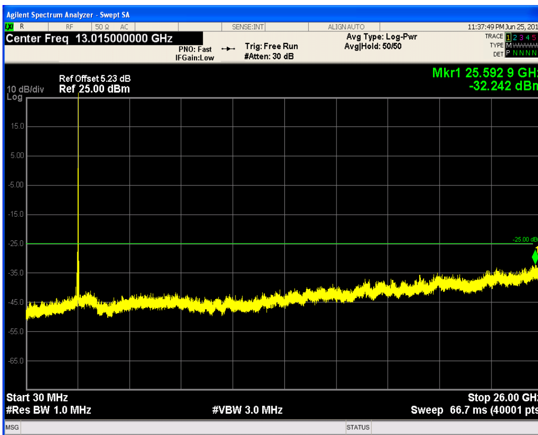
LTE Band41 QPSK BW=20MHz Channel=40140 RB Size=50 Position=#Max
