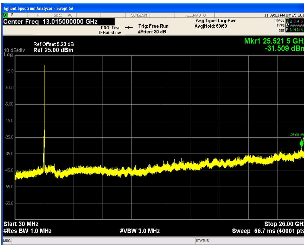
LTE Band41 QPSK BW=20MHz Channel=41140 RB Size=50 Position=#0
