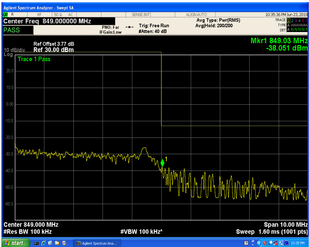
LTE Band5 QPSK BW=10MHz Channel=20600 RB Size=1 Position=#Mid
