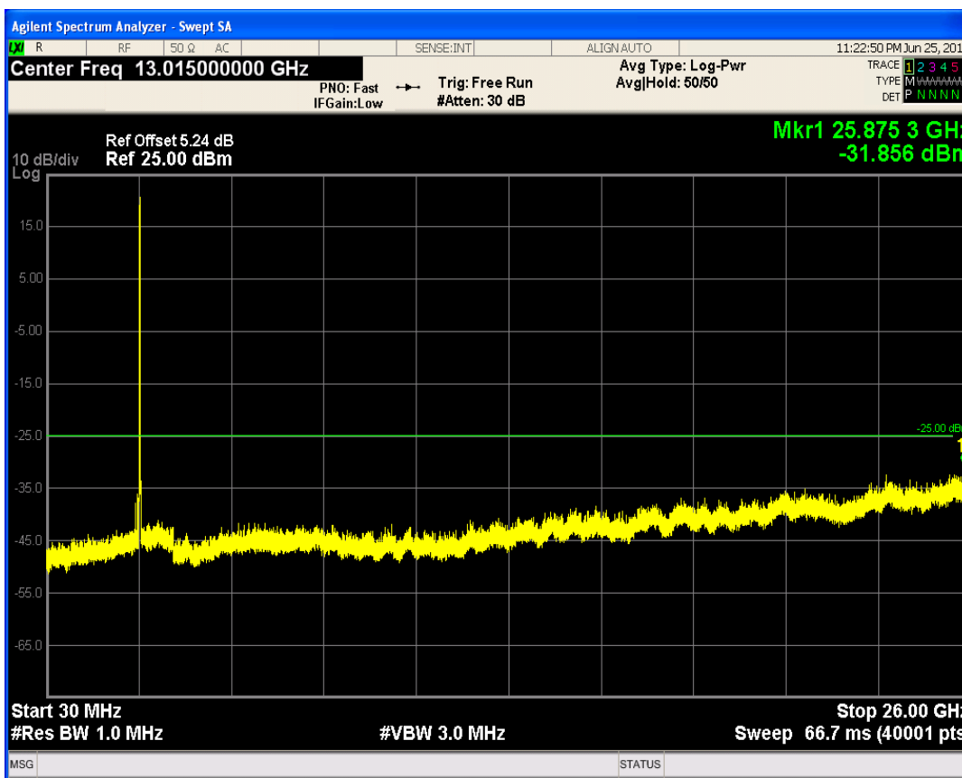
LTE Band41 QPSK BW=10MHz Channel=40090 RB Size=25 Position=#0
