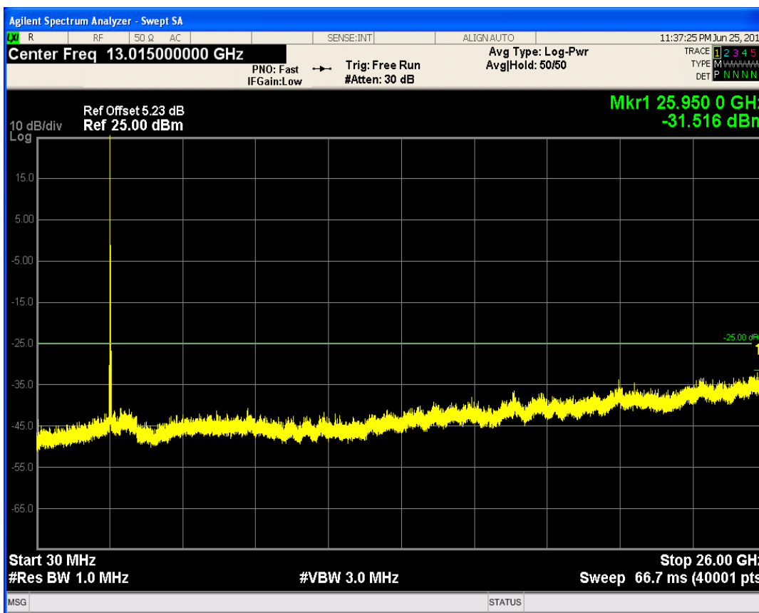
LTE Band41 QPSK BW=20MHz Channel=41140 RB Size=1 Position=#Max
