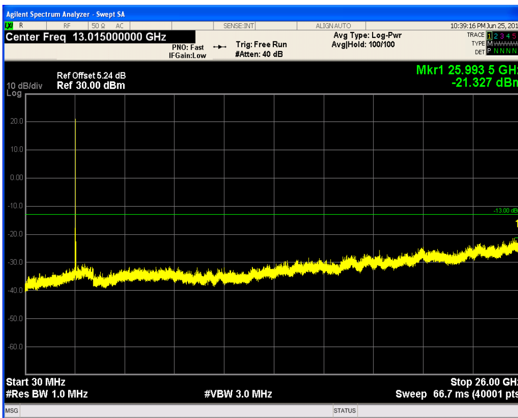
LTE Band41 QPSK BW=20MHz Channel=40140 RB Size=100 Position=#0
