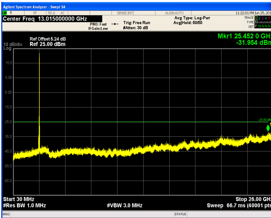
LTE Band41 QPSK BW=15MHz Channel=40115 RB Size=1 Position=#0
