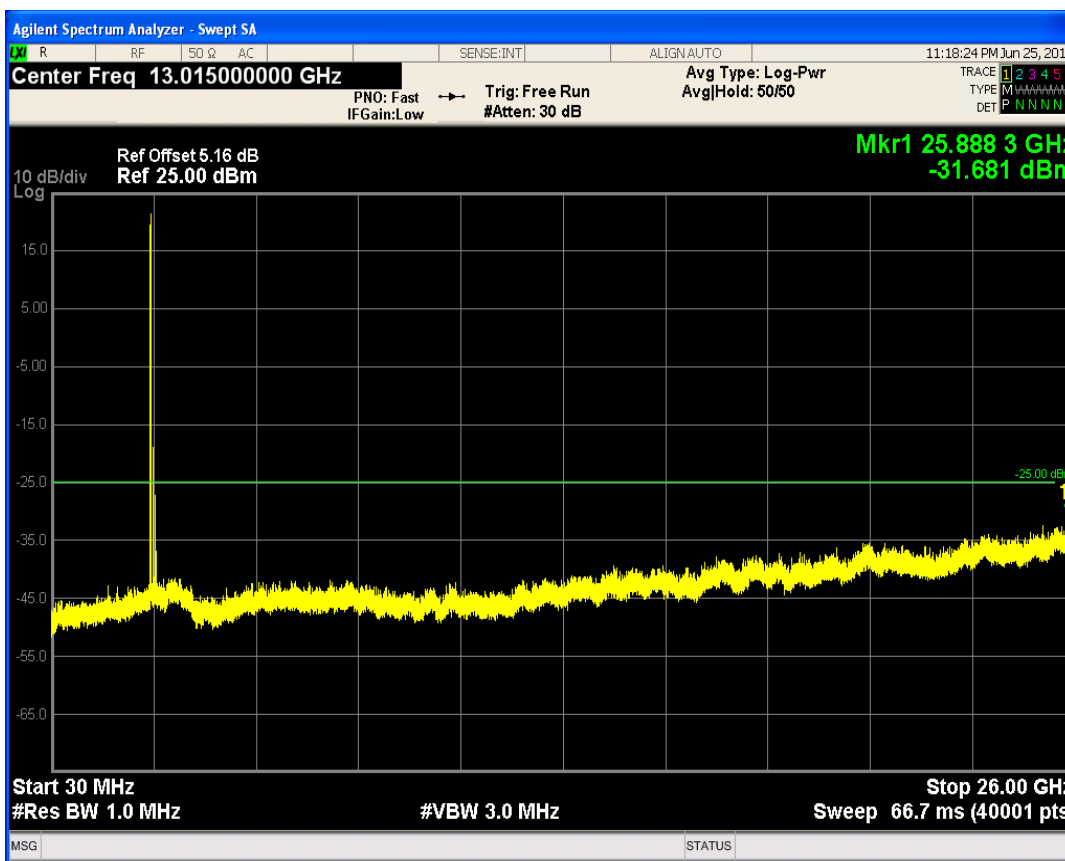
LTE Band41 QPSK BW=10MHz Channel=40090 RB Size=50 Position=#0
