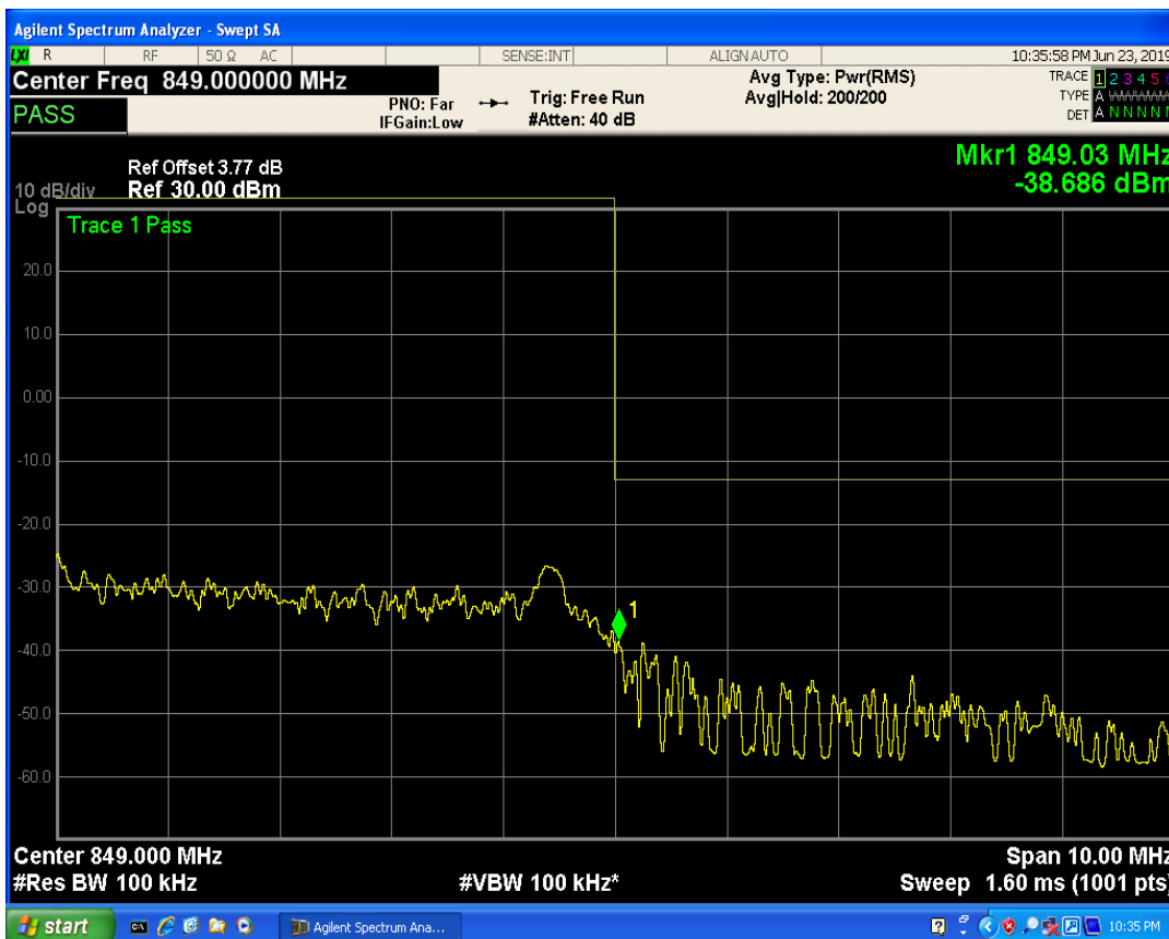
LTE Band5 QAM16 BW=10MHz Channel=20600 RB Size=1 Position=#Mid
