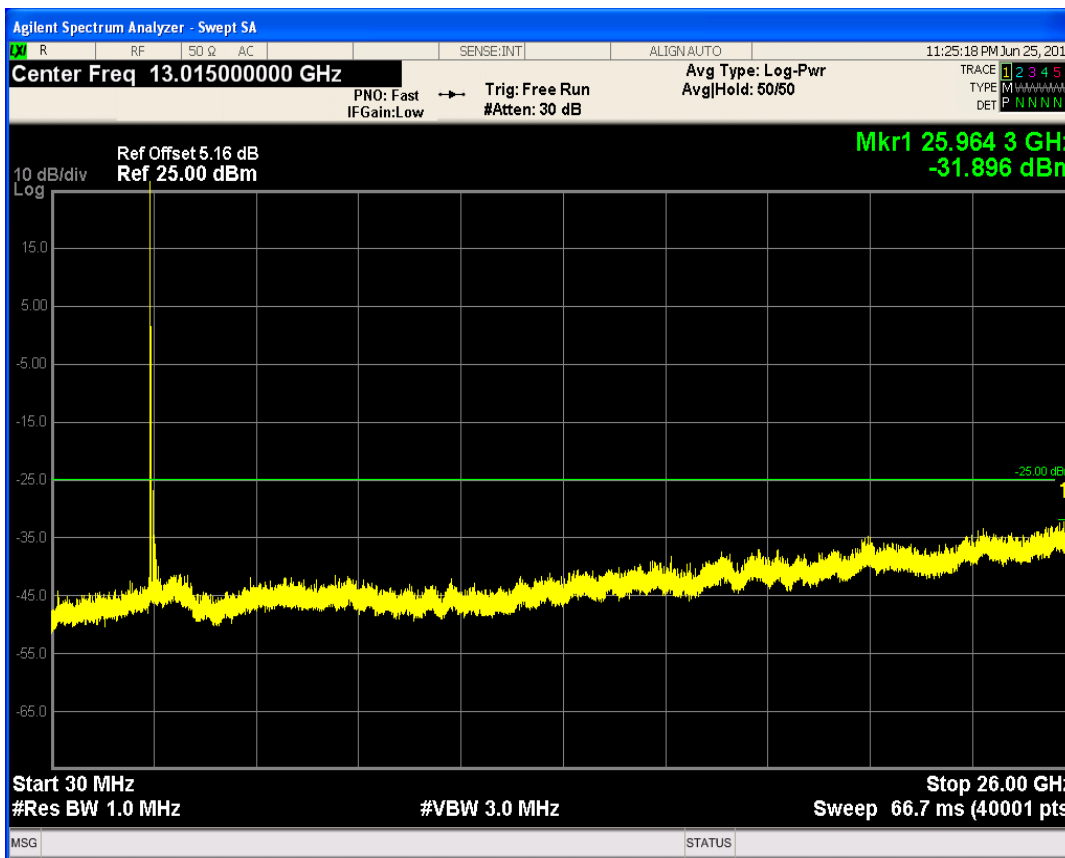
LTE Band41 QPSK BW=15MHz Channel=40115 RB Size=1 Position=#Max
