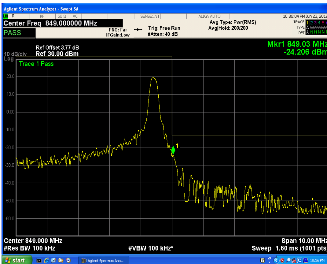
LTE Band5 QAM16 BW=10MHz Channel=20600 RB Size=25 Position=#Max
