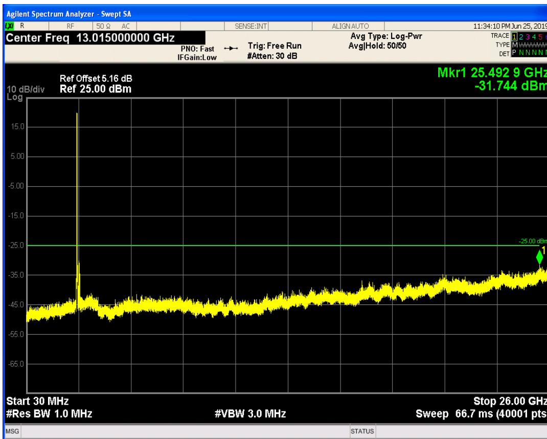
LTE Band41 QPSK BW=5MHz Channel=40065 RB Size=1 Position=#0
