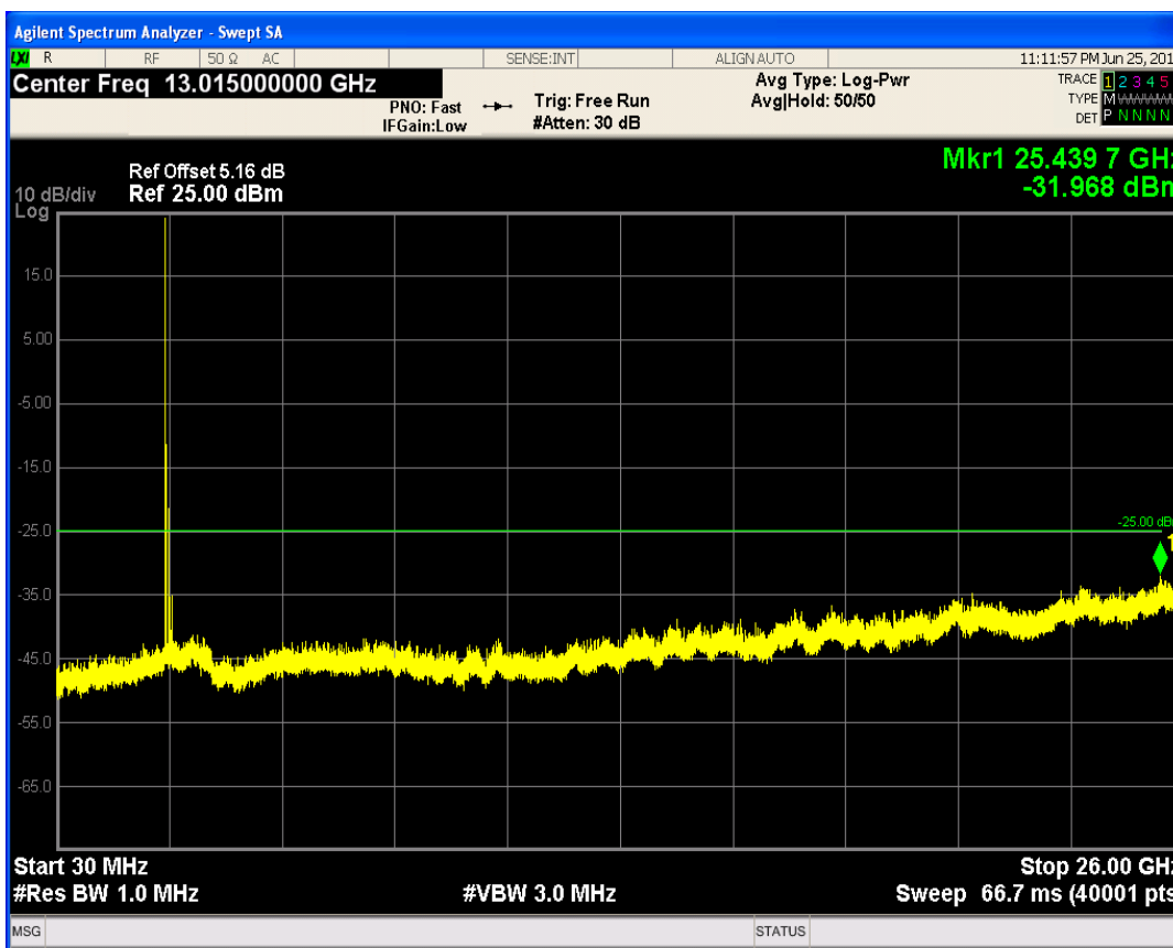
LTE Band41 QAM16 BW=5MHz Channel=40065 RB Size=1 Position=#0
