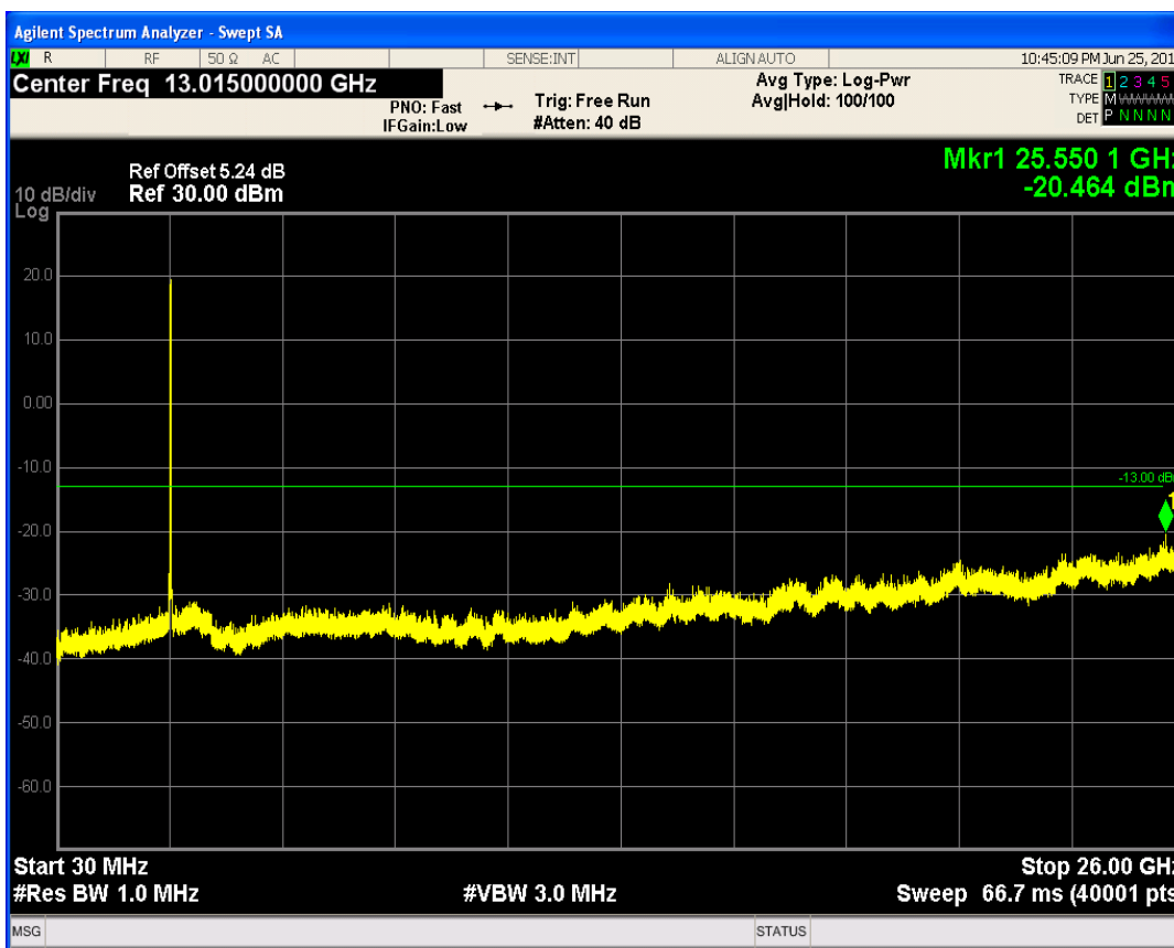
LTE Band41 QPSK BW=5MHz Channel=41215 RB Size=25 Position=#0
