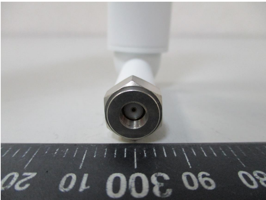
Antenna 2
