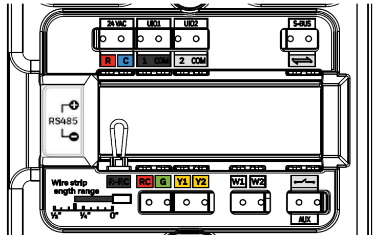
Fig. 1. Terminals
