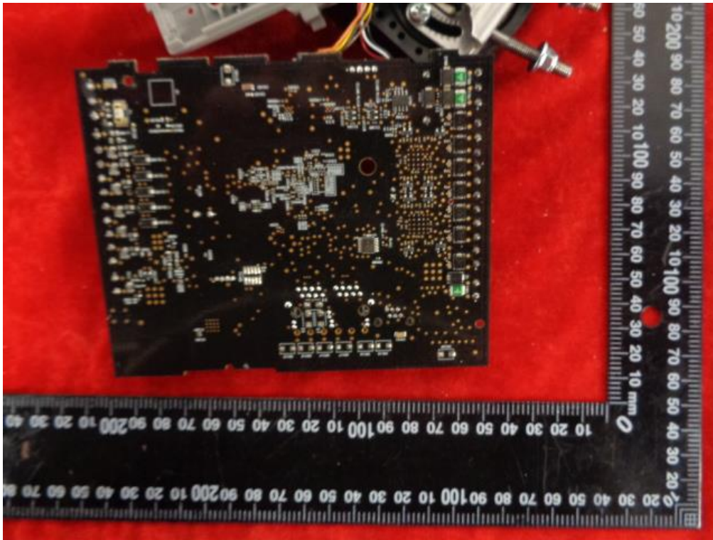
PCB view of VAVi-7u5-IP-BLE
