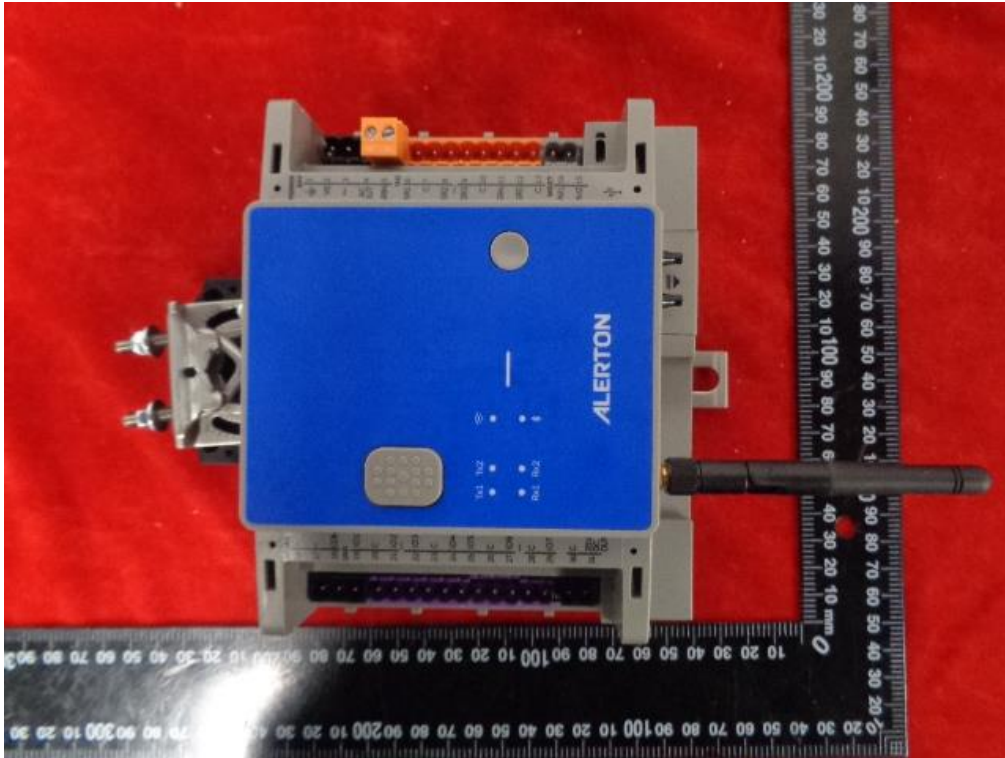
Front view of VAVi-7u5-IP-BLE
