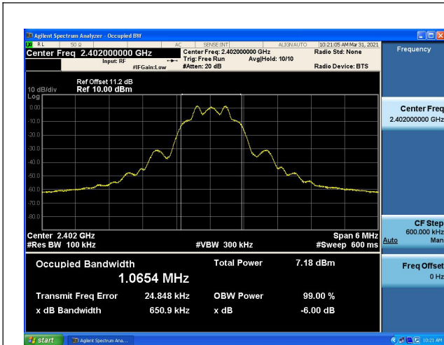
Modulation: Coded S=8 2402MHz
