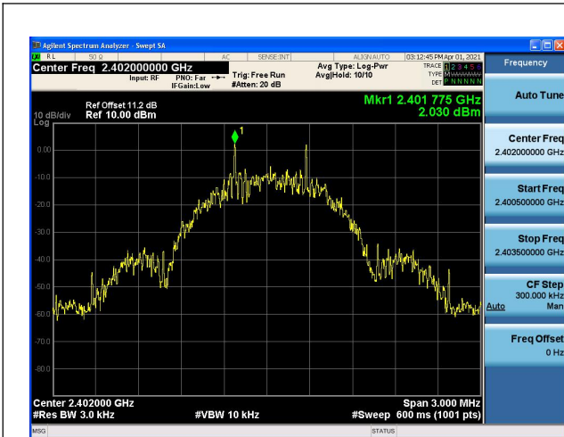
Modulation: Coded S=2 2402MHz
