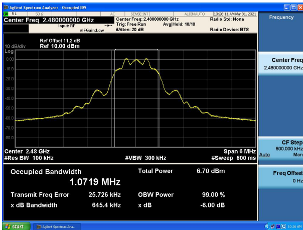
Modulation: Coded S=8 2480MHz
