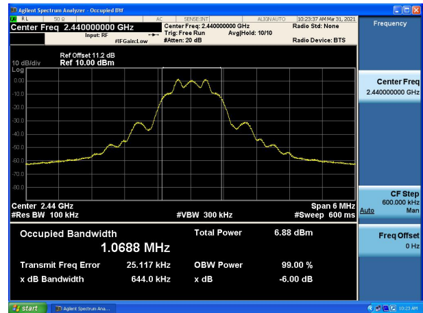
Modulation: Coded S=8 2440MHz
