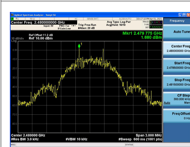
Modulation: Coded S=2 2480MHz
