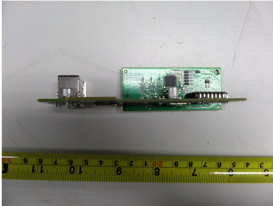
Pic 7. LED board & USB board
