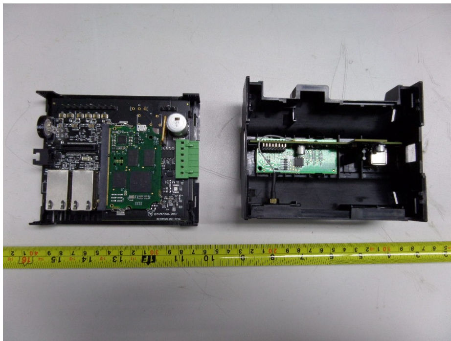
Pic 2. Internal of view
