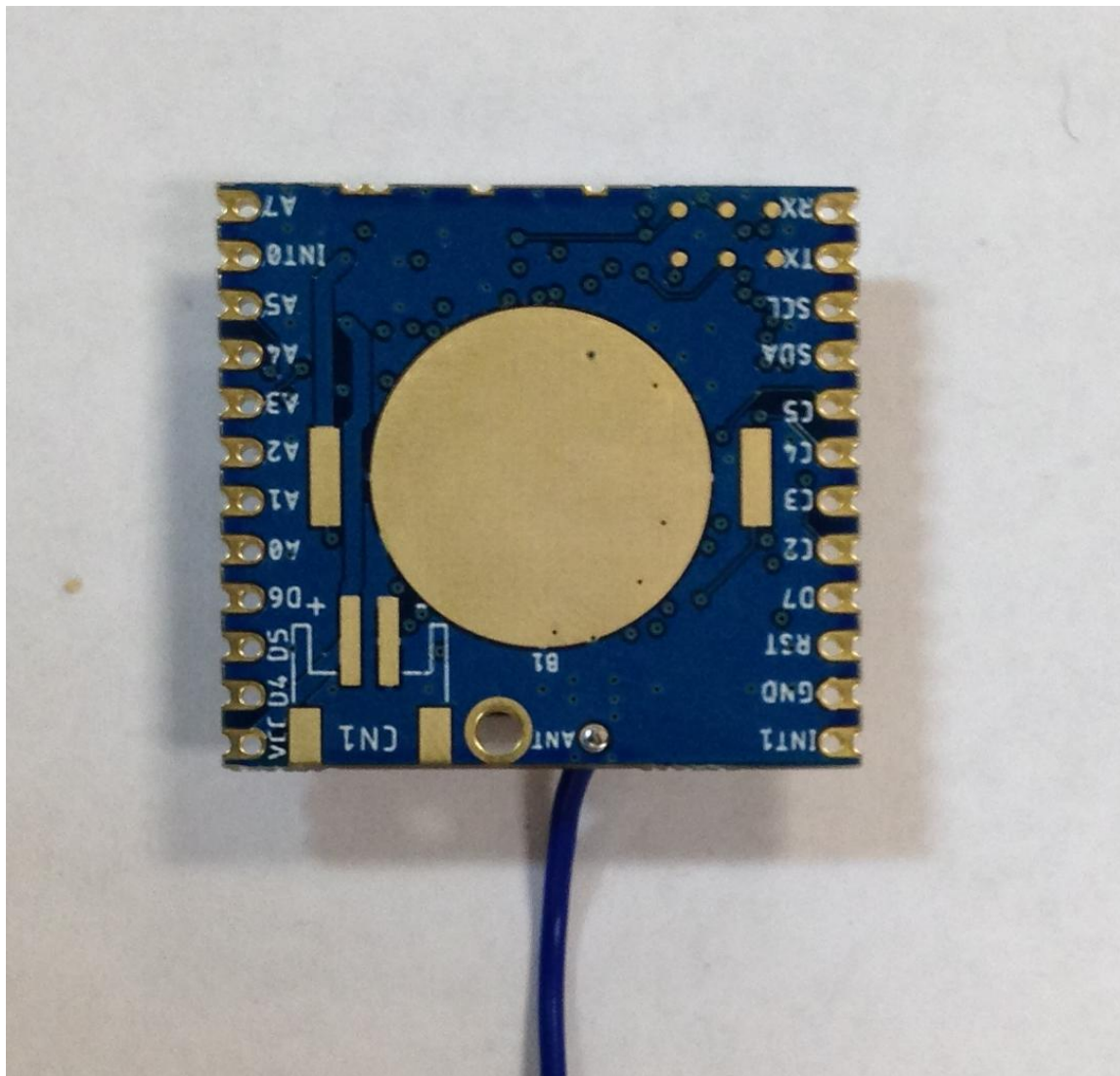
Figure 2. Module, Bottom
