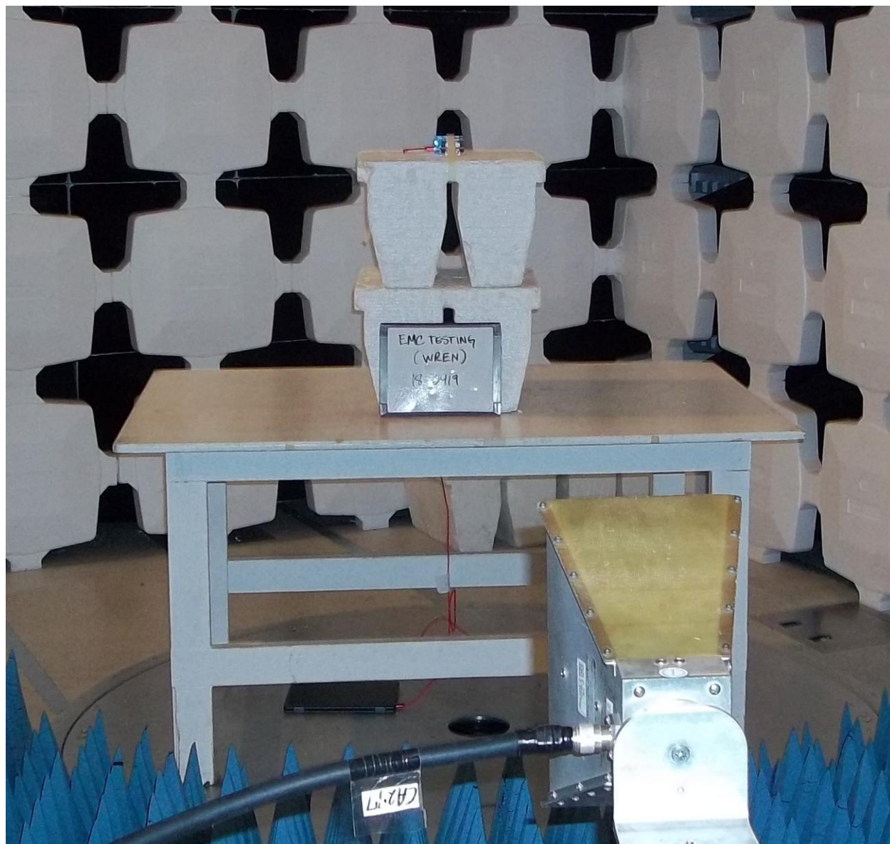
Figure 6. Radiated Emissions Test Configuration (Above 6 GHz)
