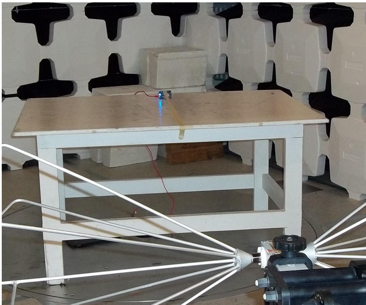
Figure 1. Radiated Emissions Test Configuration (Front)
