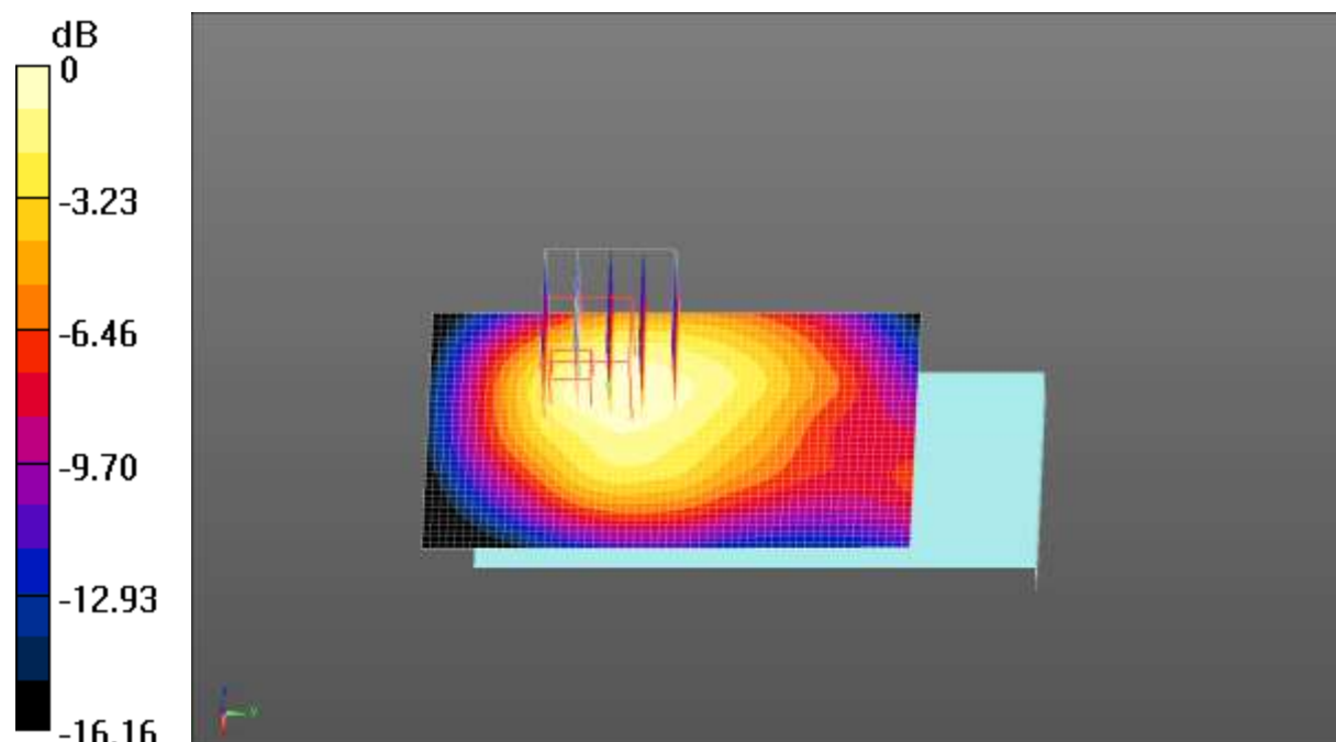
0 dB = 1.38 W/kg = 1.40 dBW/kg
