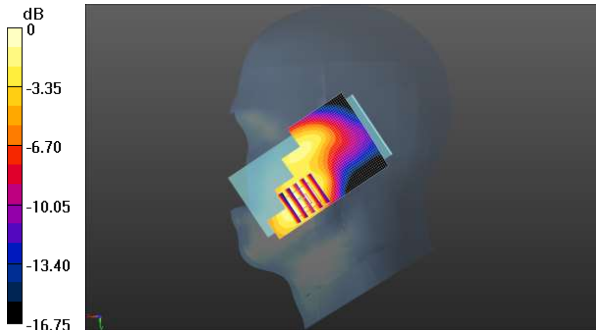
0 dB = 0.516 W/kg = -2.87 dBW/kg
