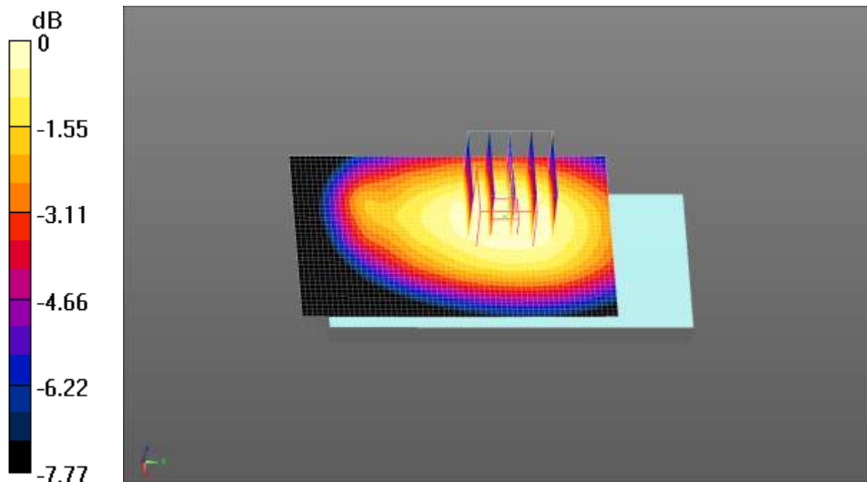
0 dB = 0.540 W/kg = -2.68 dBW/kg
