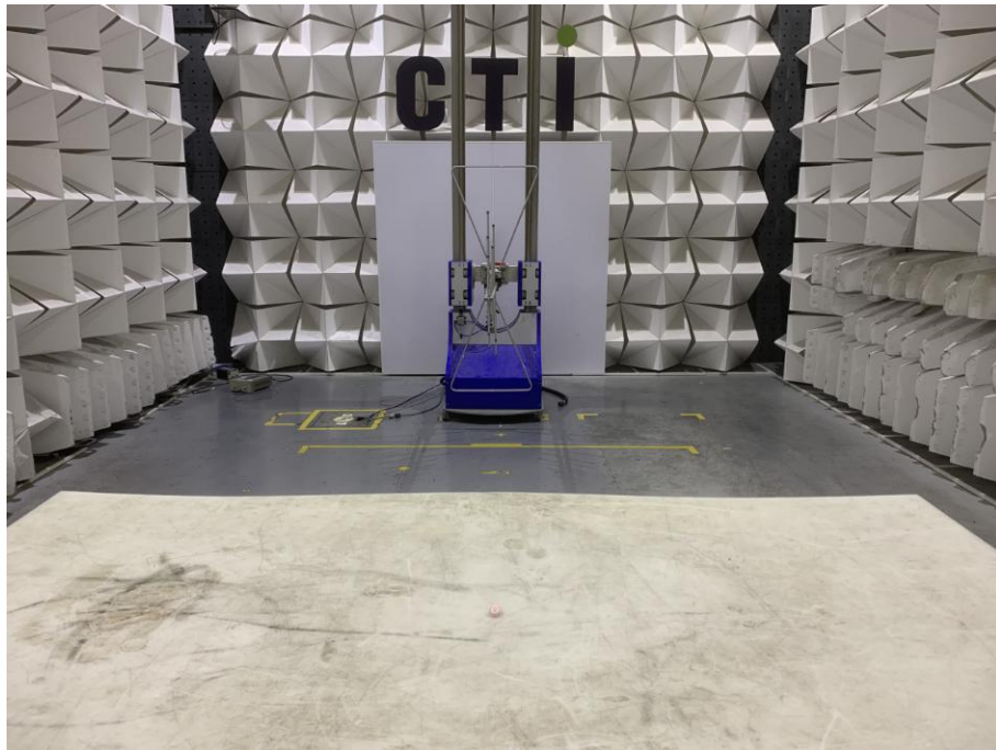
Radiated spurious emission Test Setup-1(Below 1GHz) Ear R
