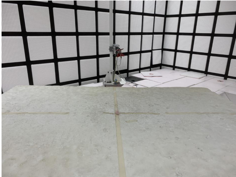
Radiated spurious emission Test Setup-2(Above 1GHz) Ear L
