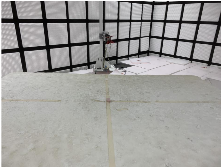
Radiated spurious emission Test Setup-2(Above 1GHz) Ear R
