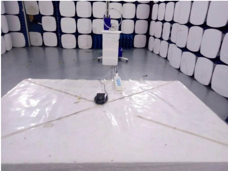
Radiated emission
