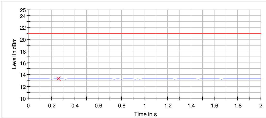
Peak Power
