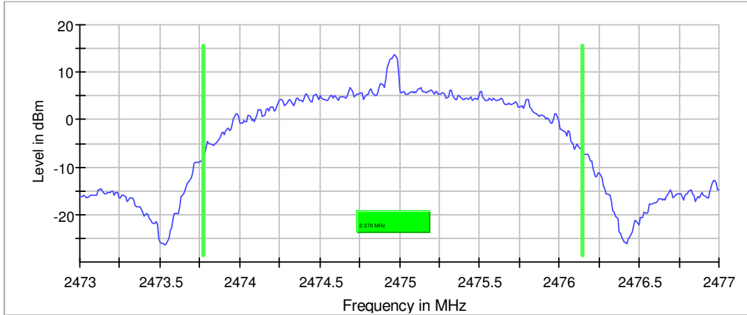
20 dB Bandwidth
