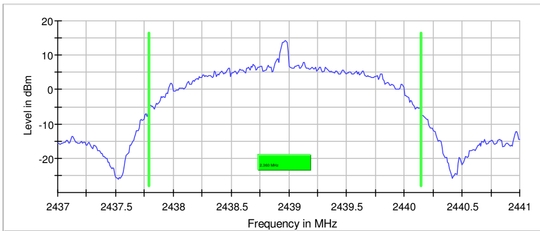
20 dB Bandwidth
