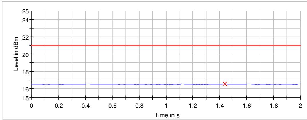
Peak Power
