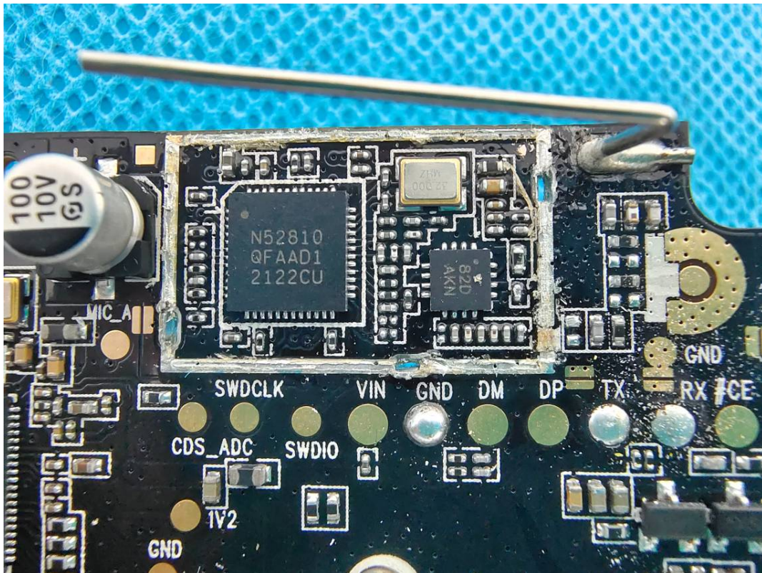
FHSS ANT
