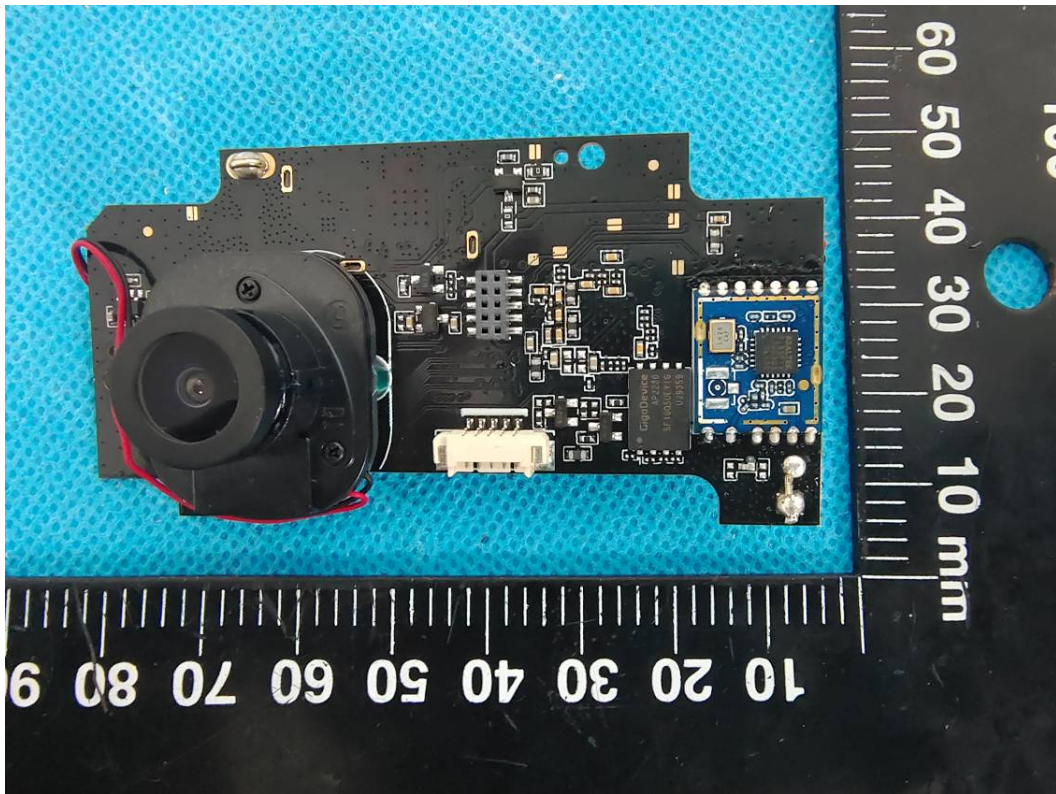
SRD Antenna
