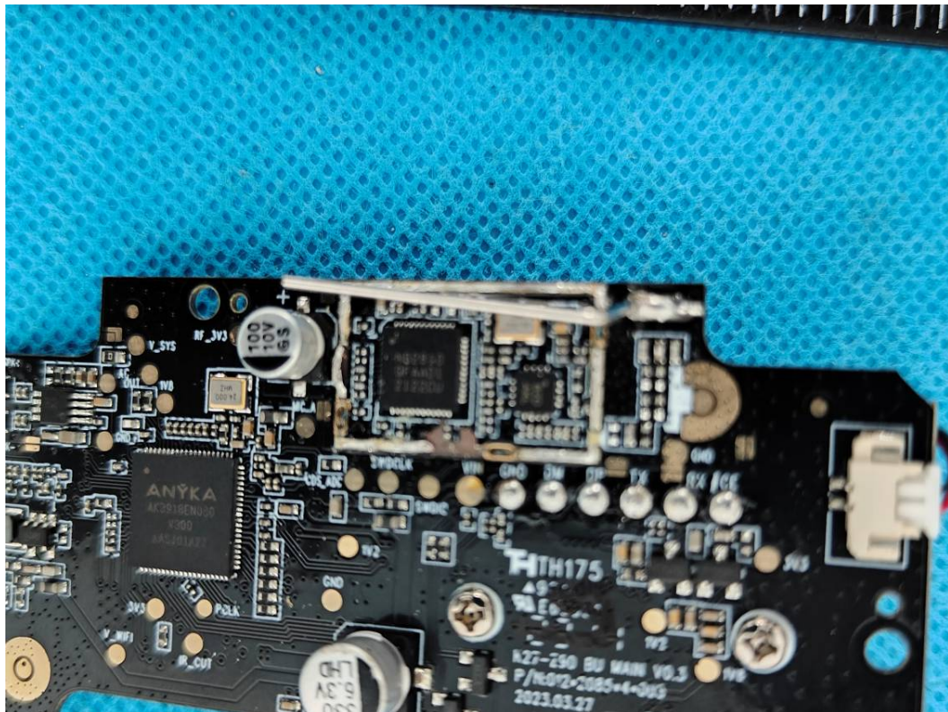
SRD Antenna
