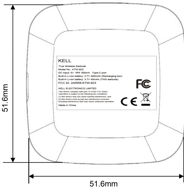
Charging box
