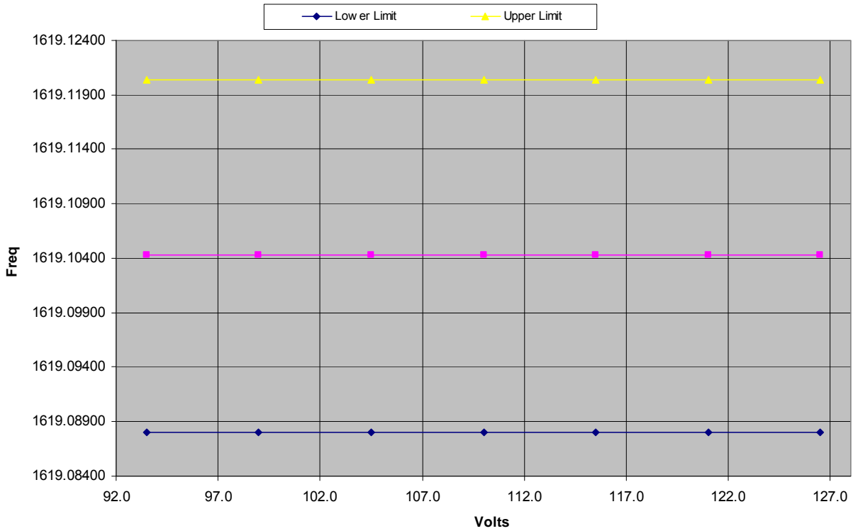
Channel 75 Frequency Stability - Voltage
