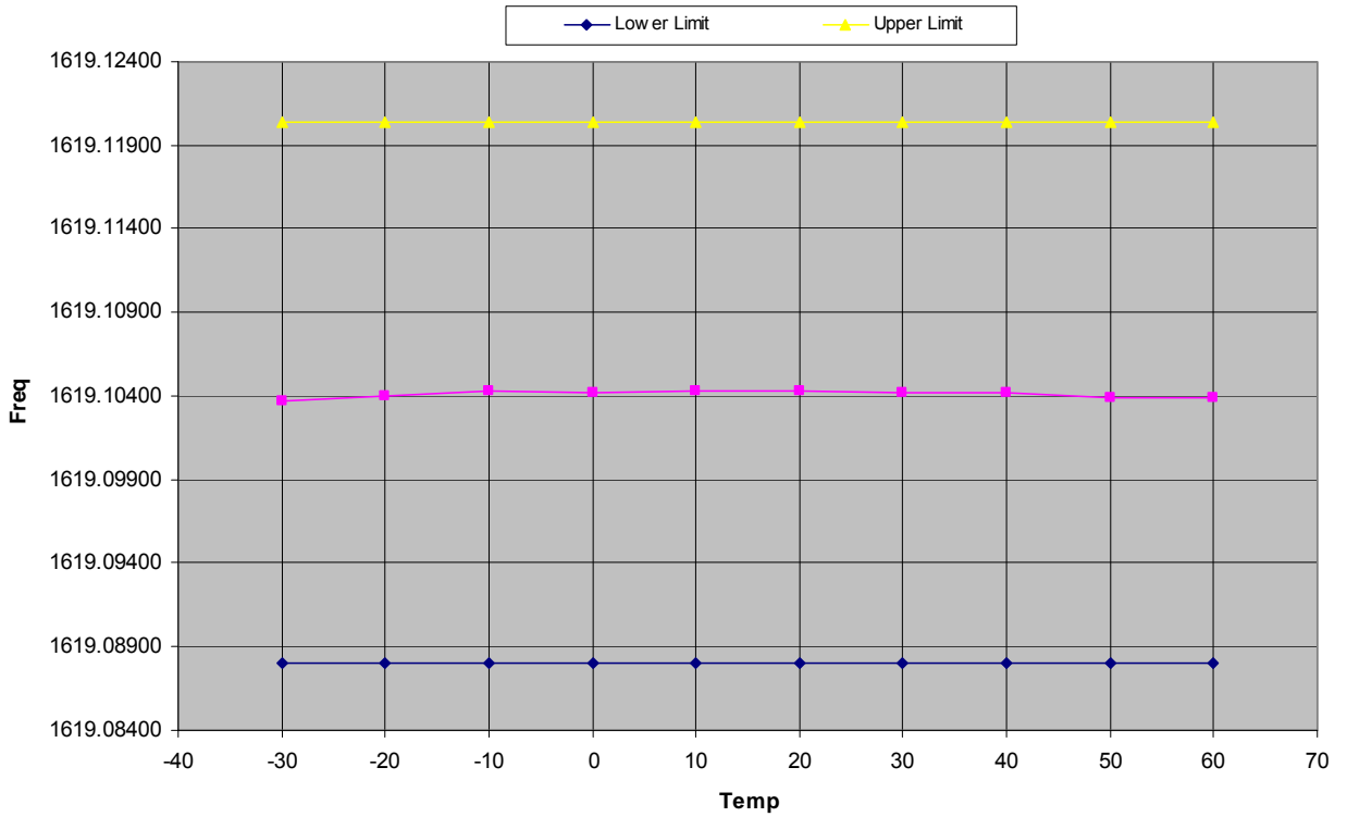
Channel 75 Frequency Stability - Temperature
