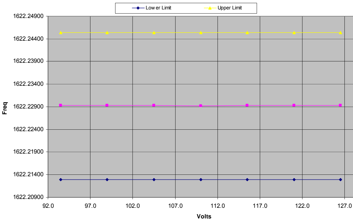
Channel 150 Frequency Stability - Voltage
