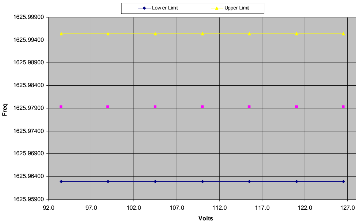
Channel 240 Frequency Stability - Voltage
