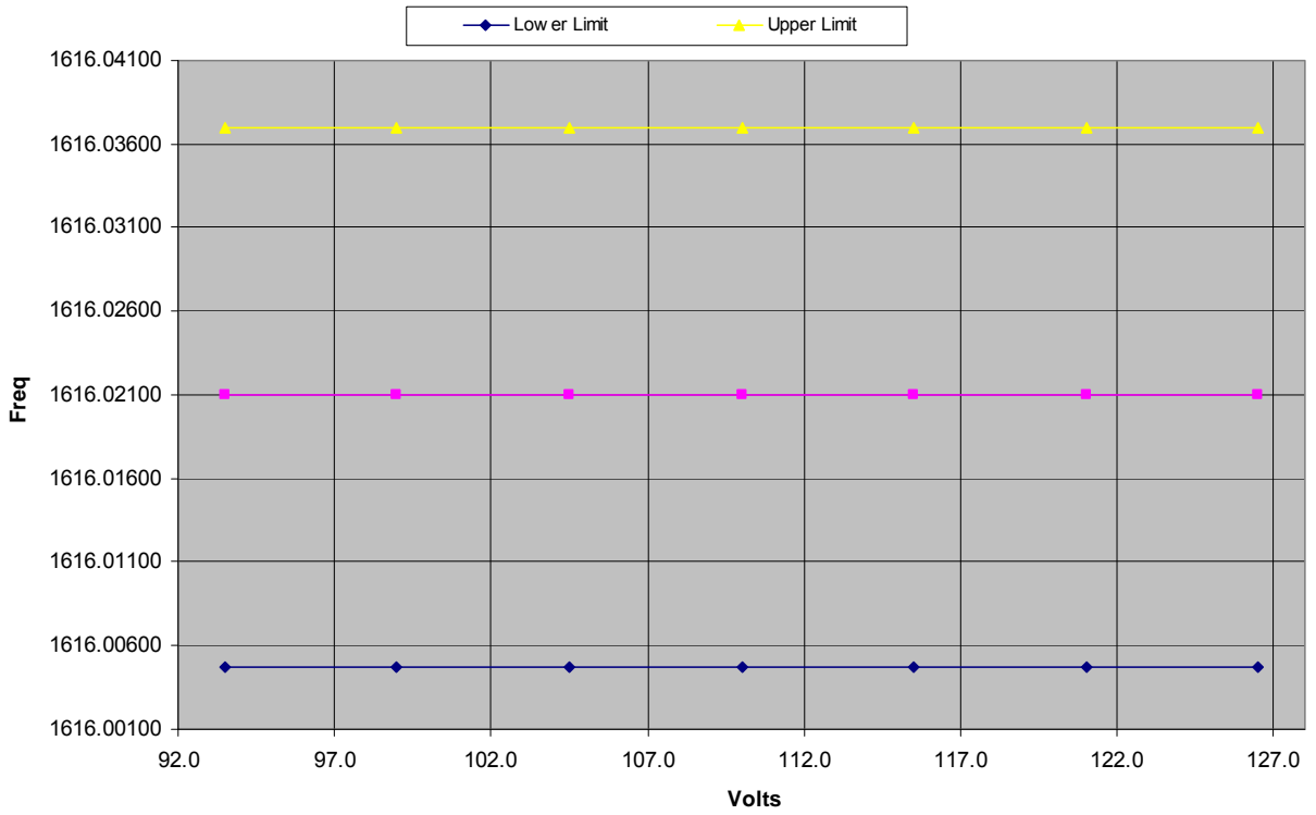
Channel 1 Frequency Stability - Voltage
