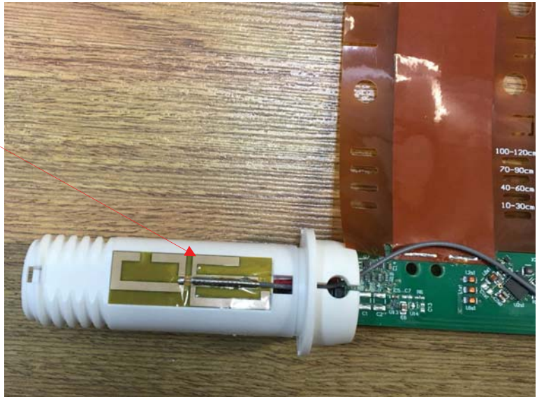
BT Antenna
