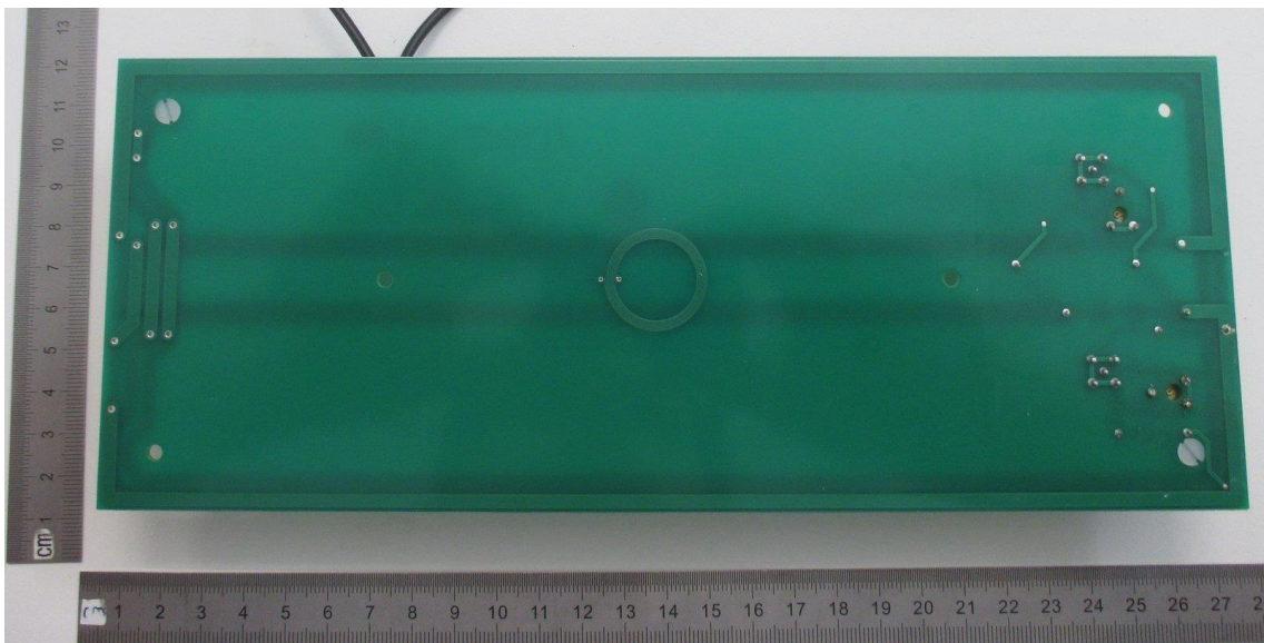
Figure 17 - PCB antenna, top side
