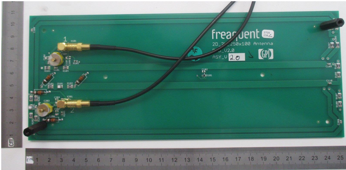
Figure 16 - PCB antenna, bottom side
