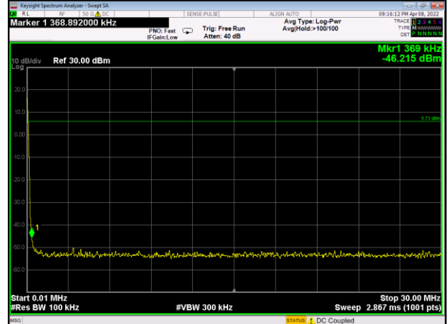
ASK on channel 01
