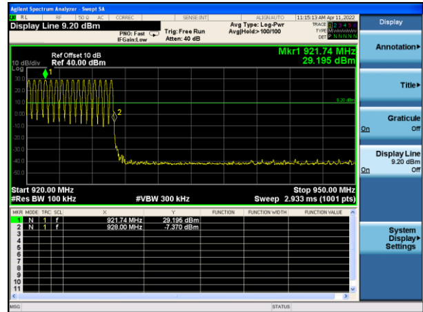
ASK: Band Edge-High Channel (Hopping Mode)
