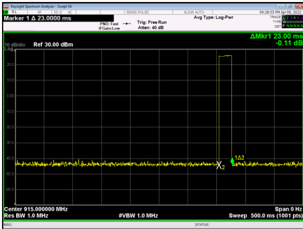
Package Transfer Time Plot 915MHz
