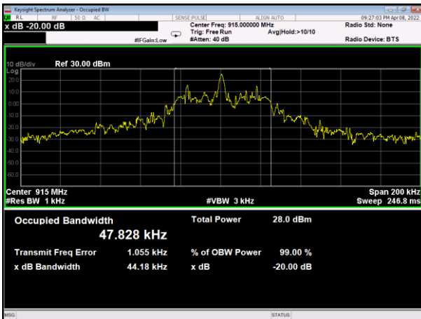
20dB Bandwidth plot on channel 26 (1Mbps)
