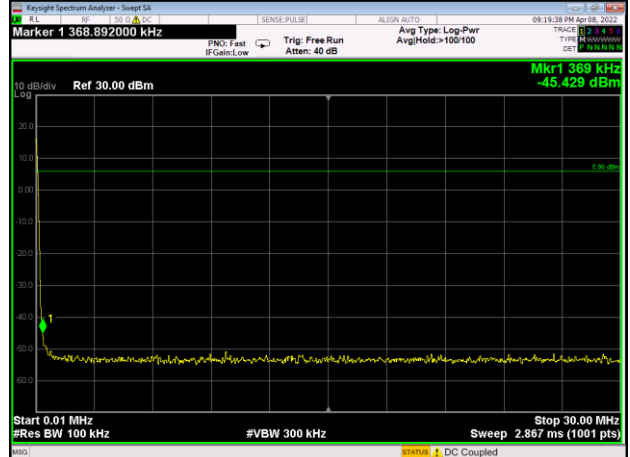
ASK on channel 26
