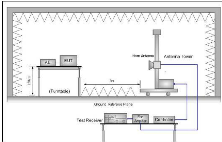
Above 1GHz Test Setup
