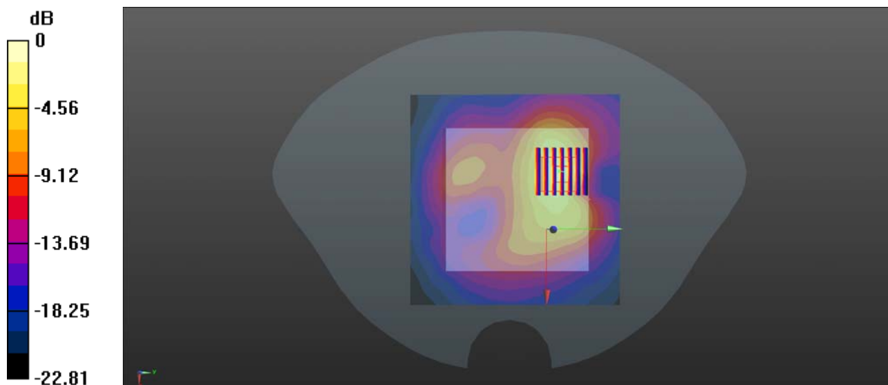
0 dB = 0.446 W/kg
