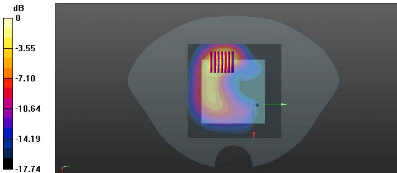
0 dB = 0.723 W/kg
