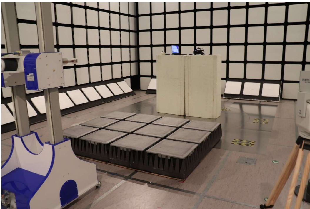
Photograph 6. Radiated emission test setup (18 GHz – 26.5 GHz)
