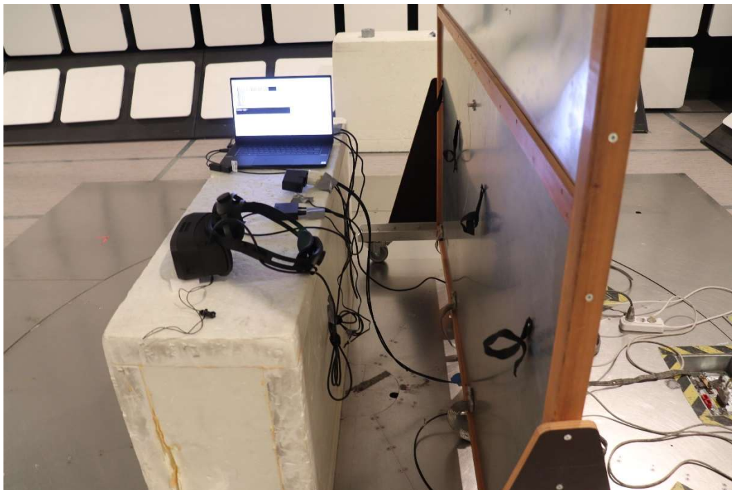
Photograph 7. Conducted emission test setup
