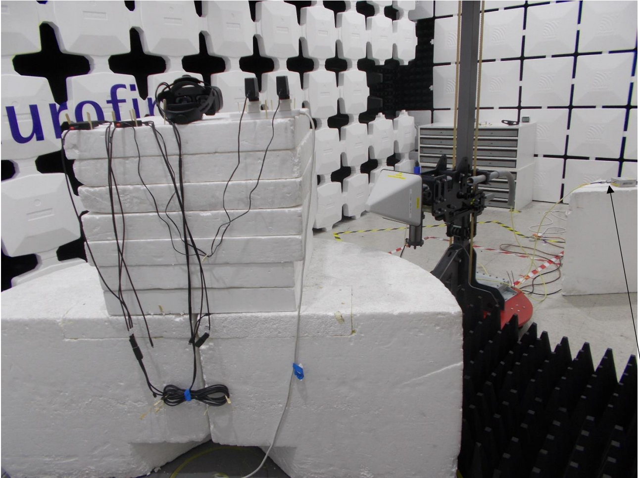
Radiated emissions 1-18GHz showing 2.4GHz notch filter at the input to the pre-amplifier
