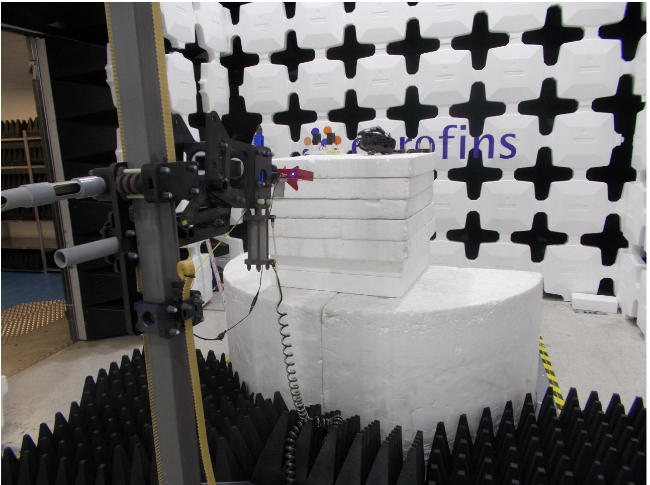
Radiated emissions 18-26GHz
