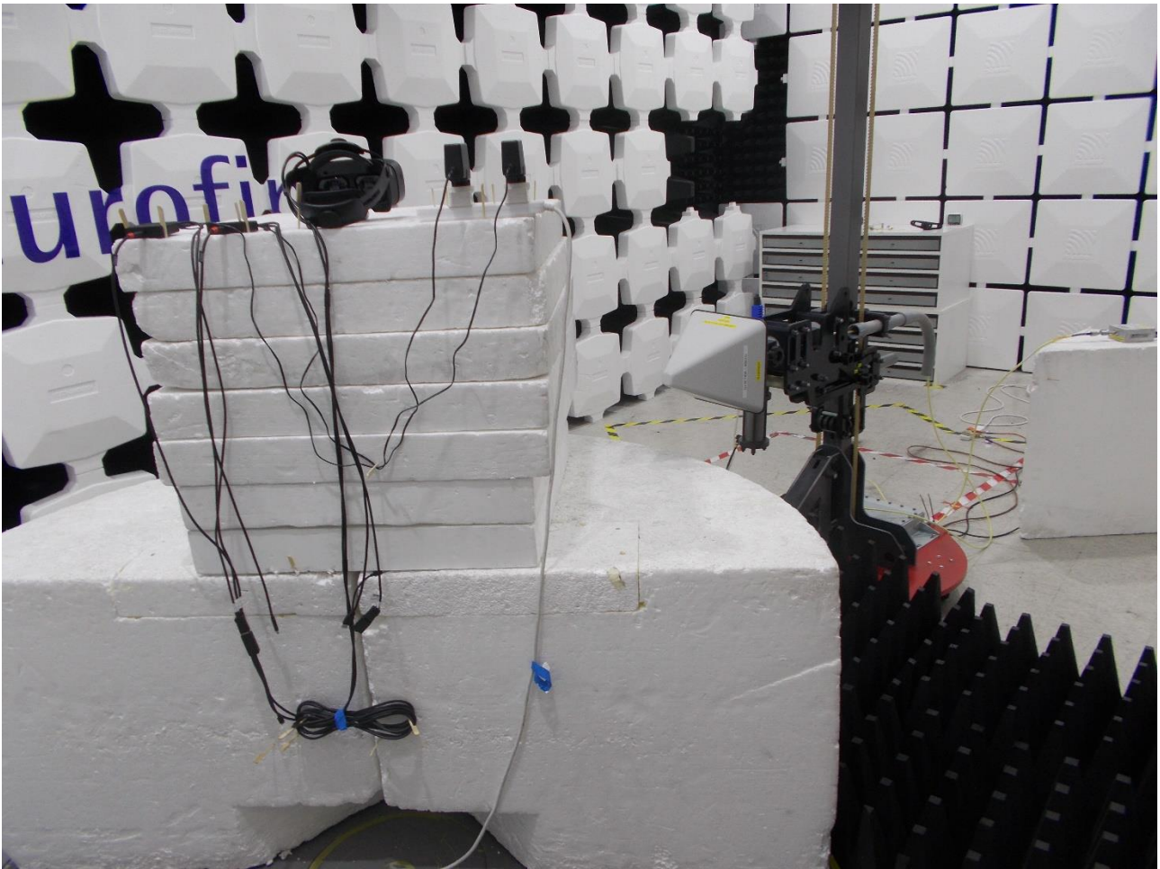
Radiated emissions 1-18GHz – for spurious and band edge measurements
