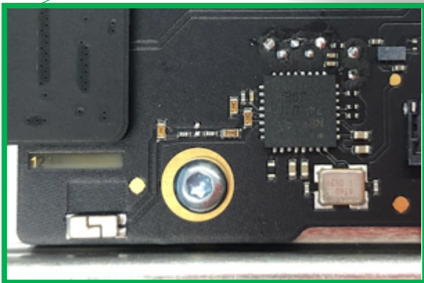
Radio circuit U2000 and antenna A2000 location
