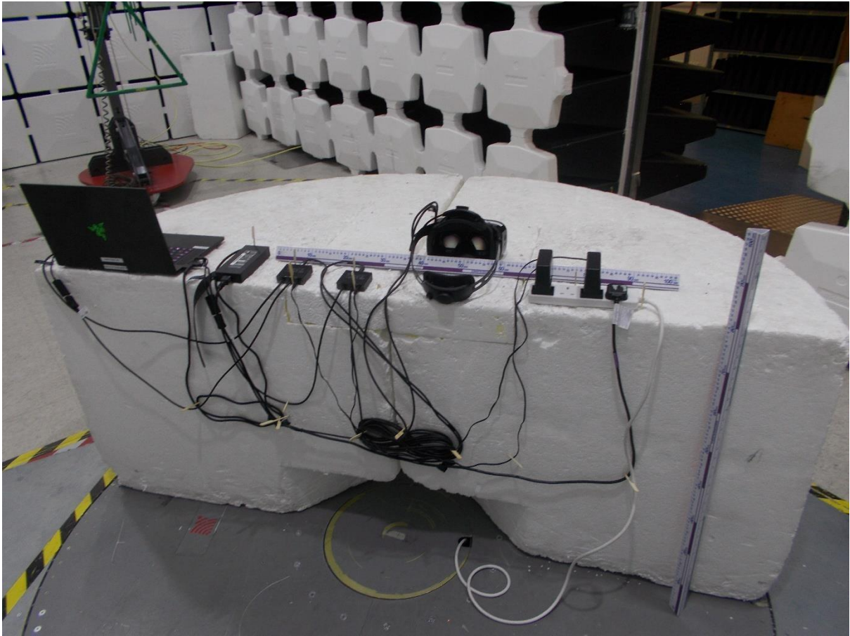
Radiated electric field emissions 30MHz to 1GHz
