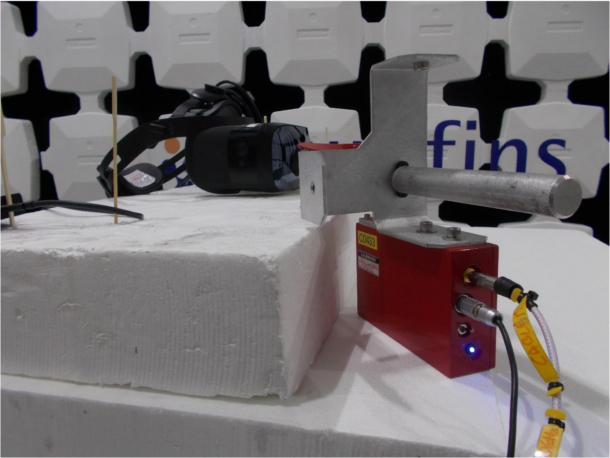
Radiated emissions manual investigation 18-26GHz
