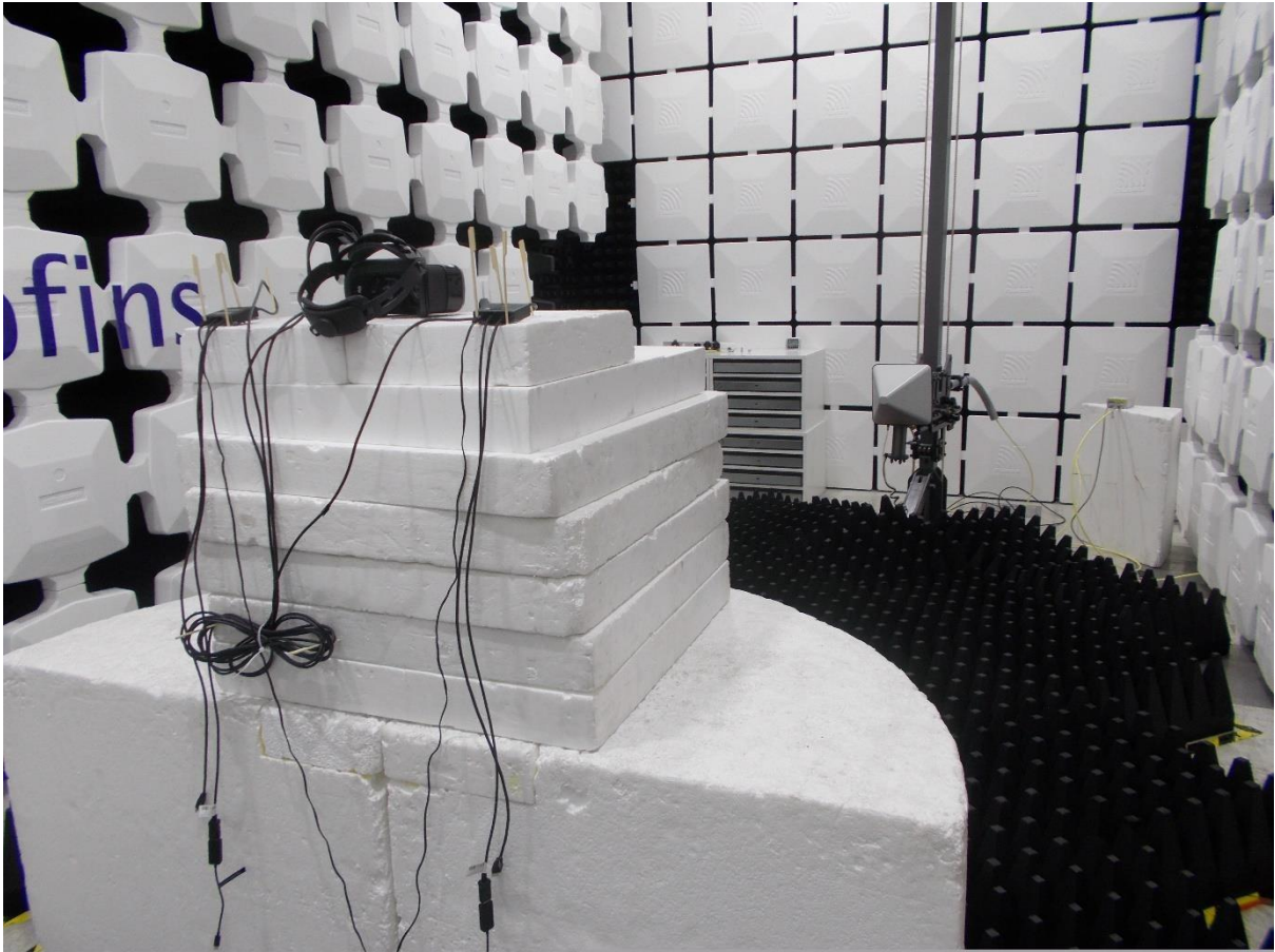
Radiated emissions 1-18GHz – radiated spurious for restricted bands and band edge measurements
